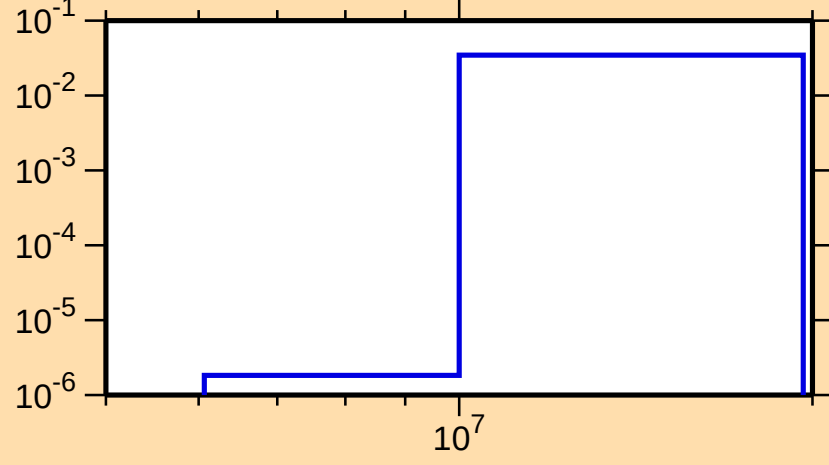
\sigma vs. E for ^{13}\text{N}(n,p\alpha)
