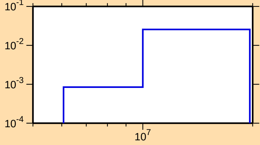
\sigma vs. E for ^{13}\text{N}(\text{n,ncont.})
