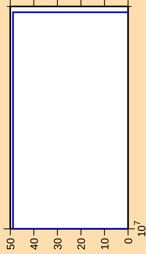
\Delta\sigma/\sigma vs. E for ^{13}\text{N}(\text{n,pd})
