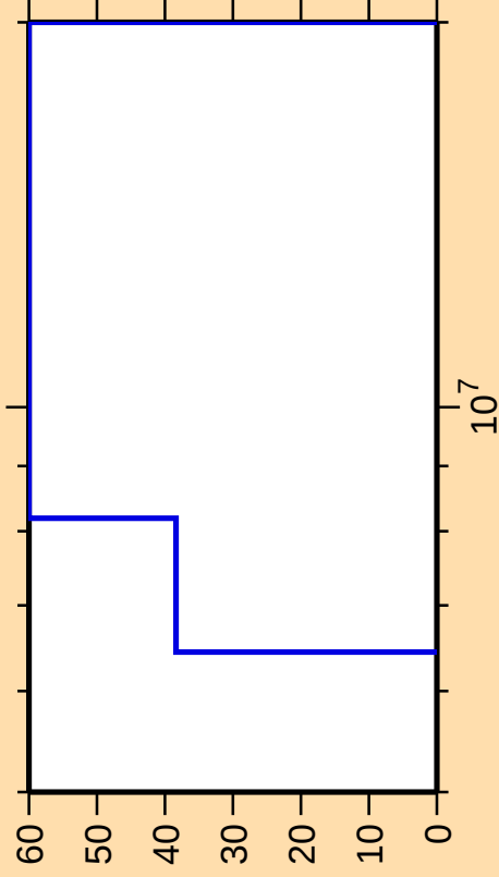
\Delta\sigma/\sigma vs. E for ^{13}\text{N}(n,\alpha)
