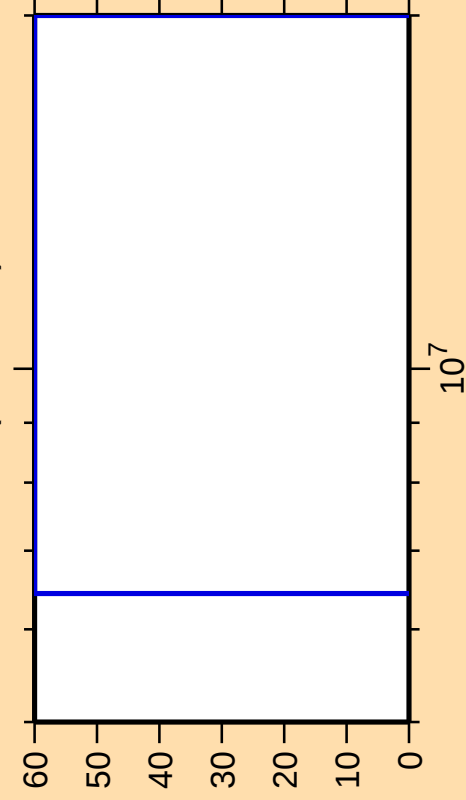
\Delta\sigma/\sigma vs. E for ^{13}\text{N}(\text{n,ncont.})
