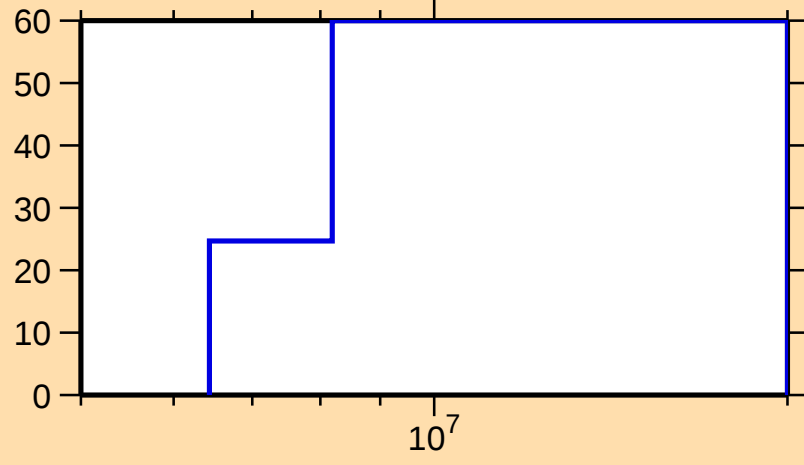
\Delta\sigma/\sigma vs. E for ^{13}\text{N}(\text{n},\text{inel.})
