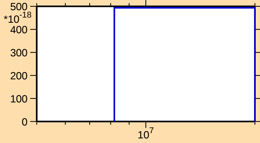
\sigma vs. E for ^{13}\text{N}(\text{n},\text{nd})
