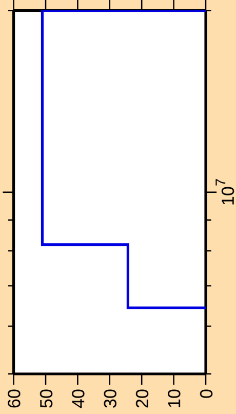
\Delta\sigma/\sigma vs. E for ^{13}\text{N}(n,n_4)
