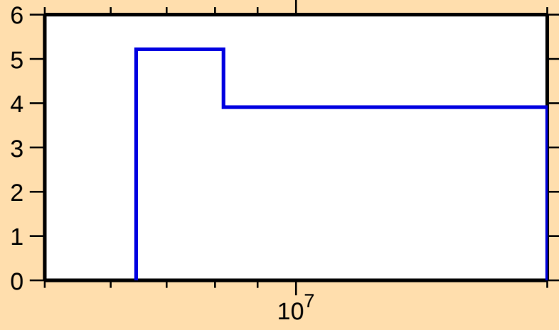
\Delta\sigma/\sigma vs. E for ^{13}\text{N}(\text{n},\text{tot.})
