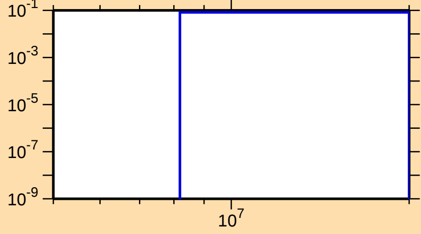
\sigma vs. E for ^{13}\text{N}(\text{mt117})
