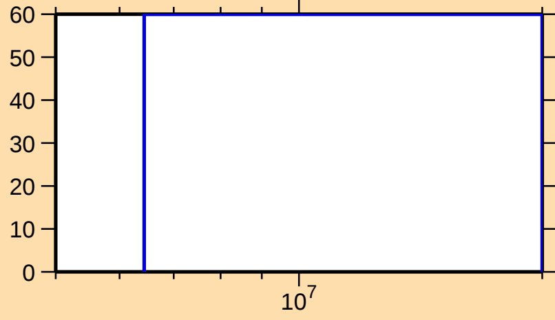
\Delta\sigma/\sigma vs. E for ^{13}\text{N}(n,\text{ncont.})
