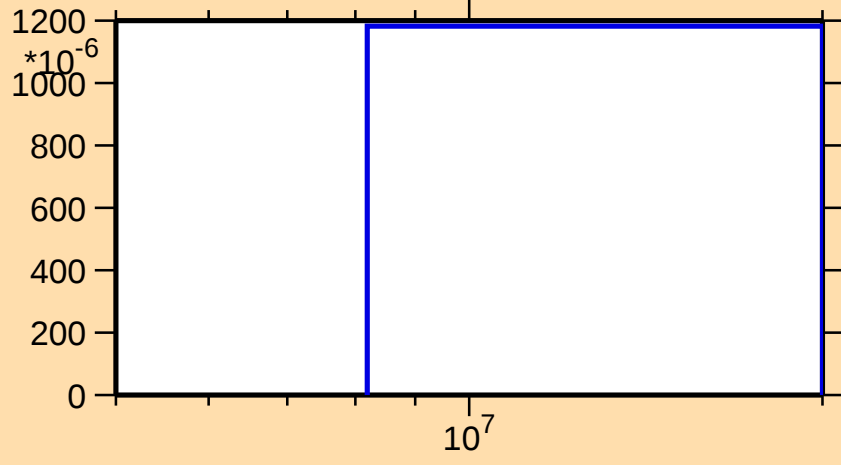
\sigma vs. E for ^{13}\text{N}(\text{mt } 45)
