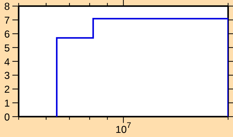
\Delta\sigma/\sigma vs. E for ^{13}\text{N}(\text{n},\text{nonel.})
