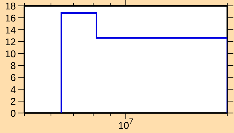
\Delta\sigma/\sigma vs. E for ^{13}\text{N}(\text{n},\text{el.})
