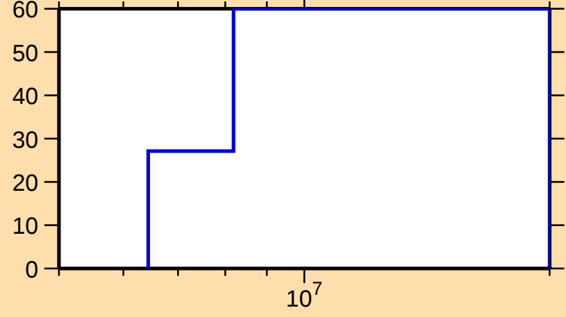
\Delta\sigma/\sigma vs. E for ^{13}\text{N}(n,n_1)
