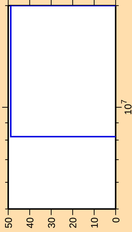
\Delta\sigma/\sigma vs. E for ^{13}\text{N}(\text{n},\text{pd})
