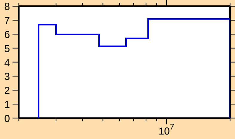
\Delta\sigma/\sigma vs. E for ^{13}\text{N}(\text{n,nonel.})
