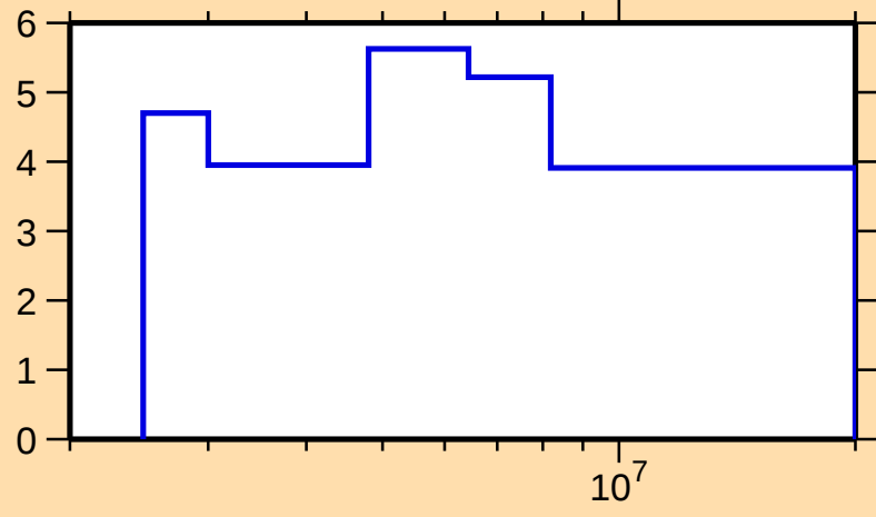
\Delta\sigma/\sigma vs. E for ^{13}\text{N}(\text{n,tot.})
