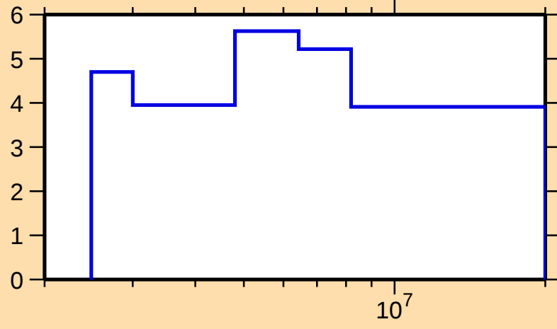
\Delta\sigma/\sigma vs. E for ^{13}\text{N}(n,\text{tot.})
