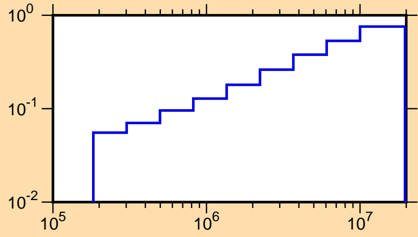
\mu vs. E for ^{17}\text{N}(\text{mt251})
