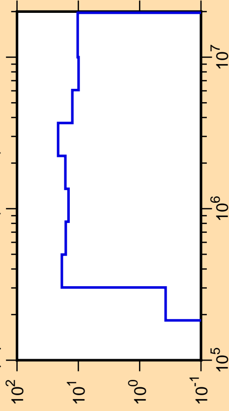
\Delta\mu/\mu vs. E for ^{17}\text{N}(\text{mt251})
