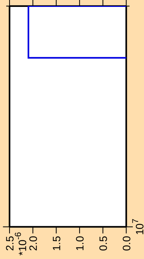
\Delta\sigma/\sigma vs. E for ^{86}\text{Nb}(n,\text{nt})
