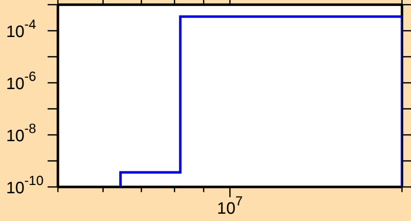
\sigma vs. E for ^{86}\text{Nb}(n,t)
