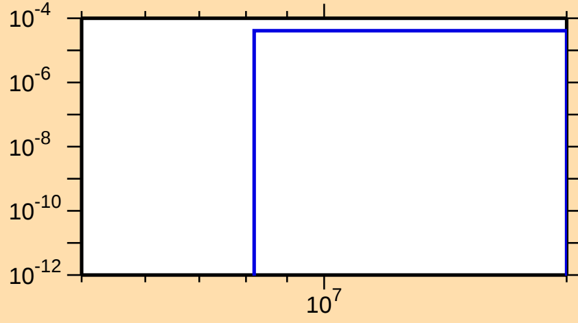
\sigma vs. E for ^{86}\text{Nb}(n,\text{pd})
