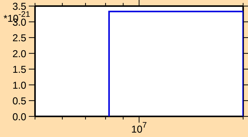
\sigma vs. E for ^{86}\text{Nb}(n,nt)
