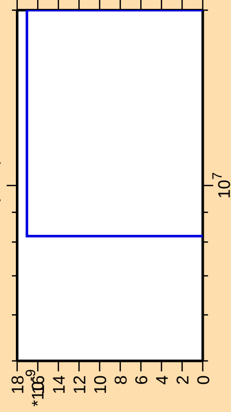
\Delta\sigma/\sigma vs. E for ^{86}\text{Nb}(n,nt)
