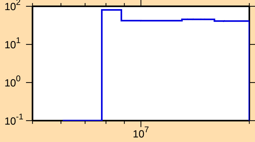
\Delta\sigma/\sigma vs. E for ^{103}\text{Nb}(n,p)
