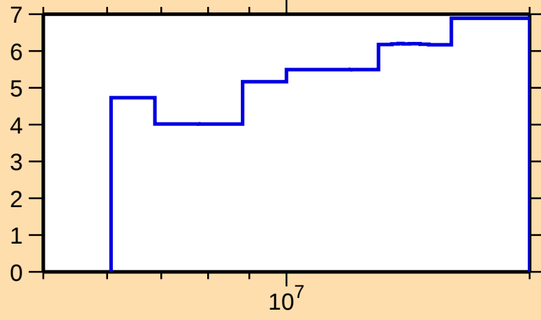
\Delta\sigma/\sigma vs. E for ^{103}\text{Nb}(n,\text{tot.})
