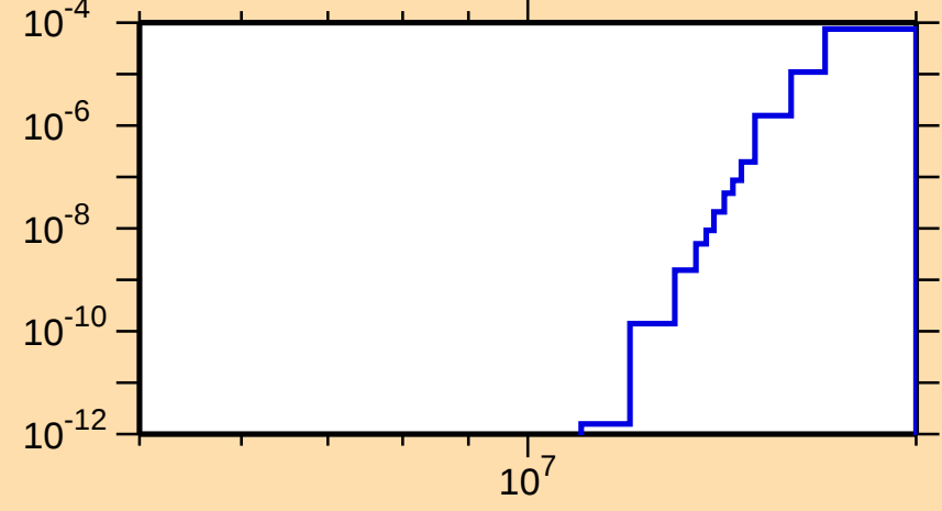
\sigma vs. E for ^{103}\text{Nb}(n,\alpha)
