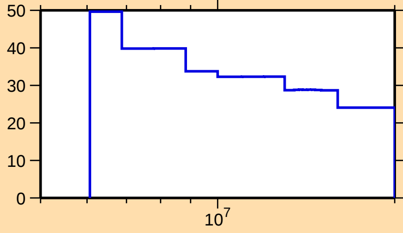
\Delta\sigma/\sigma vs. E for ^{103}\text{Nb}(n,n_1)
