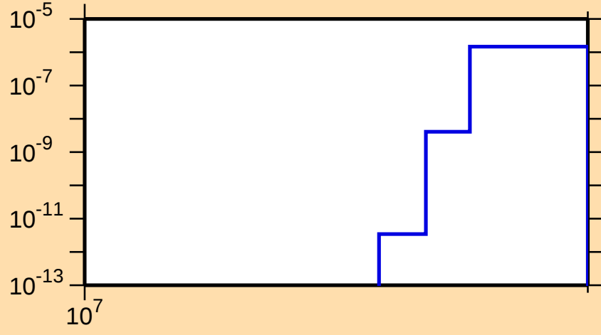
\sigma vs. E for ^{103}\text{Nb}(n,nt)
