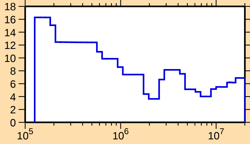
\Delta\sigma/\sigma vs. E for ^{103}\text{Nb}(n,\text{tot.})
