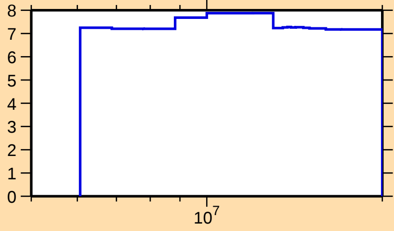
\Delta\sigma/\sigma vs. E for ^{103}\text{Nb}(n,\text{nonel.})
