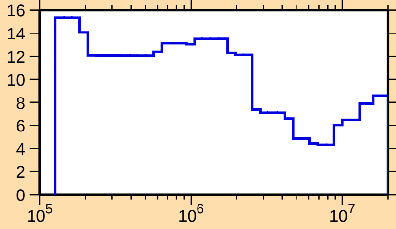
\Delta\sigma/\sigma vs. E for ^{103}\text{Nb}(n,\text{el.})
