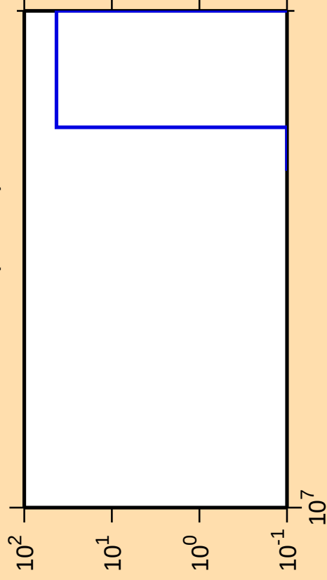
\Delta\sigma/\sigma vs. E for ^{103}\text{Nb}(n,2n\alpha)
