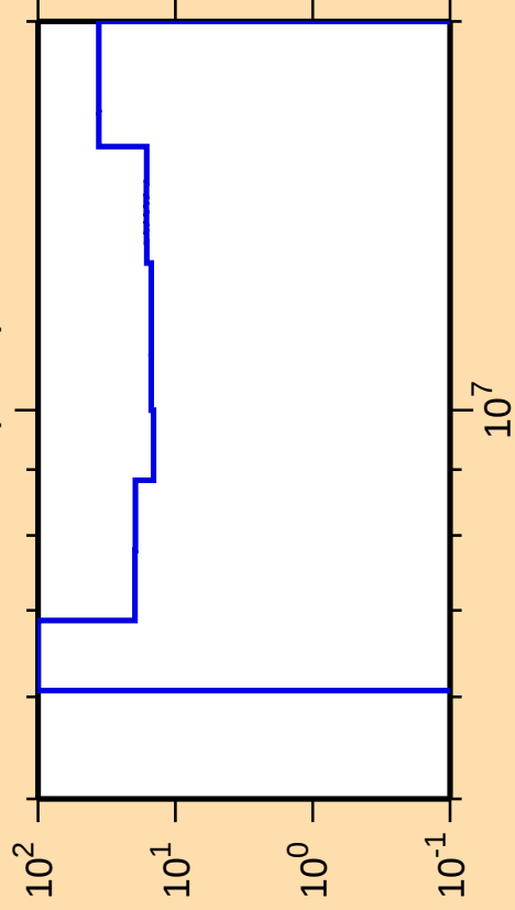
\Delta\sigma/\sigma vs. E for ^{103}\text{Nb}(n,2n)
