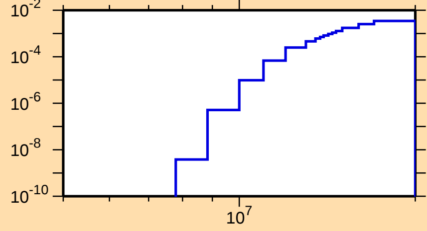
\sigma vs. E for ^{103}\text{Nb}(n,p)
