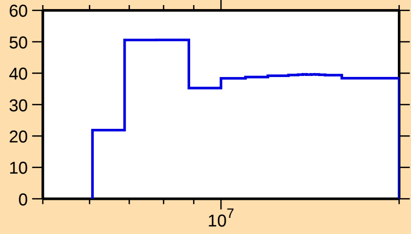
\Delta\sigma/\sigma vs. E for ^{103}\text{Nb}(n,n\text{cont.})
