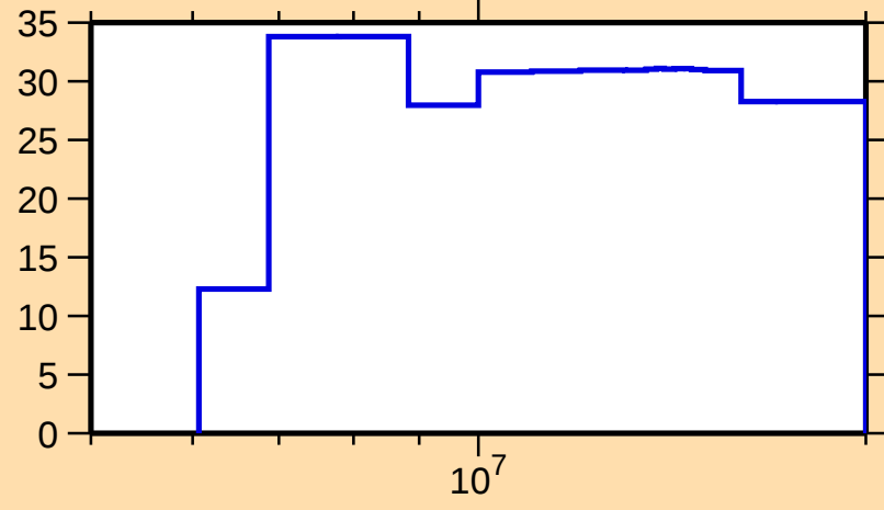
\Delta\sigma/\sigma vs. E for ^{103}\text{Nb}(n,\text{inel.})
