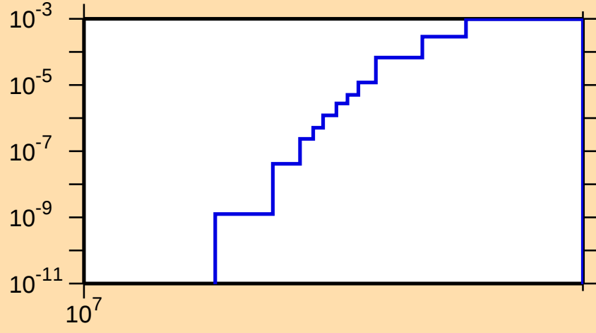
\sigma vs. E for ^{103}\text{Nb}(n,np)
