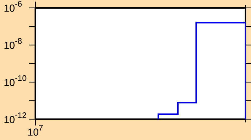
\sigma vs. E for ^{103}\text{Nb}(n,\text{nd})
