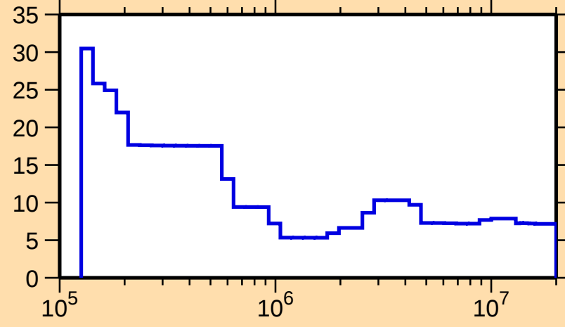
\Delta\sigma/\sigma vs. E for ^{103}\text{Nb}(n,\text{nonel.})
