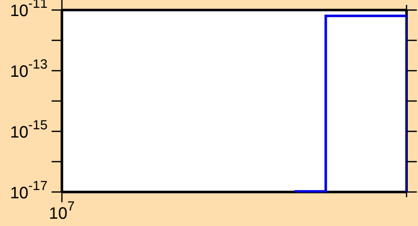
\sigma vs. E for ^{103}\text{Nb}(n,2n\alpha)
