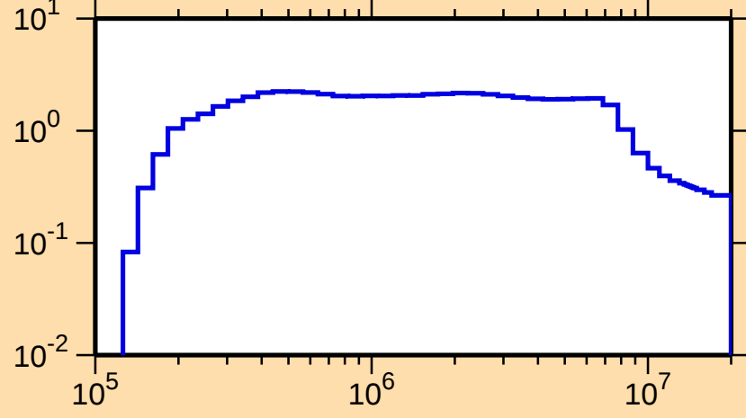
\sigma vs. E for ^{103}\text{Nb}(n,\text{inel.})
