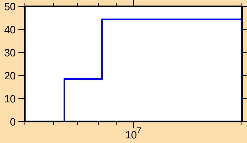
\Delta\sigma/\sigma vs. E for ^{103}\text{Nb}(n,p)
