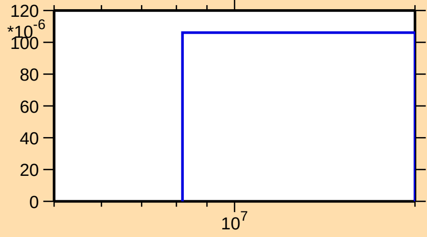
\sigma vs. E for ^{103}\text{Nb}(n,d)
