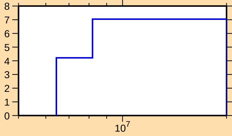
\Delta\sigma/\sigma vs. E for ^{103}\text{Nb}(n,\text{el.})
