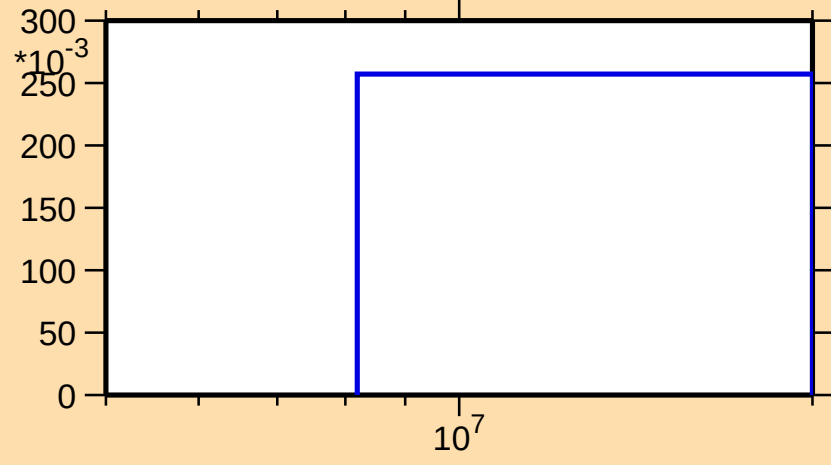
\sigma vs. E for ^{103}\text{Nb}(n,3n)
