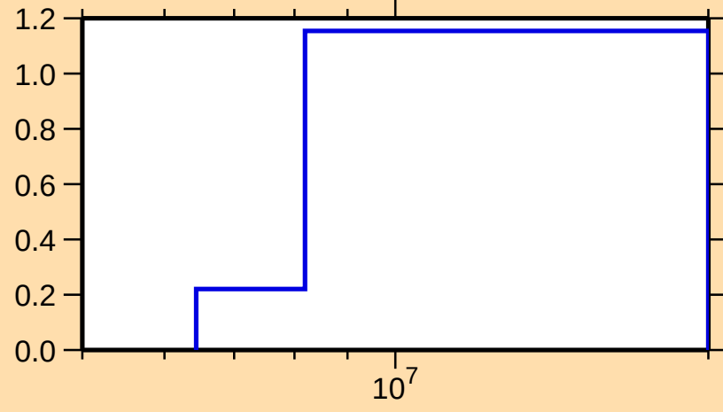
\sigma vs. E for ^{103}\text{Nb}(n,2n)
