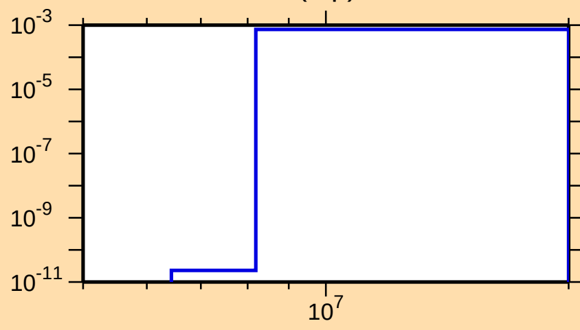
\sigma vs. E for ^{103}\text{Nb}(n,p)
