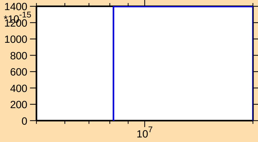
\sigma vs. E for ^{103}\text{Nb}(n,2np)
