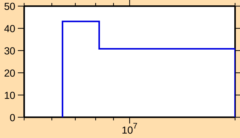
\Delta\sigma/\sigma vs. E for ^{103}\text{Nb}(n,\text{ncont.})
