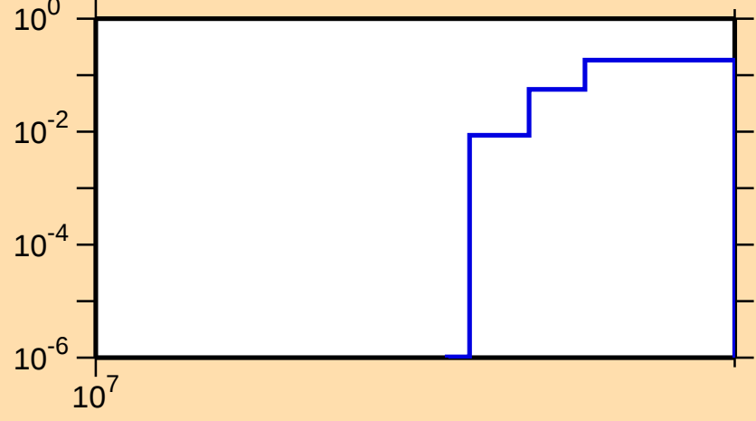
\sigma vs. E for ^{67}\text{Ni}(n,3n)
