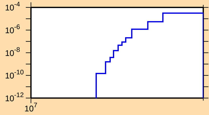
\sigma vs. E for ^{67}\text{Ni}(n,t)
