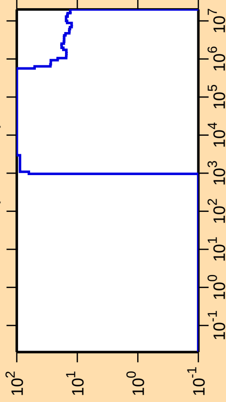
\Delta\sigma/\sigma vs. E for ^{67}\text{Ni}(n,\text{nonel.})
