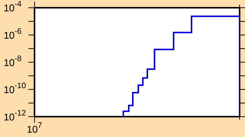
\sigma vs. E for ^{67}\text{Ni}(n,n\alpha)
