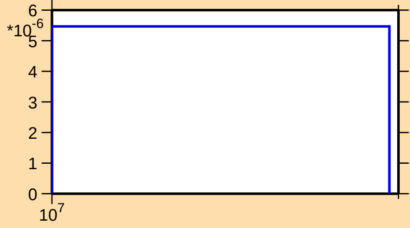
\sigma vs. E for ^{67}\text{Ni}(n,d)
