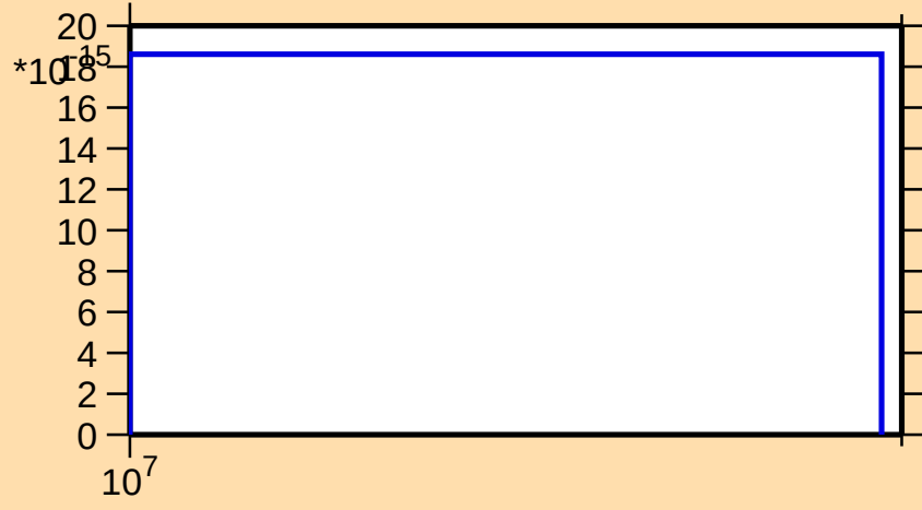
\sigma vs. E for ^{67}\text{Ni}(n,2n\alpha)
