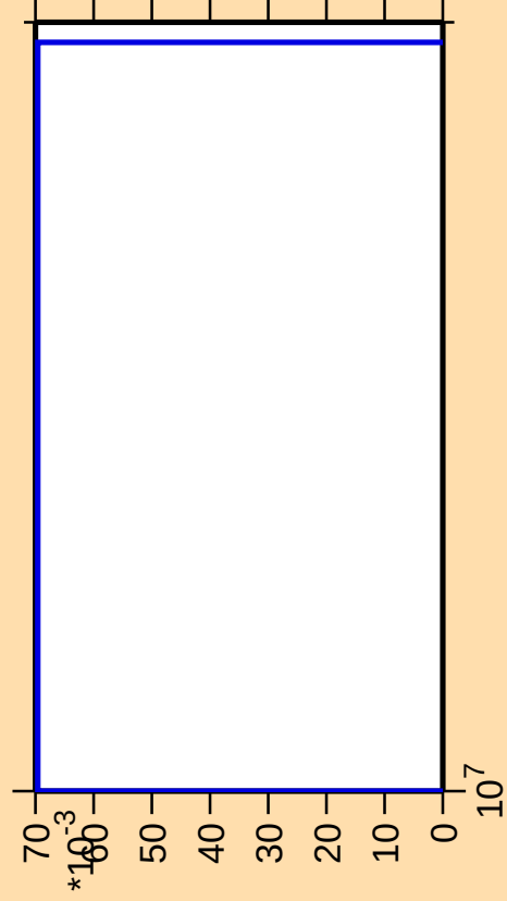
\Delta\sigma/\sigma vs. E for ^{67}\text{Ni}(n,2n\alpha)
