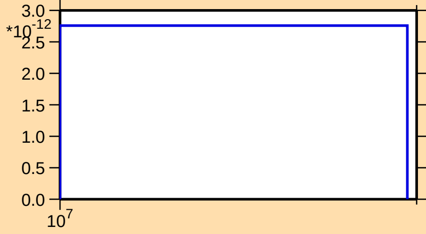
\sigma vs. E for ^{67}\text{Ni}(n,\text{nd})
