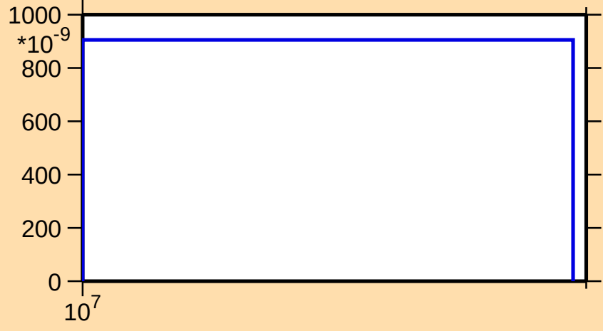
\sigma vs. E for ^{67}\text{Ni}(n,np)
