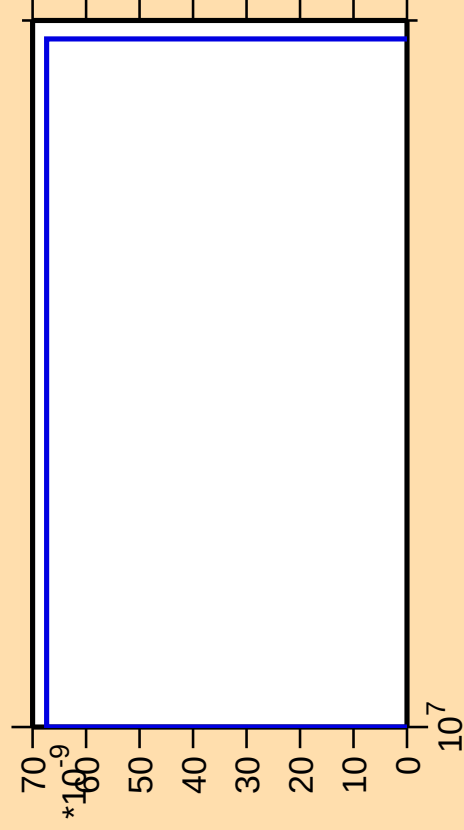
\Delta\sigma/\sigma vs. E for ^{67}\text{Ni}(n,\text{nt})
