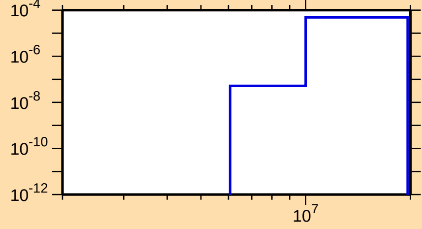
\sigma vs. E for ^{67}\text{Ni}(n,\alpha)
