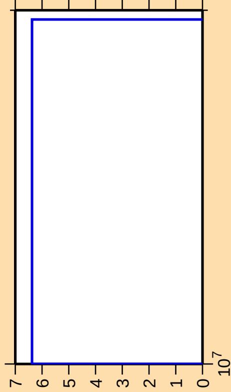
\Delta\sigma/\sigma vs. E for ^{67}\text{Ni}(n,\text{nd})
