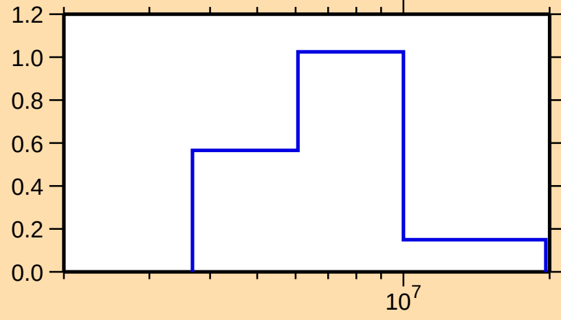
\sigma vs. E for ^{67}\text{Ni}(n,n\text{cont.})
