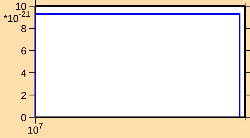
\sigma vs. E for ^{67}\text{Ni}(n,\text{nt})
