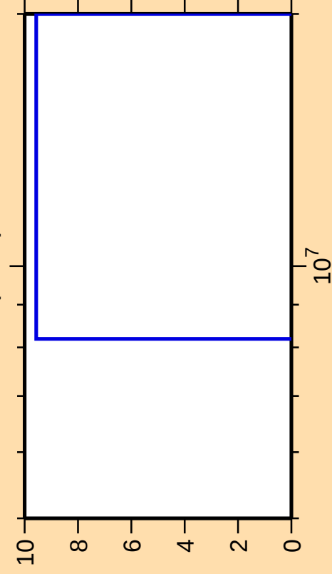
\Delta\sigma/\sigma vs. E for ^{67}\text{Ni}(n,\text{nd})
