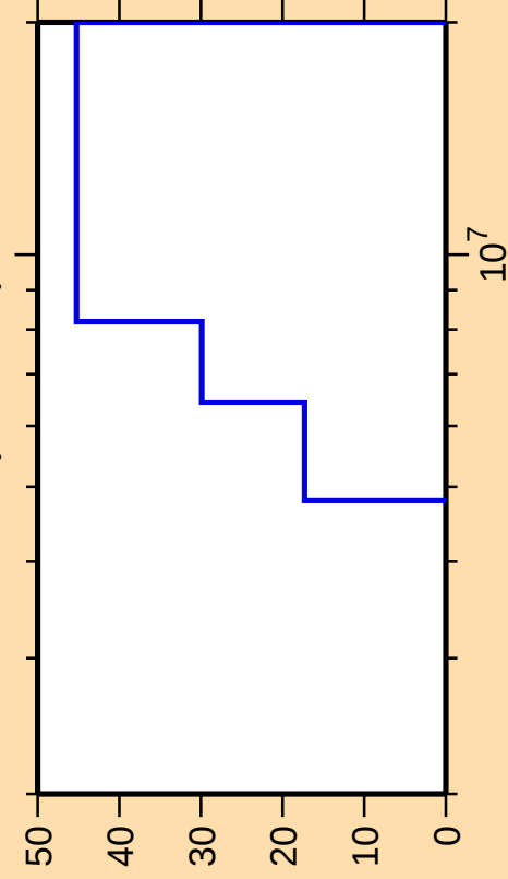
\Delta\sigma/\sigma vs. E for ^{67}\text{Ni}(n,n\text{cont.})
