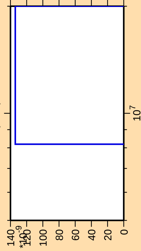
\Delta\sigma/\sigma vs. E for ^{67}\text{Ni}(n,\text{nt})
