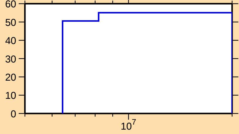
\Delta\sigma/\sigma vs. E for ^{67}\text{Ni}(n,n_1)
