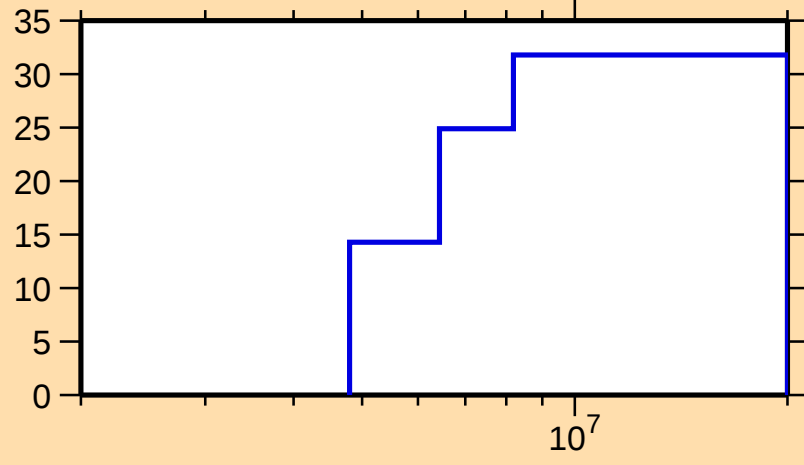
\Delta\sigma/\sigma vs. E for ^{67}\text{Ni}(n,\text{inel.})
