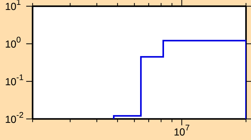
\sigma vs. E for ^{67}\text{Ni}(n,2n)
