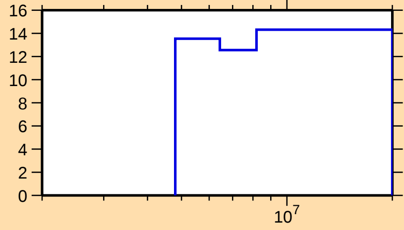
\Delta\sigma/\sigma vs. E for ^{67}\text{Ni}(n,\text{nonel.})
