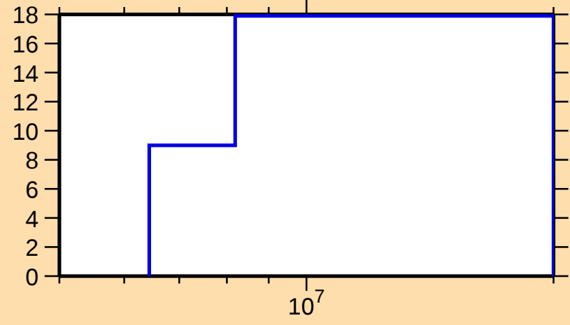
\Delta\sigma/\sigma vs. E for ^{67}\text{Ni}(n,\text{el.})
