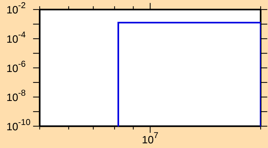
\sigma vs. E for ^{67}\text{Ni}(n,p)
