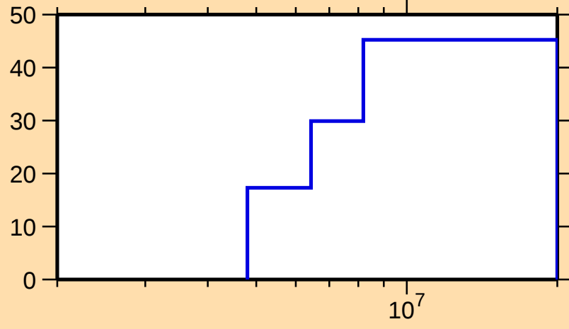
\Delta\sigma/\sigma vs. E for ^{67}\text{Ni}(n,n\text{cont.})
