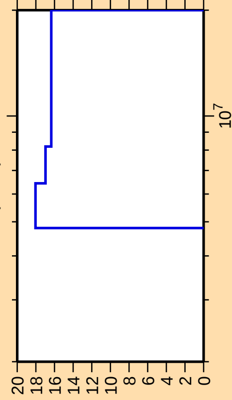
\Delta\sigma/\sigma vs. E for ^{67}\text{Ni}(n,2n)
