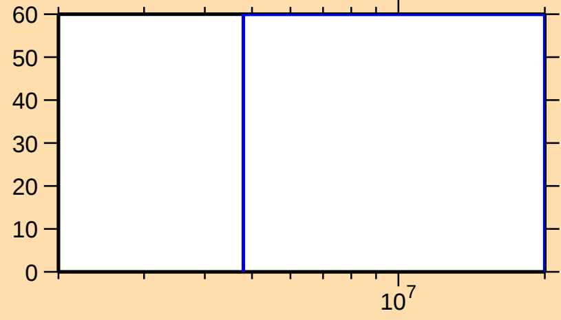
\Delta\sigma/\sigma vs. E for ^{67}\text{Ni}(n,\gamma)
