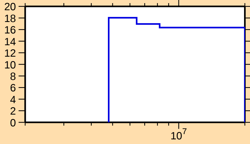
\Delta\sigma/\sigma vs. E for ^{67}\text{Ni}(n,2n)
