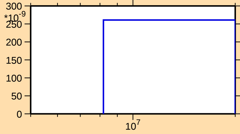
\sigma vs. E for ^{67}\text{Ni}(n,n\alpha)
