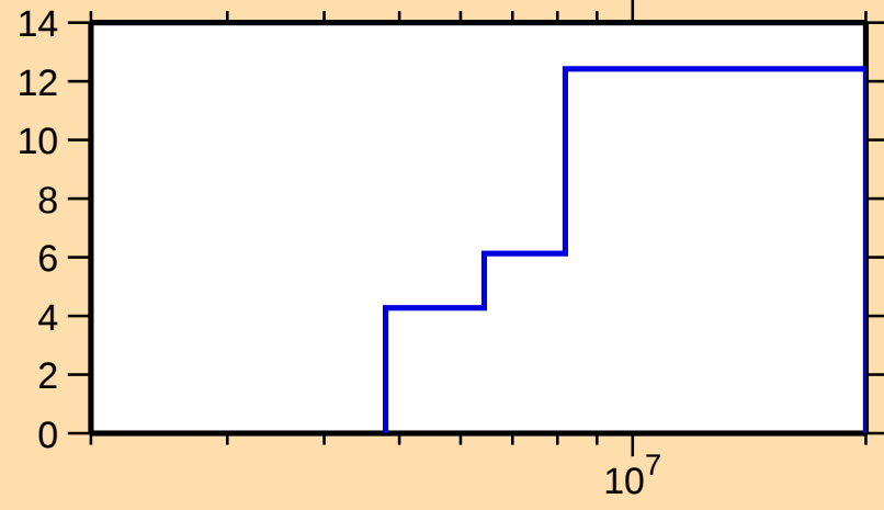
\Delta\sigma/\sigma vs. E for ^{67}\text{Ni}(n,\text{tot.})
