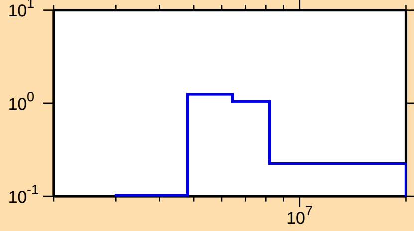
\sigma vs. E for ^{67}\text{Ni}(n,n\text{cont.})
