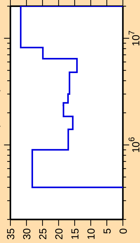
\Delta\sigma/\sigma vs. E for ^{67}\text{Ni}(n,\text{inel.})
