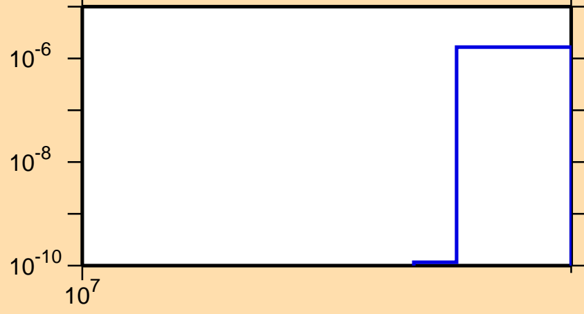
\sigma vs. E for ^{36}\text{P}(n,2np)
