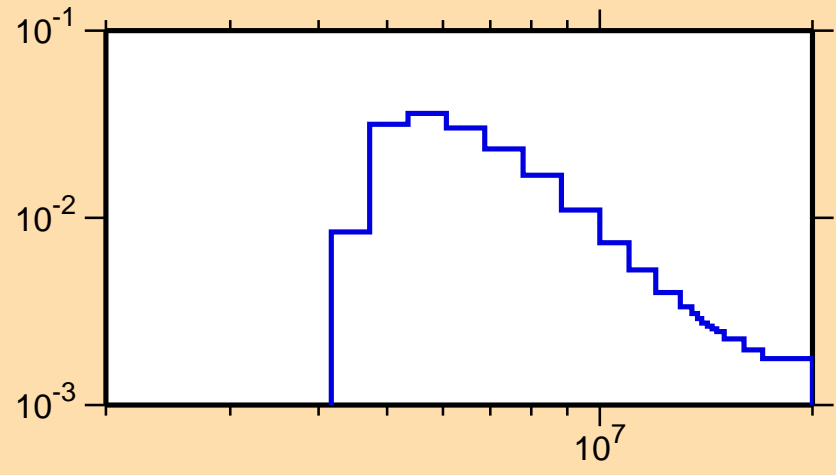
\sigma vs. E for ^{36}\text{P}(n,n\text{cont.})
