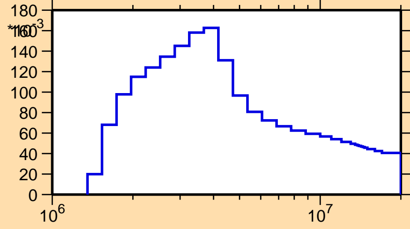
\sigma vs. E for ^{36}\text{P}(n,n_4)
