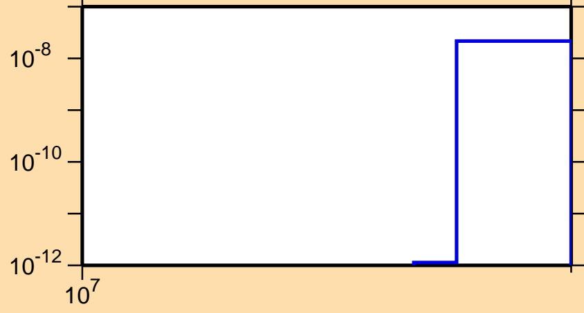
\sigma vs. E for ^{36}\text{P}(n,2n\alpha)
