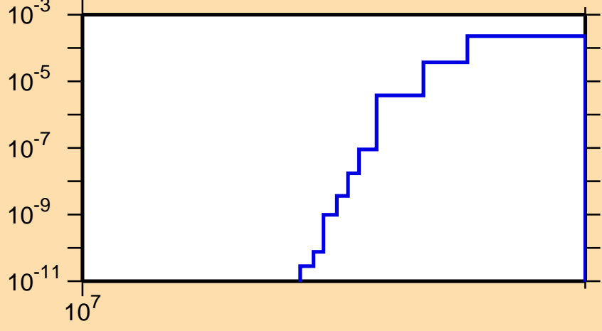
\sigma vs. E for ^{36}\text{P}(n,n\alpha)
