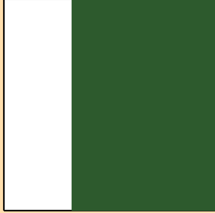
\Delta\sigma/\sigma vs. E for ^{185}\text{Pb}(n,2n)
