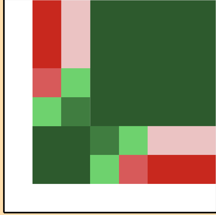
\sigma vs. E for ^{185}\text{Pb}(n,n\text{cont.})
