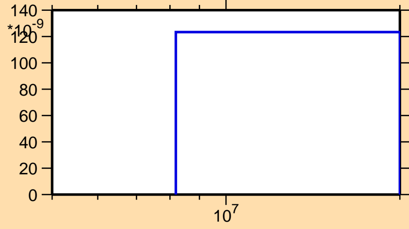
\sigma vs. E for ^{185}\text{Pb}(n,\text{nd})
