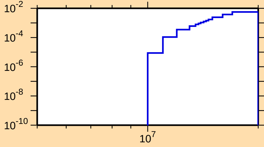
\sigma vs. E for ^{185}\text{Pb}(n,2n\alpha)
