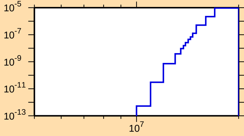
\sigma vs. E for ^{185}\text{Pb}(n,\text{pt})
