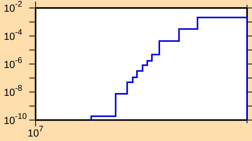
\sigma vs. E for ^{185}\text{Pb}(n,2np)
