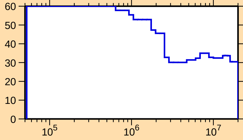
\Delta\sigma/\sigma vs. E for ^{185}\text{Pb}(n,n\text{onel.})
