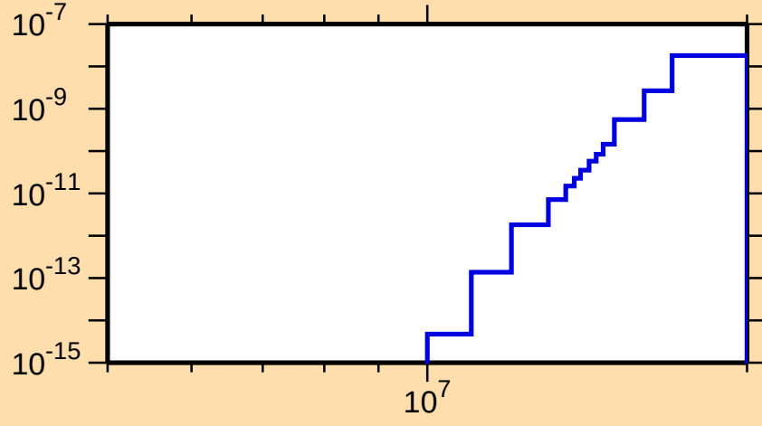
\sigma vs. E for ^{185}\text{Pb}(\text{mt } 34)
