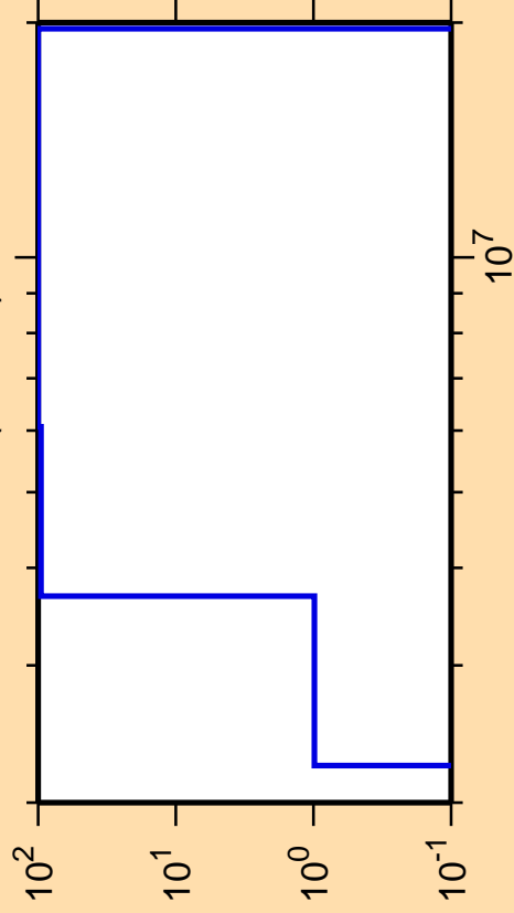
\Delta\sigma/\sigma vs. E for ^{185}\text{Pb}(n,\text{He3})
