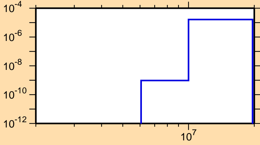
\sigma vs. E for ^{185}\text{Pb}(\text{mt } 45)
