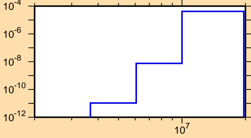
\sigma vs. E for ^{185}\text{Pb}(n,\text{He3})
