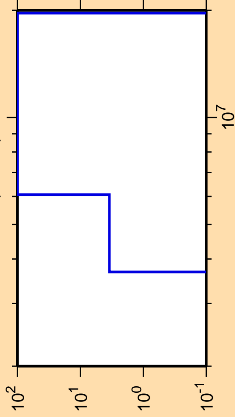
\Delta\sigma/\sigma vs. E for ^{185}\text{Pb}(\text{mt } 45)
