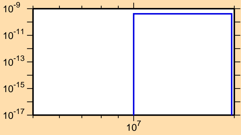
\sigma vs. E for ^{185}\text{Pb} (mt 34)
