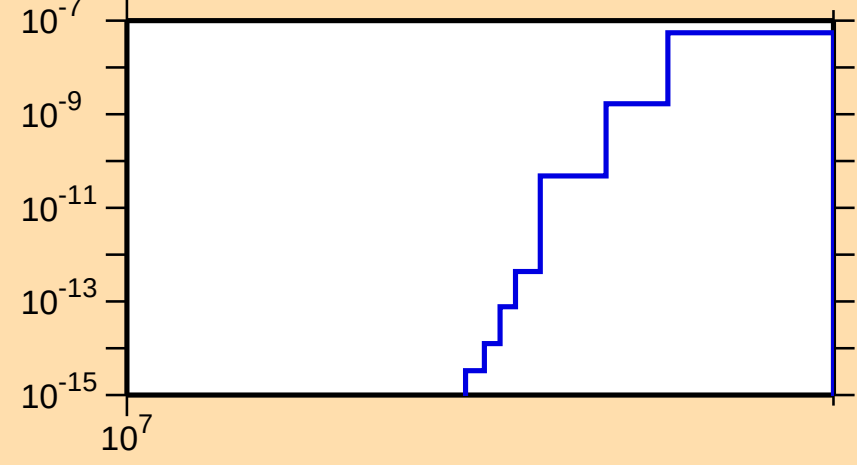
\sigma vs. E for ^{186}\text{Pb}(n,\text{nd})
