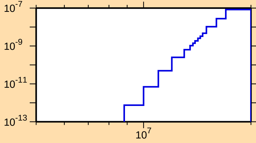
\sigma vs. E for ^{186}\text{Pb}(\text{mt117})
