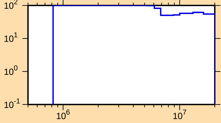
\Delta\sigma/\sigma vs. E for ^{186}\text{Pb}(n,n\text{cont.})
