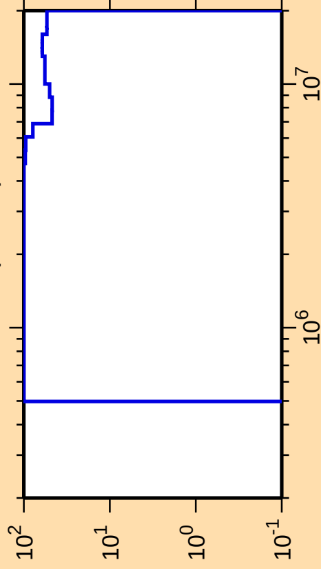
\Delta\sigma/\sigma vs. E for ^{186}\text{Pb}(n,\text{inel.})
