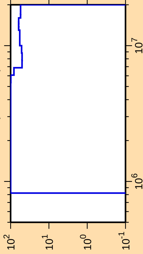
\Delta\sigma/\sigma vs. E for ^{186}\text{Pb}(n,\text{ncont.})
