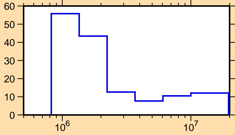
\Delta\sigma/\sigma vs. E for ^{186}\text{Pb}(n,n\text{nonel.})
