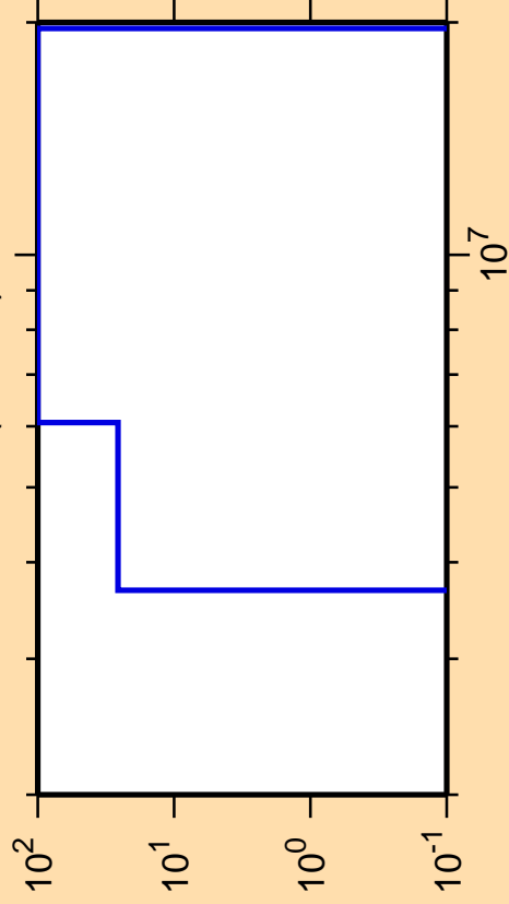
\Delta\sigma/\sigma vs. E for ^{186}\text{Pb}(n,\text{He3})
