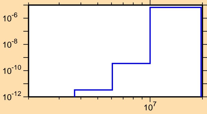
\sigma vs. E for ^{186}\text{Pb}(n,\text{He3})
