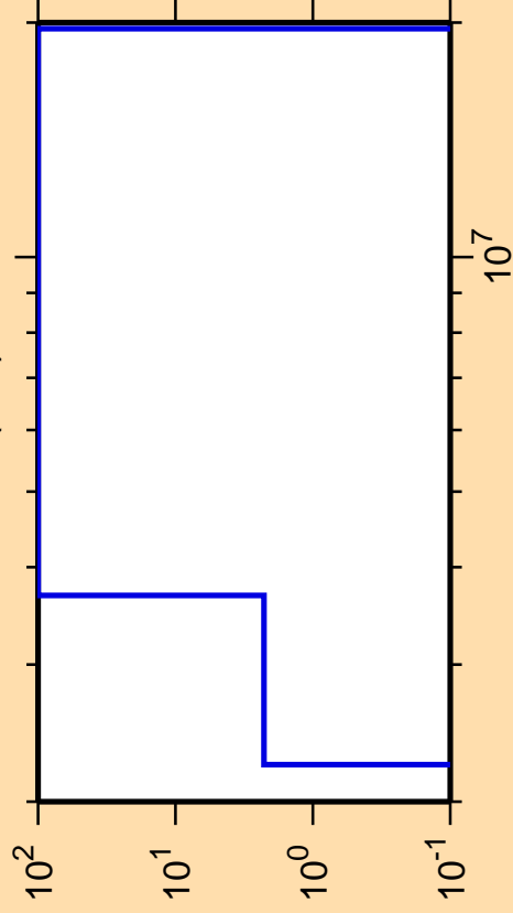
\Delta\sigma/\sigma vs. E for ^{186}\text{Pb}(n,d)
