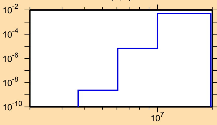
\sigma vs. E for ^{186}\text{Pb}(n,d)
