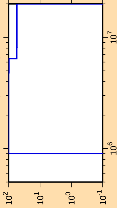
\Delta\sigma/\sigma vs. E for ^{186}\text{Pb}(n,n\text{cont.})
