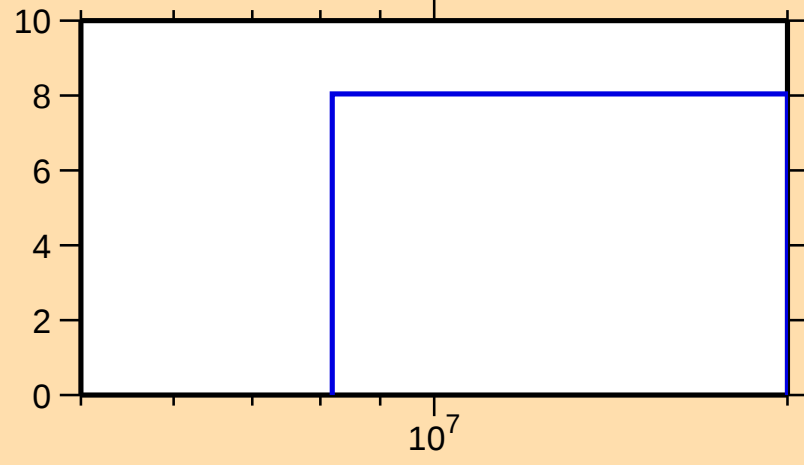
\Delta\sigma/\sigma vs. E for ^{186}\text{Pb}(n,\text{tot.})
