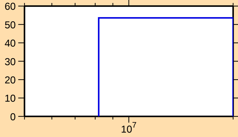
\Delta\sigma/\sigma vs. E for ^{186}\text{Pb}(n,\text{inel.})
