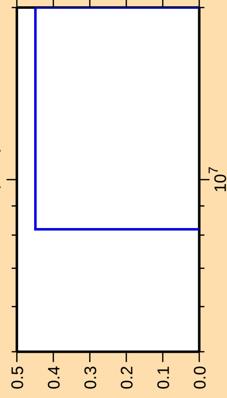
\Delta\sigma/\sigma vs. E for ^{186}\text{Pb}(n,nt)
