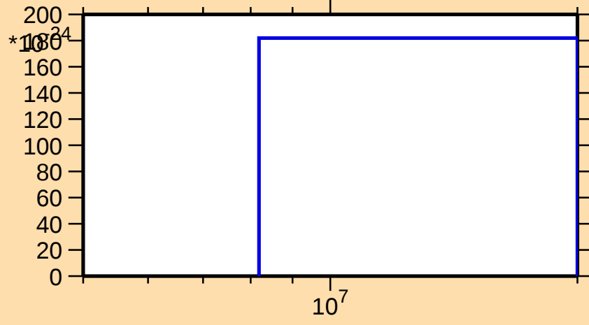
\sigma vs. E for ^{186}\text{Pb}(\text{mt 11})
