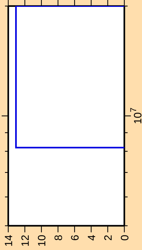
\Delta\sigma/\sigma vs. E for ^{186}\text{Pb}(\text{mt } 34)
