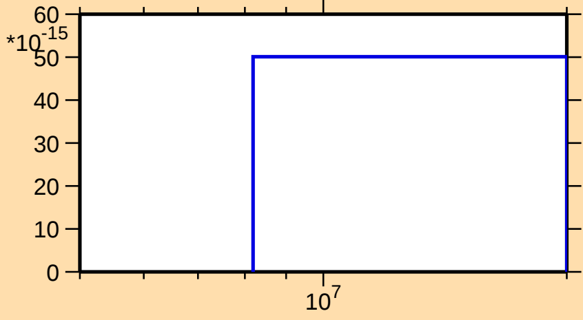
\sigma vs. E for ^{186}\text{Pb}(n,nt)
