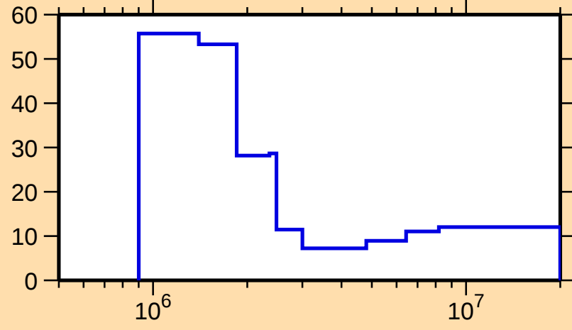
\Delta\sigma/\sigma vs. E for ^{186}\text{Pb}(n,n\text{onel.})
