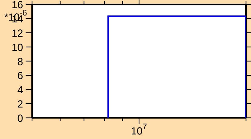
\sigma vs. E for ^{186}\text{Pb}(n,2n\alpha)
