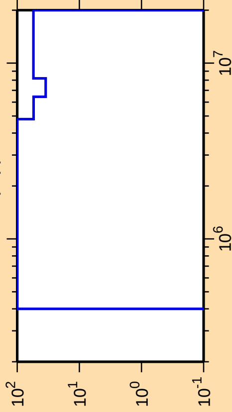
\Delta\sigma/\sigma vs. E for ^{186}\text{Pb}(n,p)
