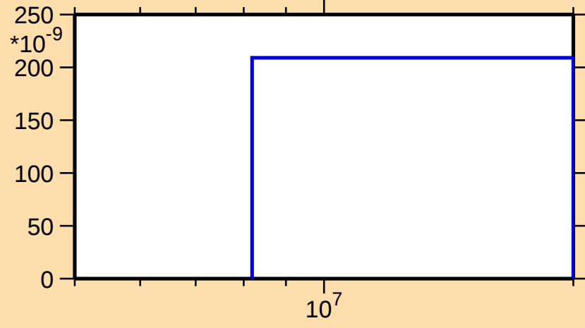
\sigma vs. E for ^{186}\text{Pb}(n,2np)
