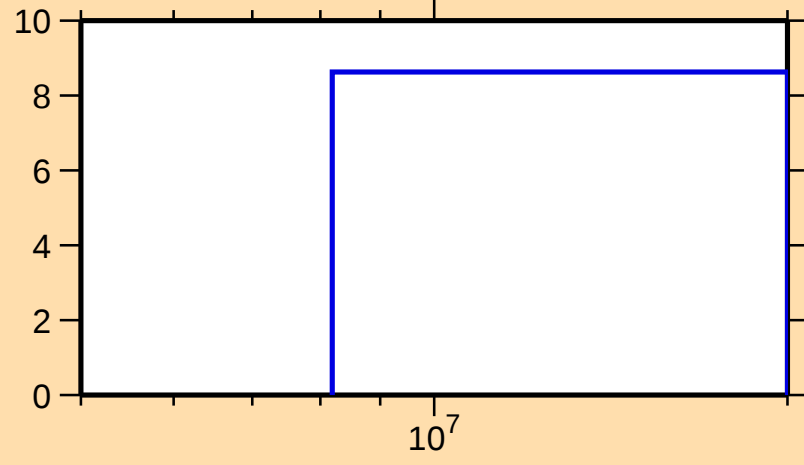
\Delta\sigma/\sigma vs. E for ^{186}\text{Pb}(n,\text{el.})
