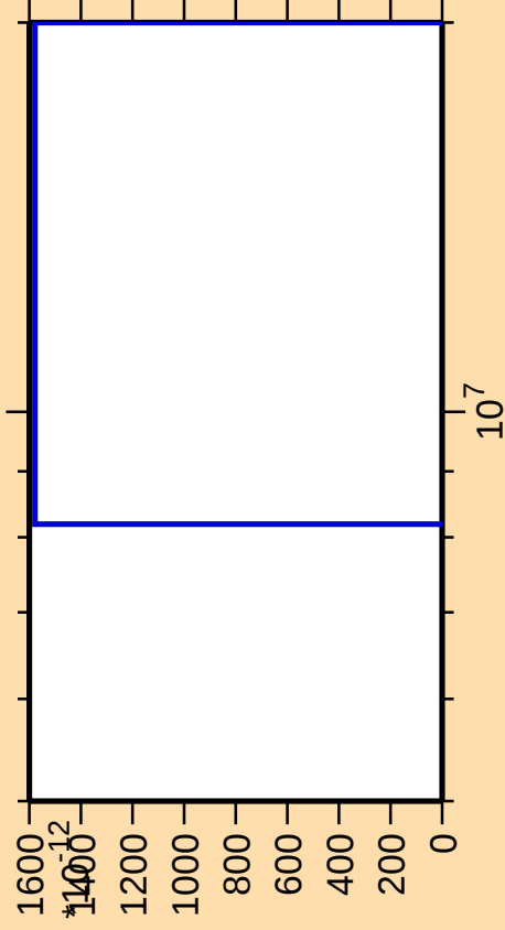
\Delta\sigma/\sigma vs. E for ^{186}\text{Pb}(\text{mt 11})
