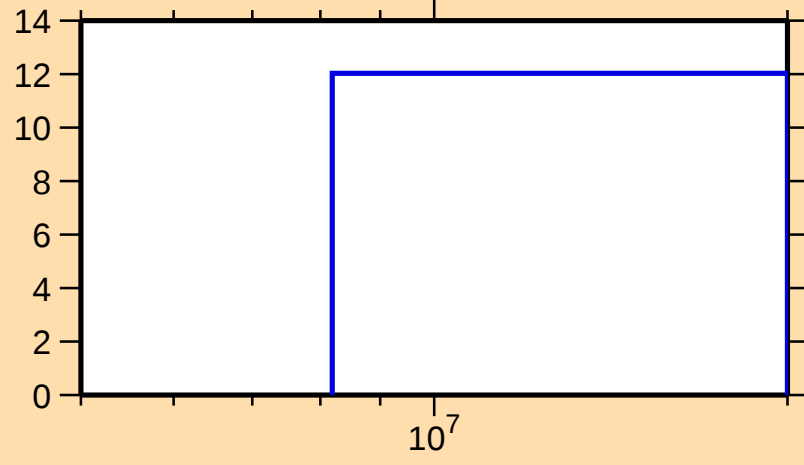
\Delta\sigma/\sigma vs. E for ^{186}\text{Pb}(n,\text{nonel.})
