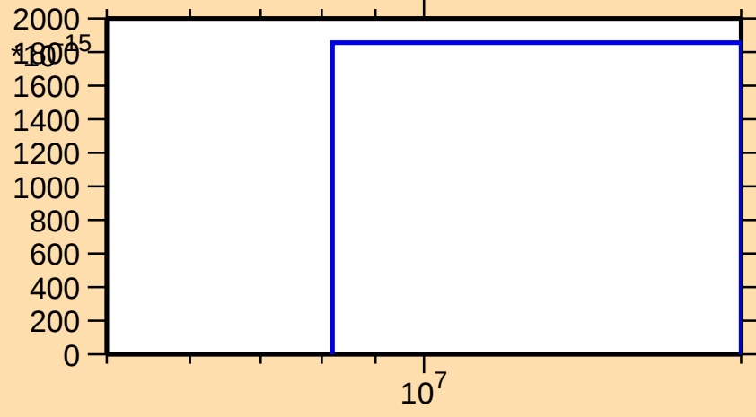
\sigma vs. E for ^{186}\text{Pb}(\text{mt } 34)
