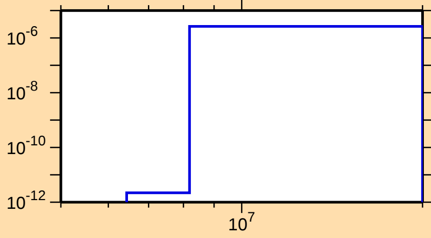
\sigma vs. E for ^{186}\text{Pb}(\text{mt } 45)
