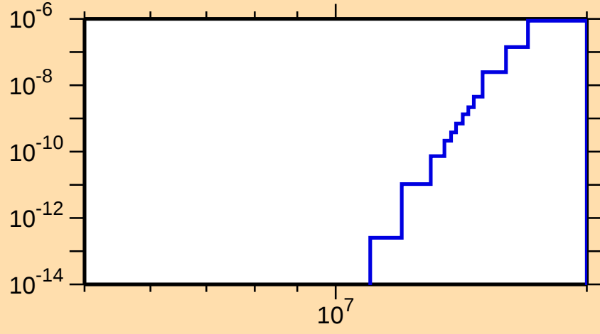
\sigma vs. E for ^{187}\text{Pb}(n,\text{pt})
