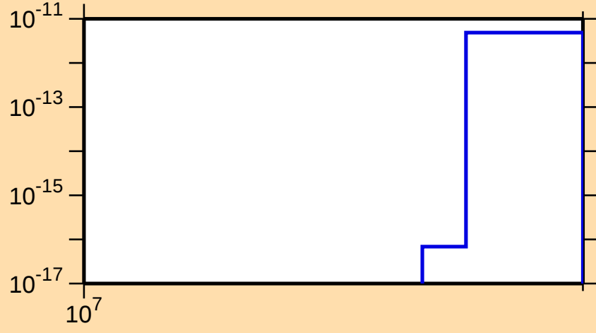
\sigma vs. E for ^{187}\text{Pb}(n,nt)
