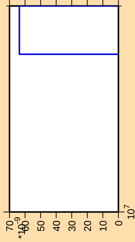
\Delta\sigma/\sigma vs. E for ^{187}\text{Pb}(\text{mt 11})
