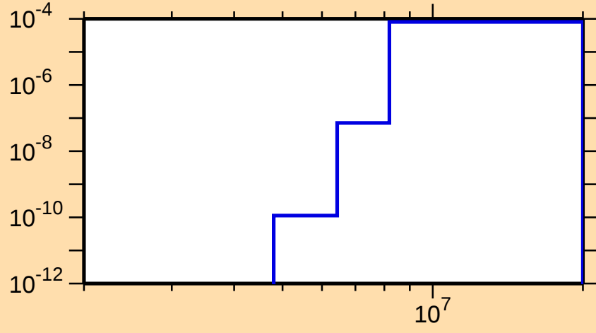
\sigma vs. E for ^{187}\text{Pb}(\text{mt } 45)
