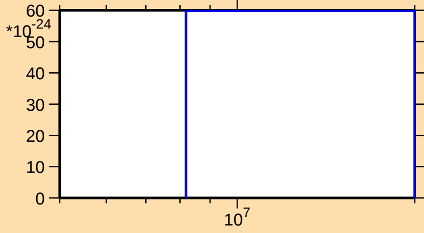
\sigma vs. E for ^{187}\text{Pb}(\text{mt } 11)
