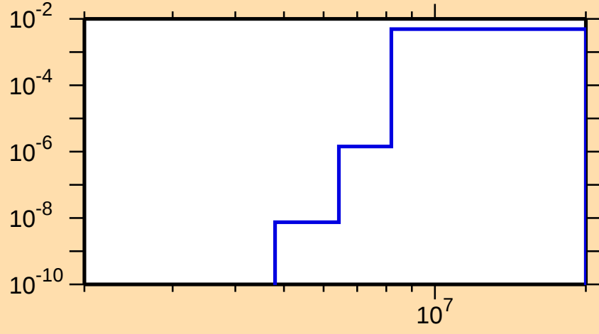
\sigma vs. E for ^{187}\text{Pb}(n,d)
