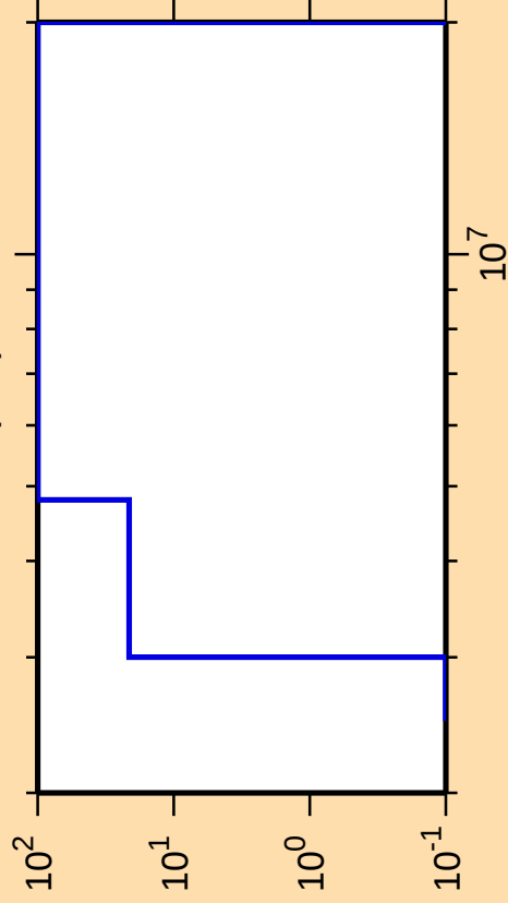
\Delta\sigma/\sigma vs. E for ^{187}\text{Pb}(n,d)
