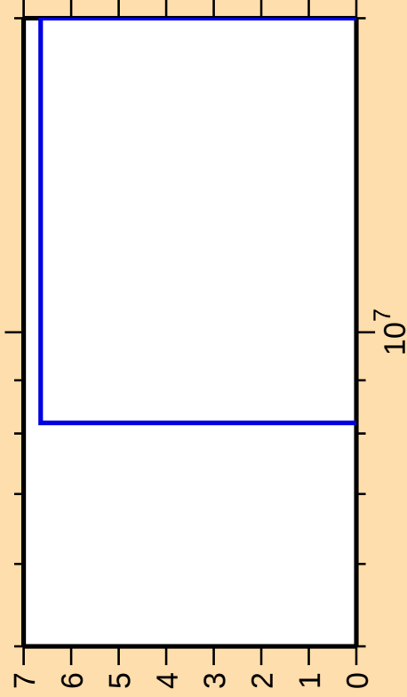
\Delta\sigma/\sigma vs. E for ^{187}\text{Pb}(n,3n)
