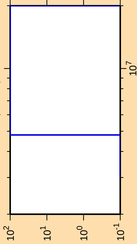
\Delta\sigma/\sigma vs. E for ^{187}\text{Pb}(\text{mt } 45)
