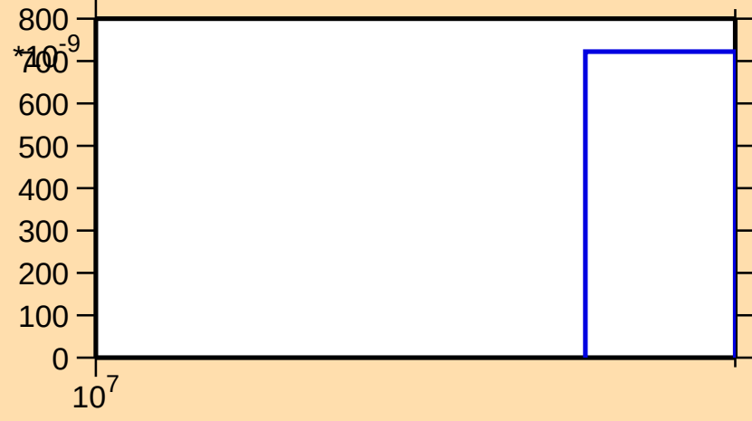
\sigma vs. E for ^{189}\text{Pb}(n,3n)
