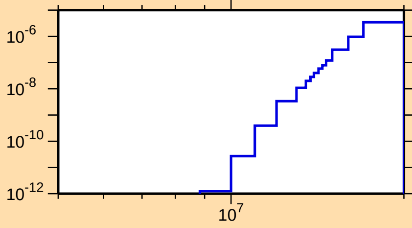
\sigma vs. E for ^{189}\text{Pb}(\text{mt } 45)
