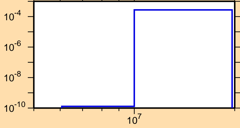
\sigma vs. E for ^{189}\text{Pb}(n,2n\alpha)
