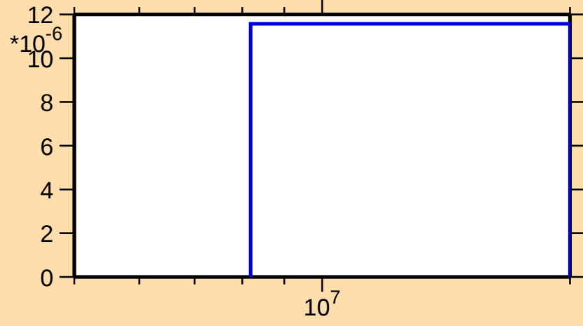
\sigma vs. E for ^{189}\text{Pb}(n,2np)
