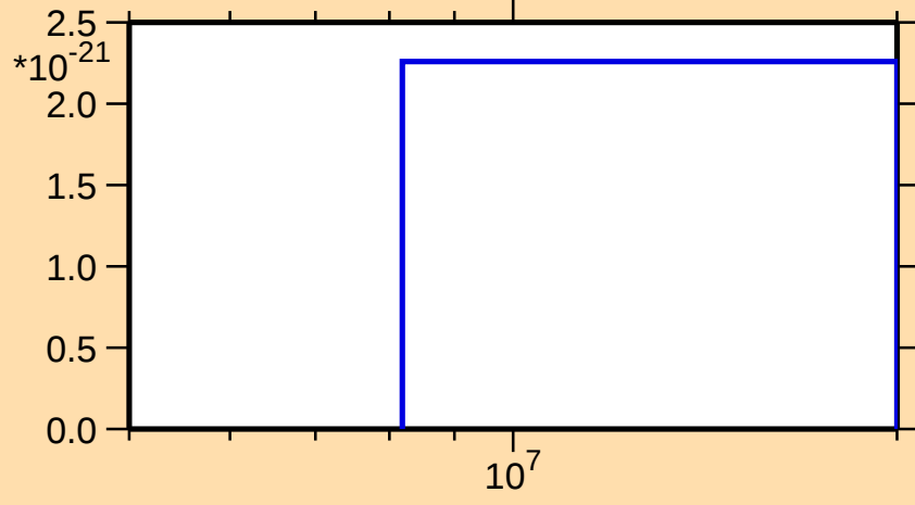
\sigma vs. E for ^{189}\text{Pb}(\text{mt } 11)
