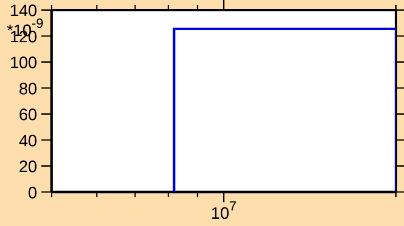
\sigma vs. E for ^{189}\text{Pb}(\text{mt } 45)
