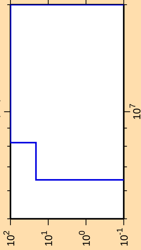
\Delta\sigma/\sigma vs. E for ^{189}\text{Pb}(n,t)
