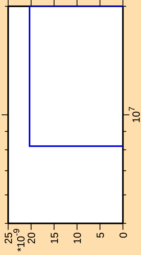
\Delta\sigma/\sigma vs. E for ^{189}\text{Pb}(\text{mt } 11)
