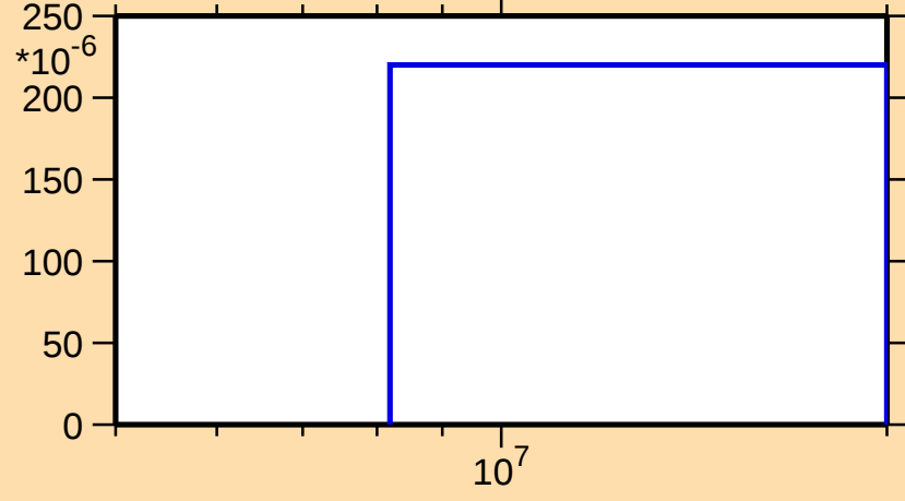
\sigma vs. E for ^{189}\text{Pb}(n,2n\alpha)
