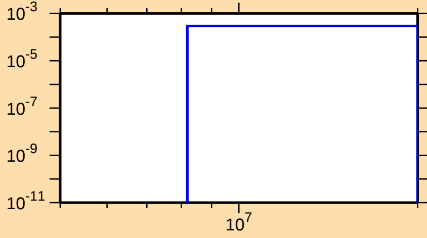
\sigma vs. E for ^{189}\text{Pb}(n,t)
