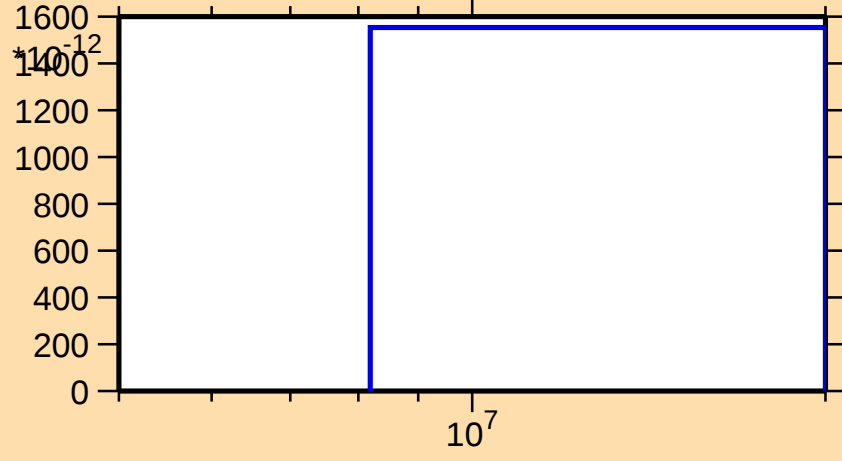
\sigma vs. E for ^{189}\text{Pb}(n,\text{pt})
