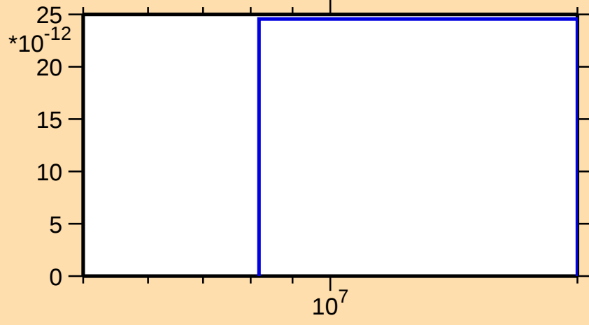
\sigma vs. E for ^{189}\text{Pb}(\text{mt } 34)
