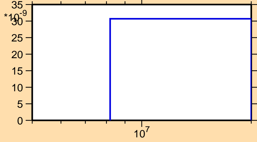
\sigma vs. E for ^{191}\text{Pb}(n,3n)
