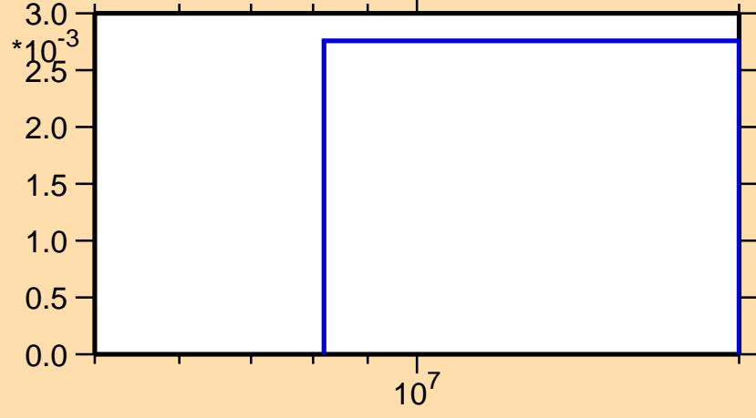
\sigma vs. E for ^{191}\text{Pb}(n,2n\alpha)
