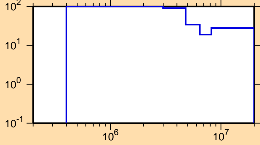
\Delta\sigma/\sigma vs. E for ^{191}\text{Pb}(n,ncont.)
