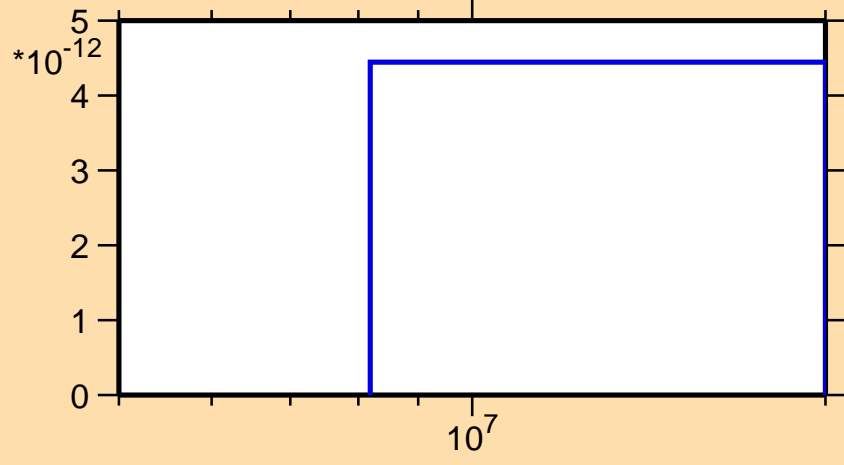
\sigma vs. E for ^{191}\text{Pb} (mt 34)
