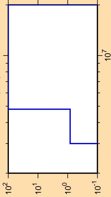
\Delta\sigma/\sigma vs. E for ^{191}\text{Pb}(n,d)
