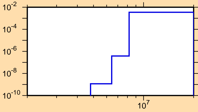
\sigma vs. E for ^{191}\text{Pb}(n,d)
