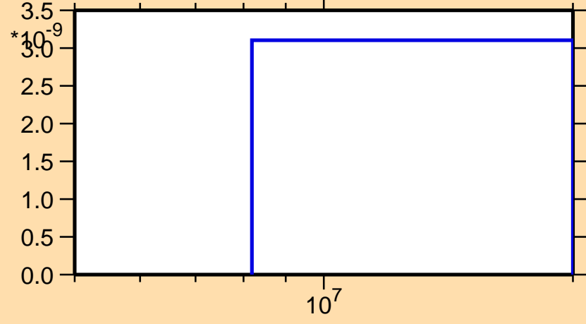
\sigma vs. E for ^{191}\text{Pb}(n,\text{pd})
