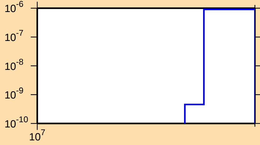
\sigma vs. E for ^{194}\text{Pb}(n,2np)
