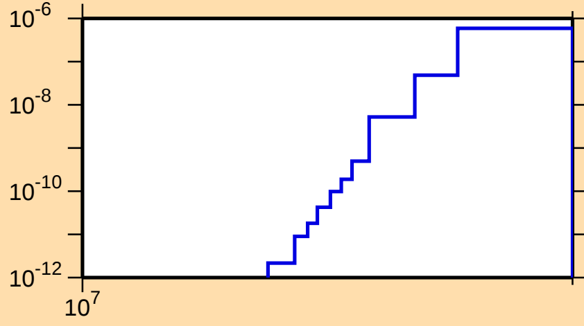
\sigma vs. E for ^{194}\text{Pb}(n,2n\alpha)
