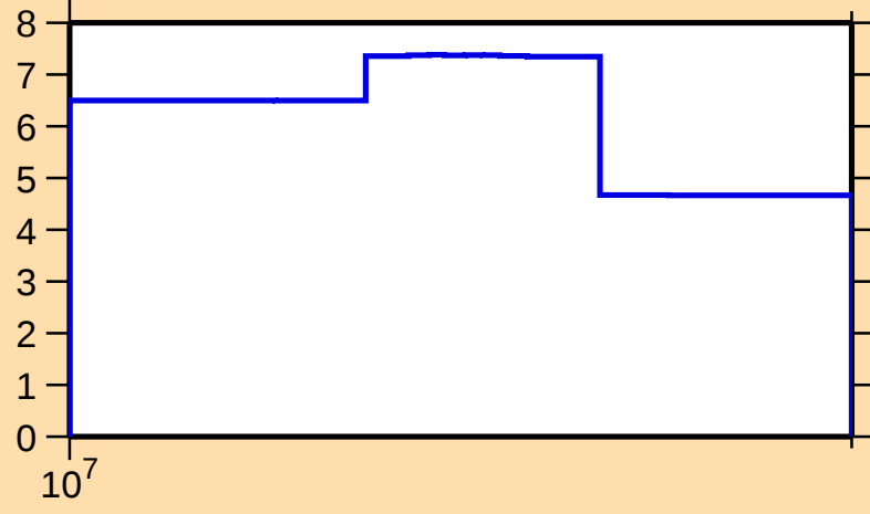
\Delta\sigma/\sigma vs. E for ^{194}\text{Pb}(n,\text{el.})
