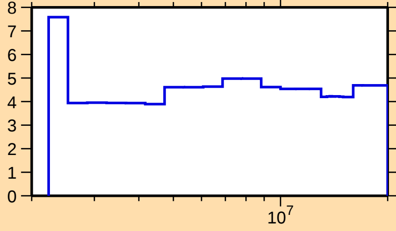
\Delta\sigma/\sigma vs. E for ^{194}\text{Pb}(n,n\text{onel.})
