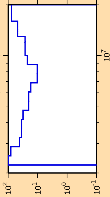
\Delta\sigma/\sigma vs. E for ^{194}\text{Pb}(n,\text{ncont.})
