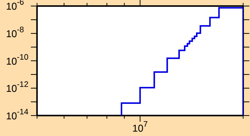
\sigma vs. E for ^{194}\text{Pb}(n,\text{He}3)
