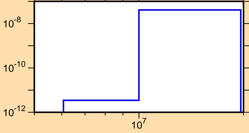
\sigma vs. E for ^{194}\text{Pb}(n,p\alpha)
