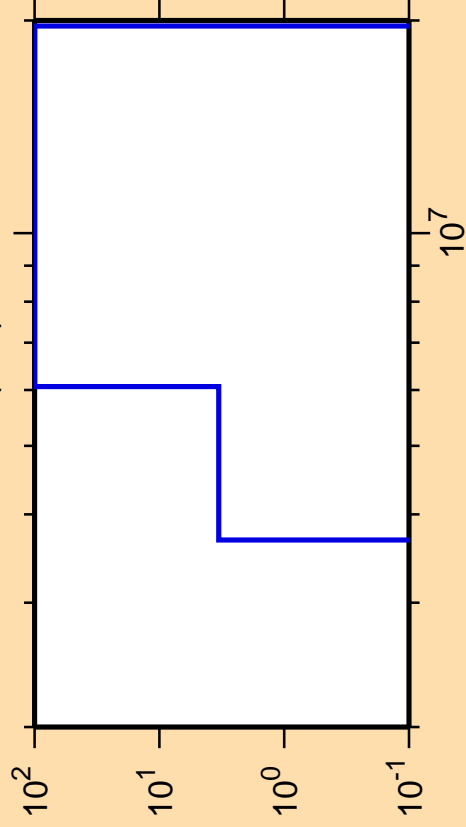
\Delta\sigma/\sigma vs. E for ^{194}\text{Pb}(n,d)
