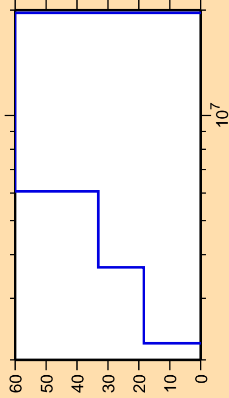
\Delta\sigma/\sigma vs. E for ^{194}\text{Pb}(n,\gamma)
