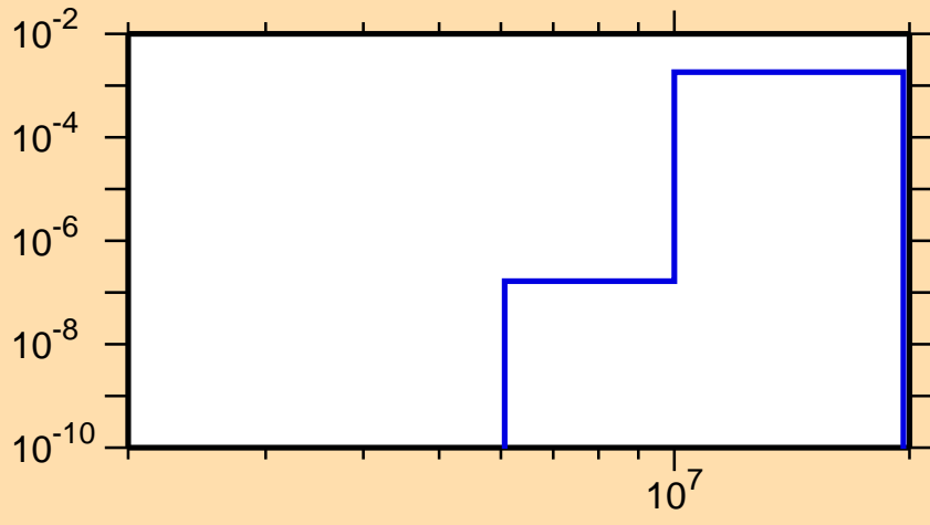
\sigma vs. E for ^{194}\text{Pb}(n,d)
