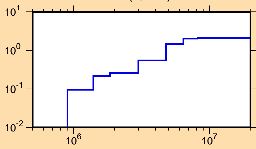
\sigma vs. E for ^{194}\text{Pb}(n,\text{inel.})
