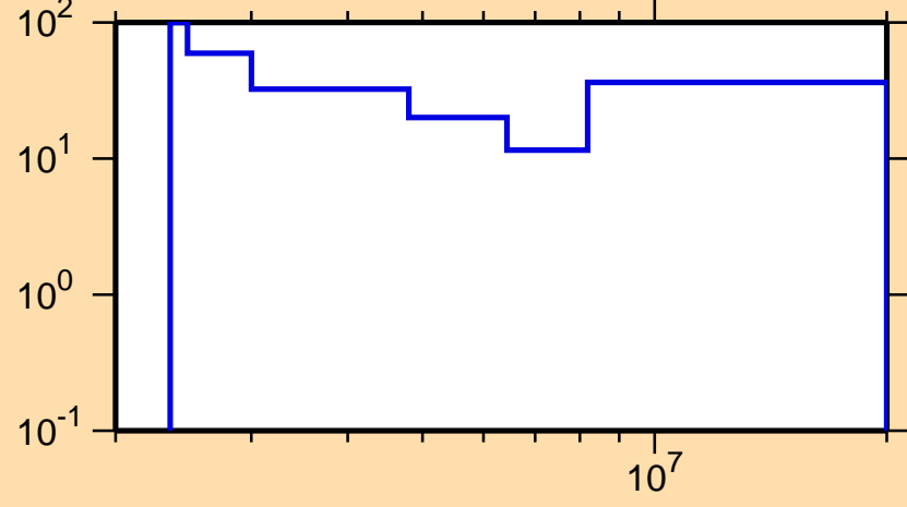
\Delta\sigma/\sigma vs. E for ^{194}\text{Pb}(n,n\text{cont.})
