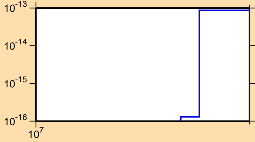
\sigma vs. E for ^{196}\text{Pb}(\text{mt } 34)
