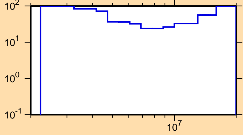
\Delta\sigma/\sigma vs. E for ^{196}\text{Pb}(n,n\text{cont.})
