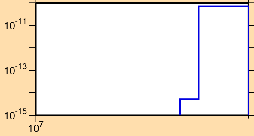
\sigma vs. E for ^{196}\text{Pb}(n,nt)
