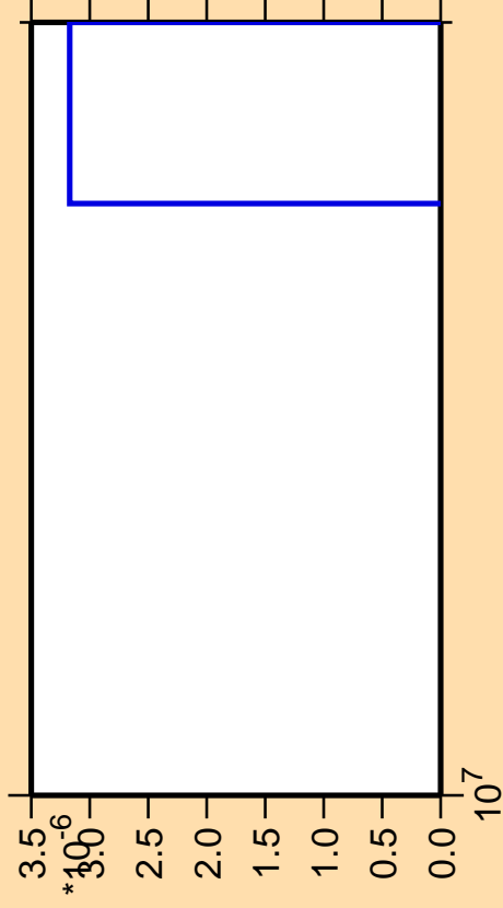
\Delta\sigma/\sigma vs. E for ^{196}\text{Pb}(\text{mt } 11)
