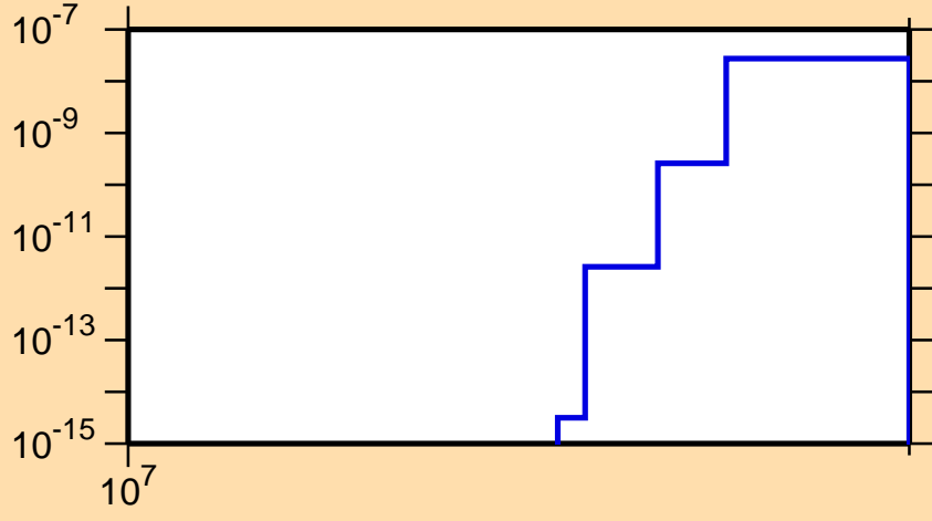
\sigma vs. E for ^{196}\text{Pb}(n,\text{nd})
