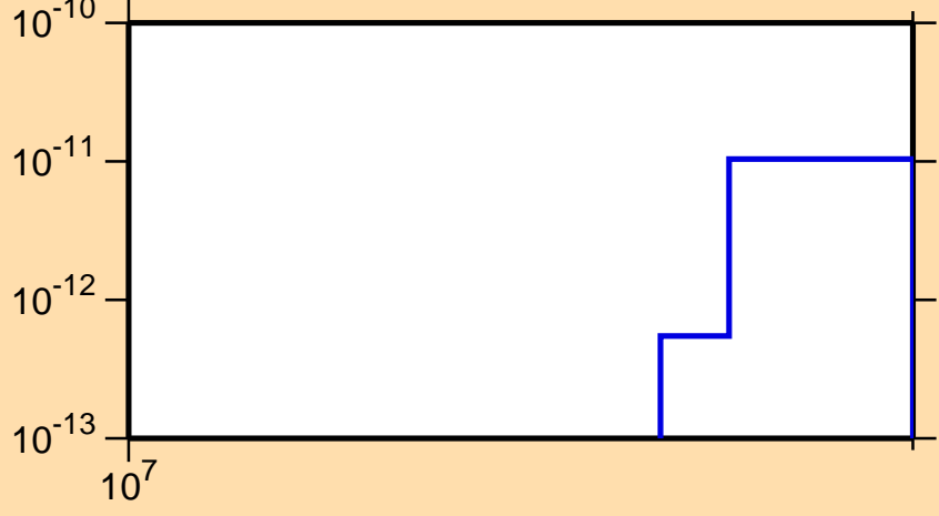
\sigma vs. E for ^{196}\text{Pb} (mt 45)
