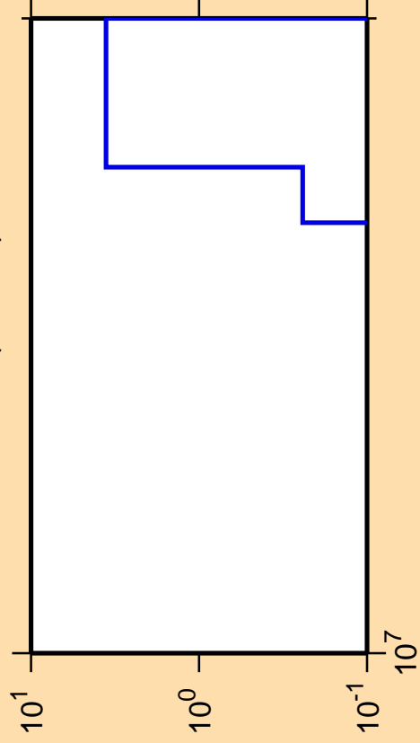
\Delta\sigma/\sigma vs. E for ^{196}\text{Pb}(\text{mt117})
