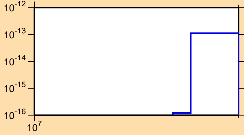
\sigma vs. E for ^{196}\text{Pb}(n,\text{pt})
