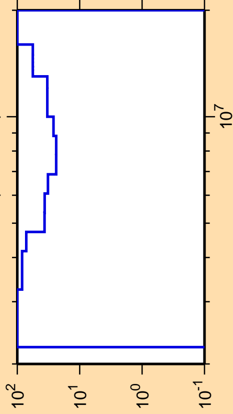
\Delta\sigma/\sigma vs. E for ^{196}\text{Pb}(n,n\text{cont.})
