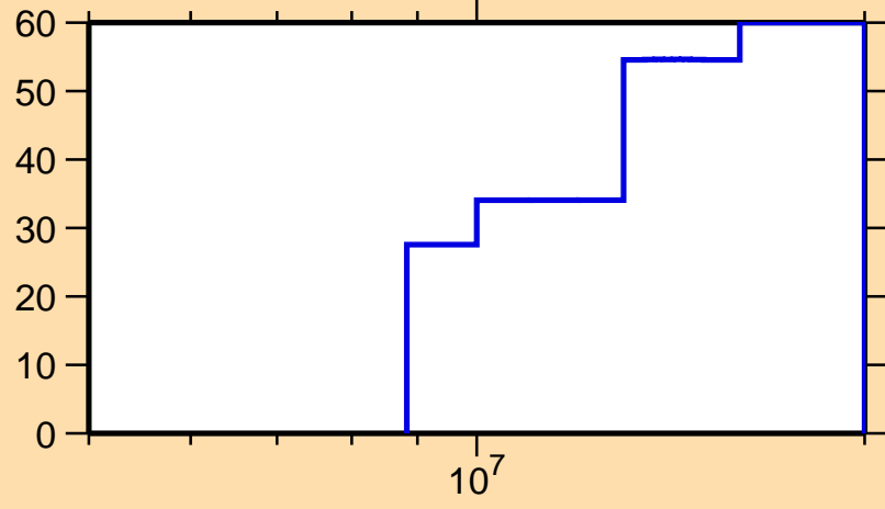
\Delta\sigma/\sigma vs. E for ^{196}\text{Pb}(n,\text{inel.})
