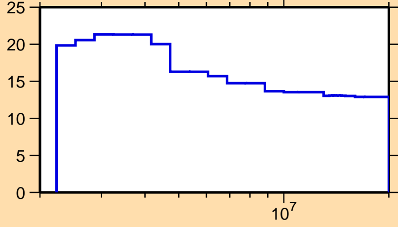
\Delta\sigma/\sigma vs. E for ^{196}\text{Pb}(n,n\text{onel.})
