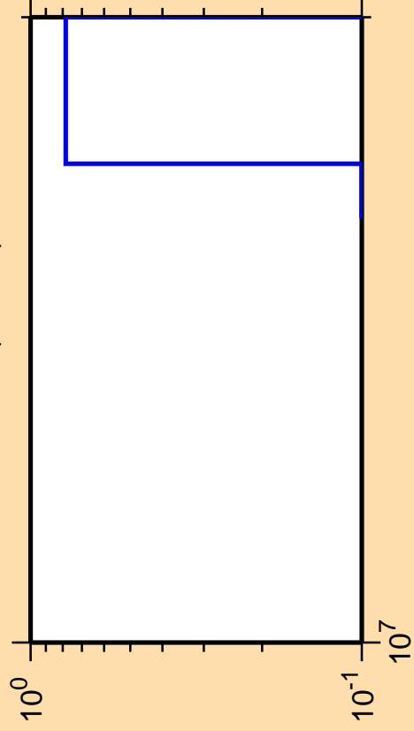
\Delta\sigma/\sigma vs. E for ^{196}\text{Pb}(\text{mt } 34)
