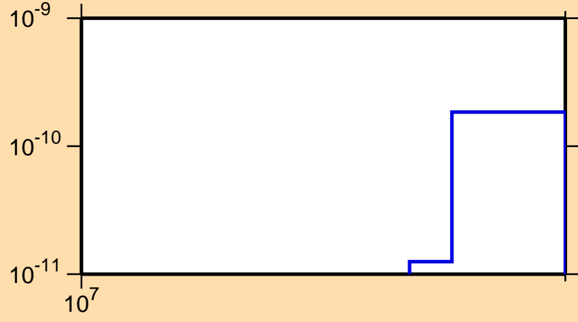
\sigma vs. E for ^{196}\text{Pb}(n,\text{pd})
