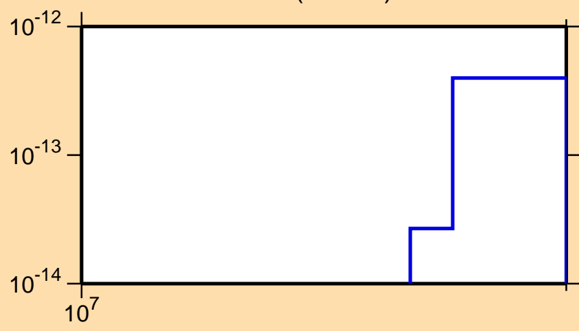
\sigma vs. E for ^{196}\text{Pb}(\text{mt117})
