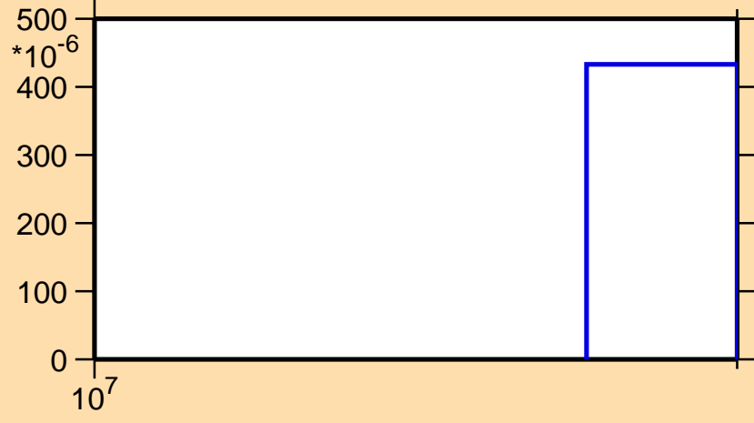
\sigma vs. E for ^{196}\text{Pb}(n,3n)
