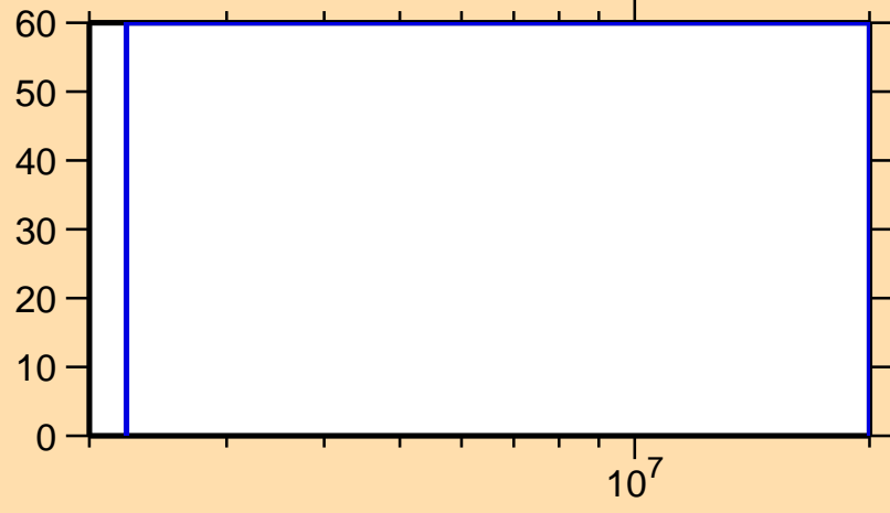
\Delta\sigma/\sigma vs. E for ^{196}\text{Pb}(n, n_1)
