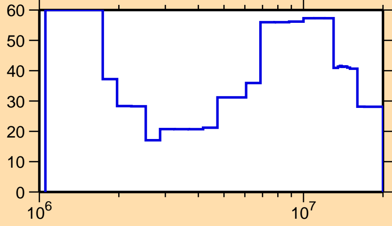
\Delta\sigma/\sigma vs. E for ^{196}\text{Pb}(n,\text{el.})
