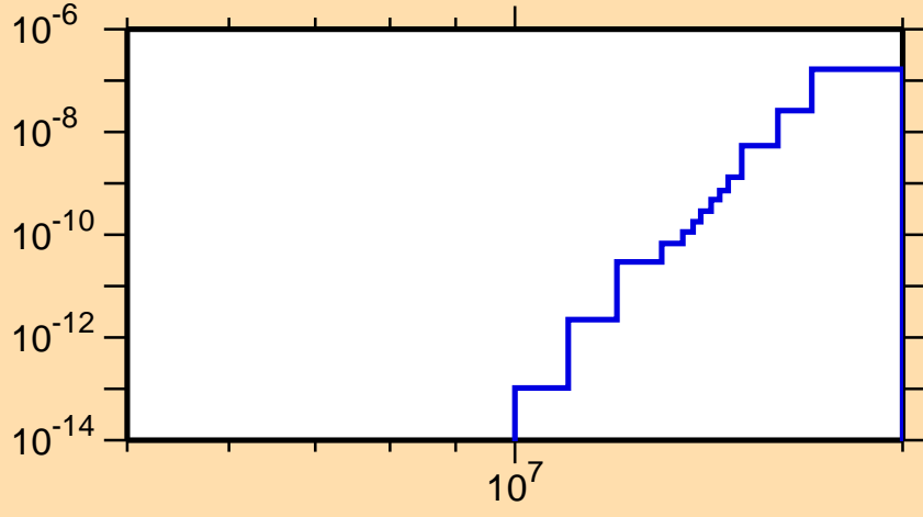
\sigma vs. E for ^{196}\text{Pb}(n,\text{He}3)
