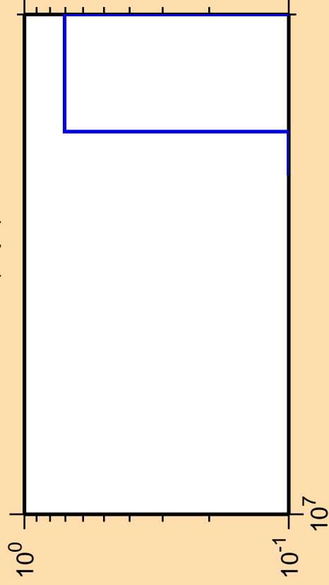
\Delta\sigma/\sigma vs. E for ^{196}\text{Pb}(n,\text{pt})
