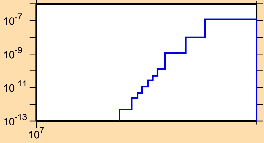
\sigma vs. E for ^{196}\text{Pb}(n,2n\alpha)
