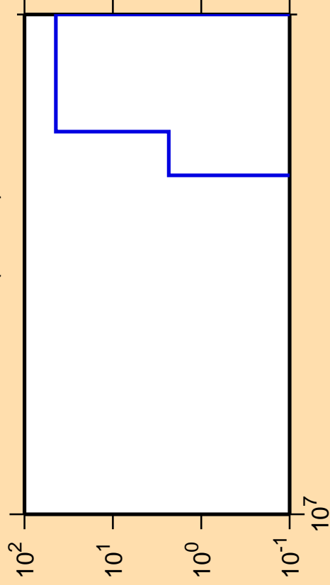
\Delta\sigma/\sigma vs. E for ^{196}\text{Pb} (mt 45)
