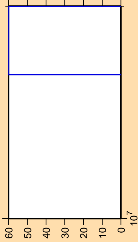
\Delta\sigma/\sigma vs. E for ^{196}\text{Pb}(n,\text{pd})
