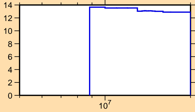
\Delta\sigma/\sigma vs. E for ^{196}\text{Pb}(n,\text{nonel.})
