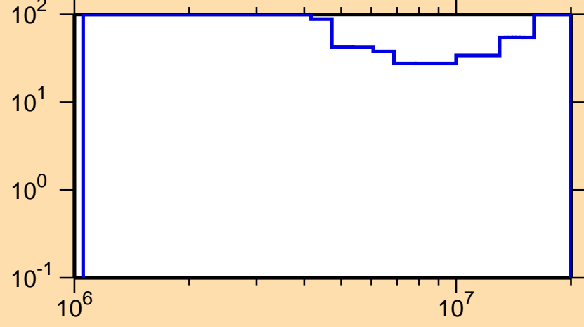
\Delta\sigma/\sigma vs. E for ^{196}\text{Pb}(n,\text{inel.})
