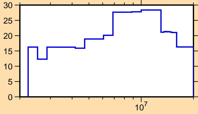
\Delta\sigma/\sigma vs. E for ^{196}\text{Pb}(n,\text{tot.})
