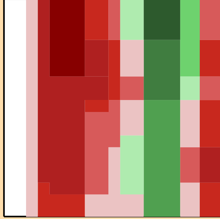
\Delta\sigma/\sigma vs. E for ^{196}\text{Pb}(n,n\text{cont.})
