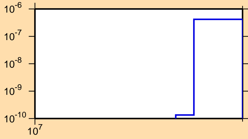
\sigma vs. E for ^{196}\text{Pb}(n,2np)
