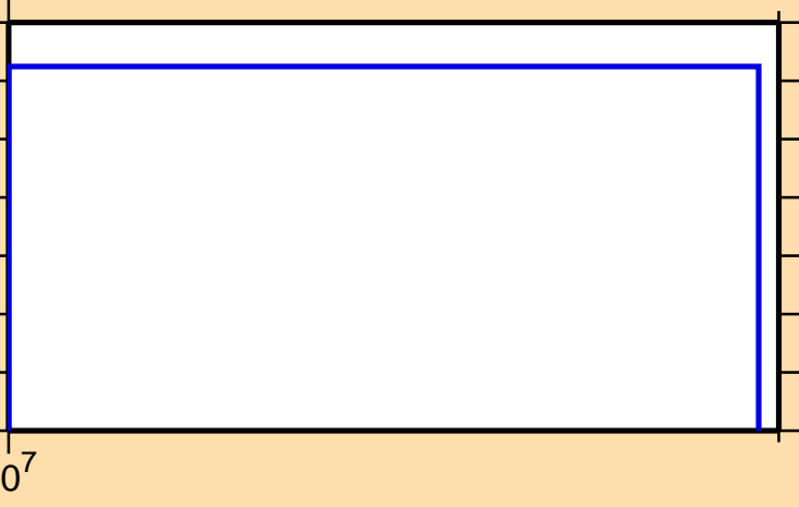
\sigma vs. E for ^{196}\text{Pb} (mt 34)
