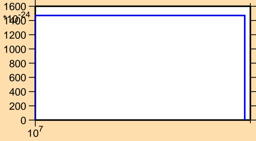
\sigma vs. E for ^{196}\text{Pb}(\text{mt 11})
