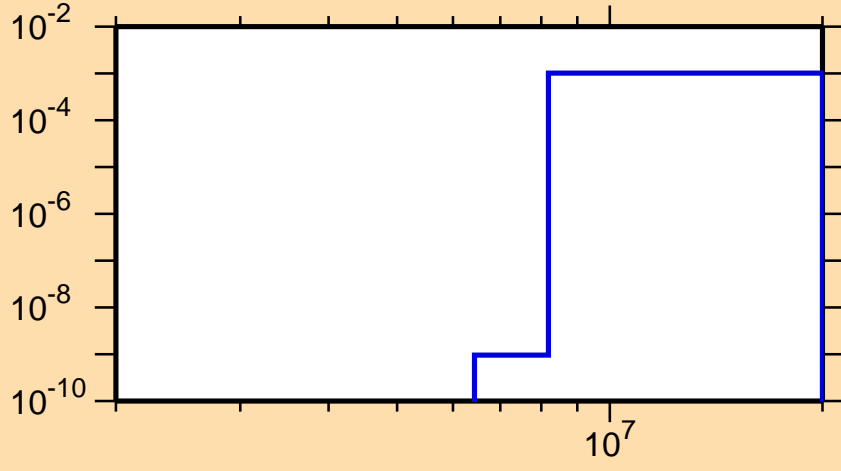
\sigma vs. E for ^{196}\text{Pb}(n,d)
