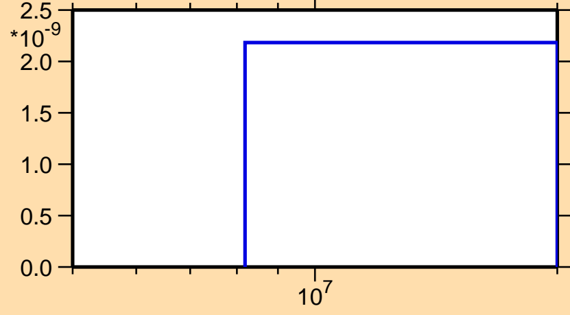
\sigma vs. E for ^{196}\text{Pb}(n,p\alpha)
