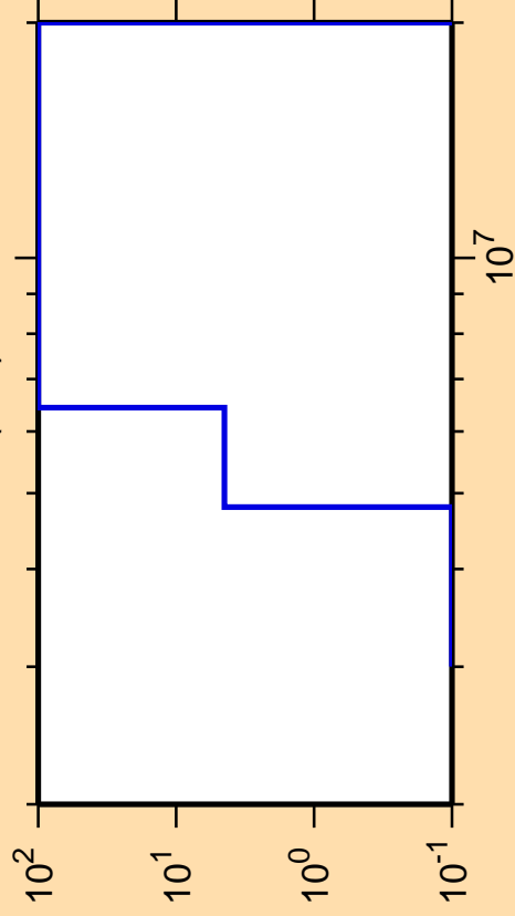
\Delta\sigma/\sigma vs. E for ^{196}\text{Pb}(n,d)
