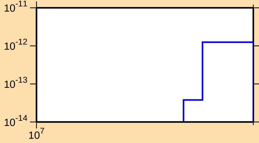
\sigma vs. E for ^{197}\text{Pb}(\text{mt } 45)
