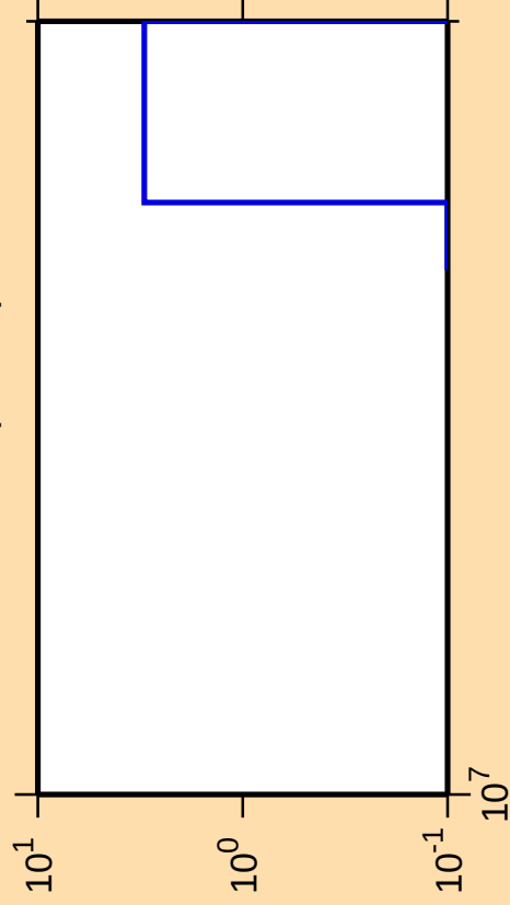
\Delta\sigma/\sigma vs. E for ^{197}\text{Pb}(\text{mt } 45)
