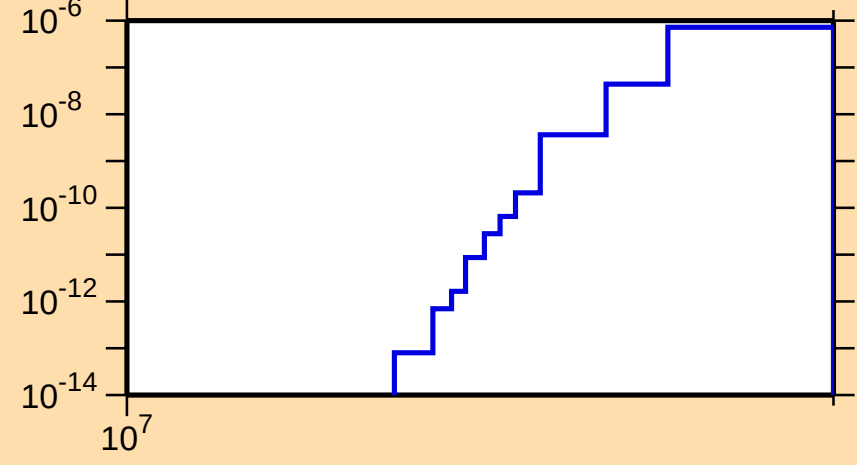
\sigma vs. E for ^{197}\text{Pb}(n,\text{nd})
