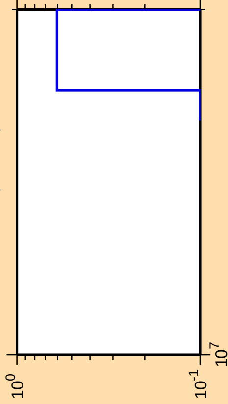
\Delta\sigma/\sigma vs. E for ^{197}\text{Pb}(\text{mt117})
