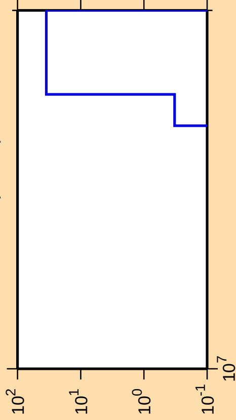
\Delta\sigma/\sigma vs. E for ^{197}\text{Pb}(\text{mt } 34)
