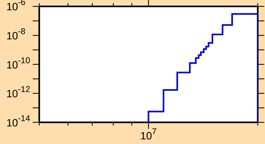
\sigma vs. E for ^{197}\text{Pb}(n,\text{He3})
