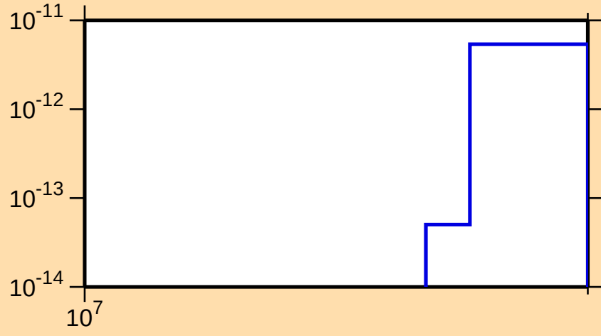
\sigma vs. E for ^{197}\text{Pb}(\text{mt } 34)
