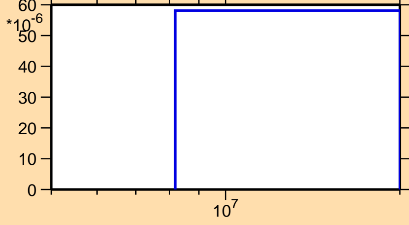
\sigma vs. E for ^{197}\text{Pb}(n,t)
