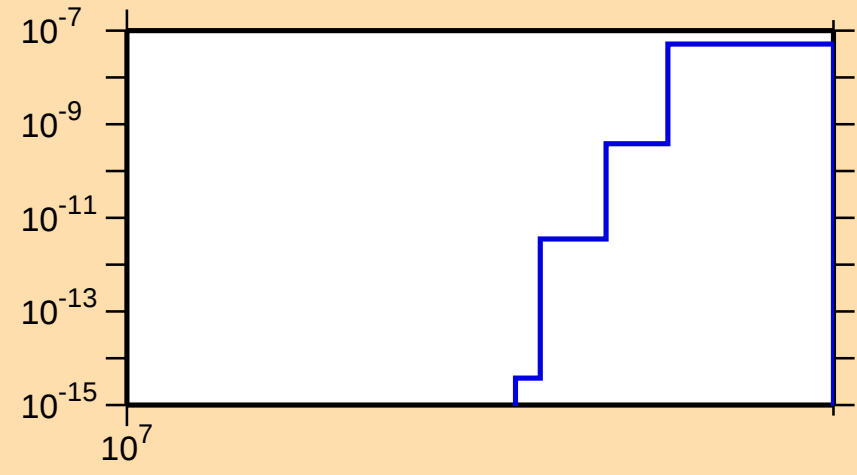
\sigma vs. E for ^{198}\text{Pb}(n,\text{nd})
