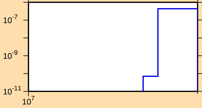
\sigma vs. E for ^{198}\text{Pb}(n,2np)
