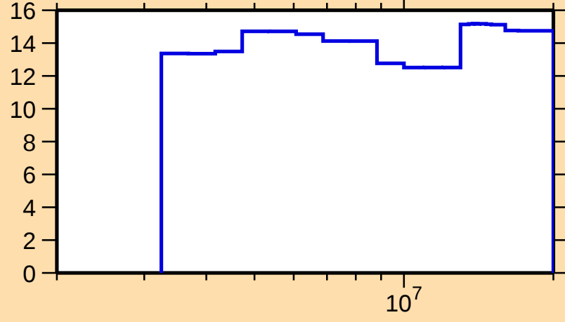
\Delta\sigma/\sigma vs. E for ^{198}\text{Pb}(n,n\text{onel.})
