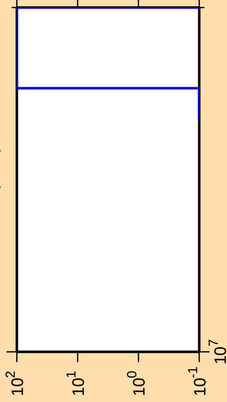
\Delta\sigma/\sigma vs. E for ^{198}\text{Pb}(n,nt)
