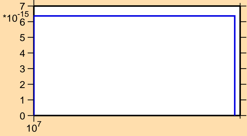
\sigma vs. E for ^{198}\text{Pb} (mt 45)
