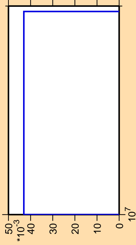
\Delta\sigma/\sigma vs. E for ^{198}\text{Pb} (mt 45)
