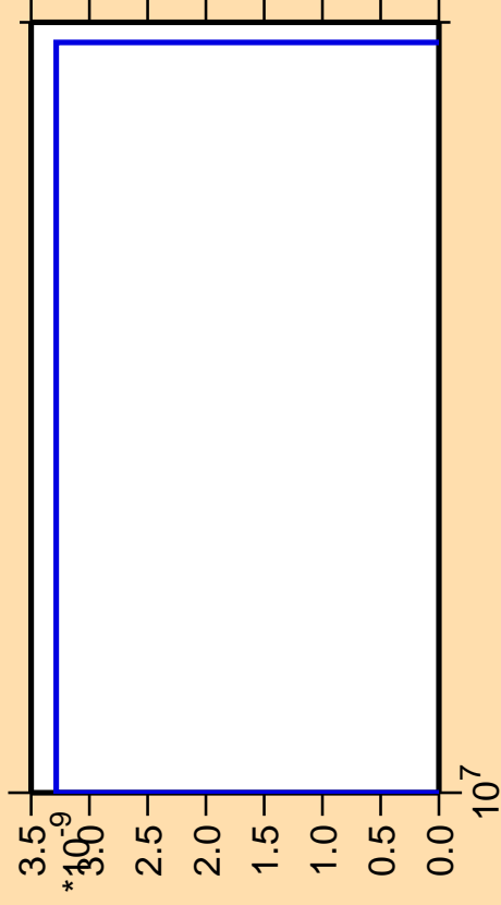
\Delta\sigma/\sigma vs. E for ^{198}\text{Pb} (mt 11)
