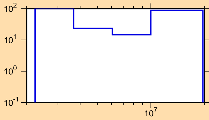
\Delta\sigma/\sigma vs. E for ^{198}\text{Pb}(n,n\text{cont.})
