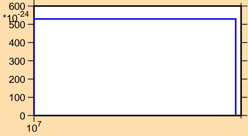
\sigma vs. E for ^{198}\text{Pb} (mt 11)
