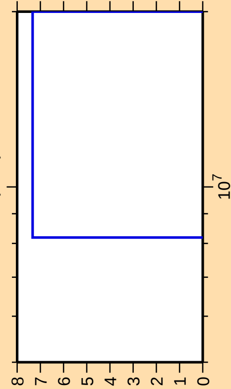
\Delta\sigma/\sigma vs. E for ^{198}\text{Pb}(n,nt)
