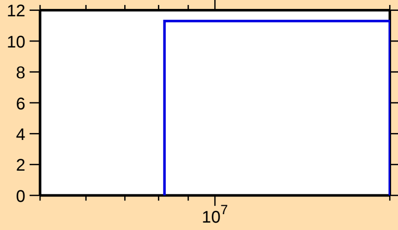
\Delta\sigma/\sigma vs. E for ^{198}\text{Pb}(n,\text{tot.})
