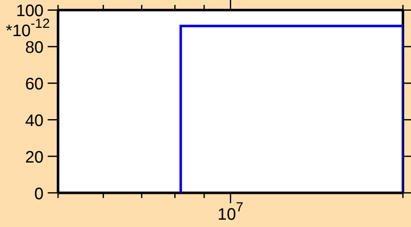
\sigma vs. E for ^{198}\text{Pb}(n,p\alpha)
