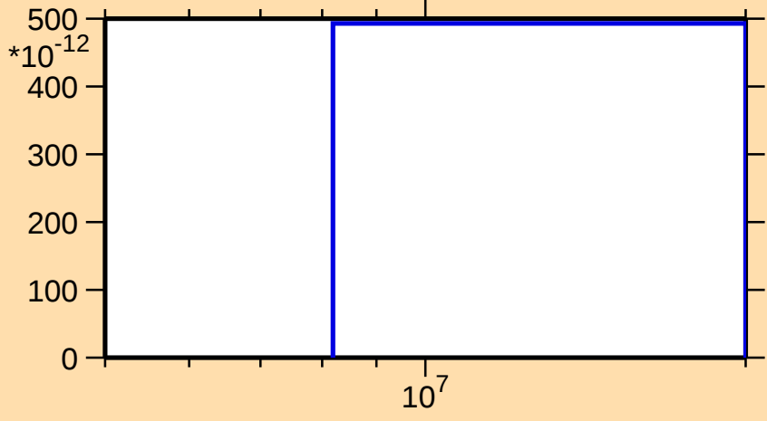
\sigma vs. E for ^{198}\text{Pb}(n,\text{He}3)
