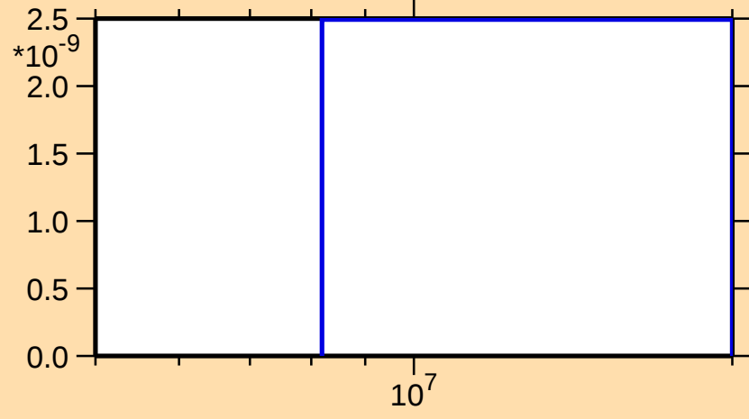
\sigma vs. E for ^{198}\text{Pb}(n,2n\alpha)
