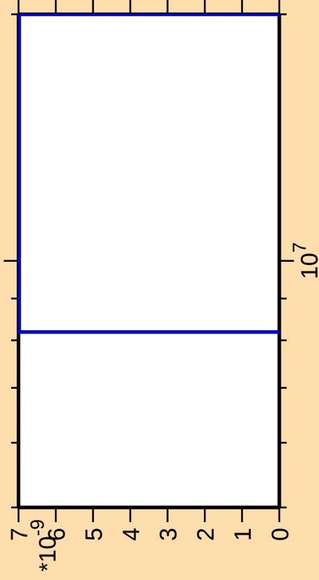
\Delta\sigma/\sigma vs. E for ^{198}\text{Pb}(\text{mt } 11)
