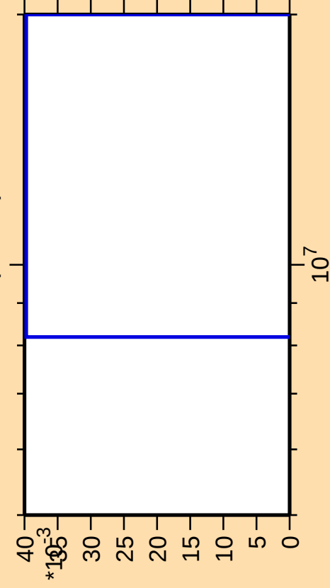
\Delta\sigma/\sigma vs. E for ^{198}\text{Pb}(\text{mt } 45)
