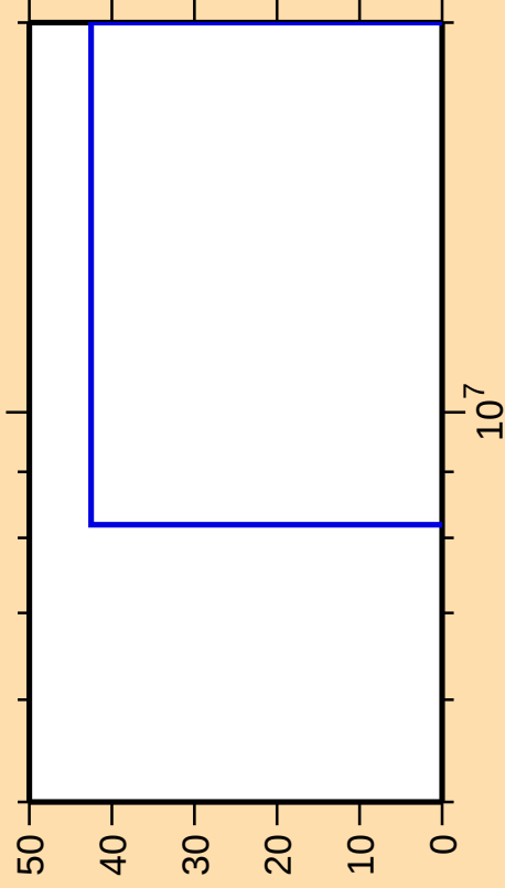
\Delta\sigma/\sigma vs. E for ^{198}\text{Pb}(n,2n)
