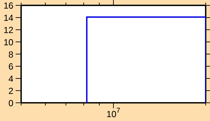
\Delta\sigma/\sigma vs. E for ^{198}\text{Pb}(n,\text{nonel.})
