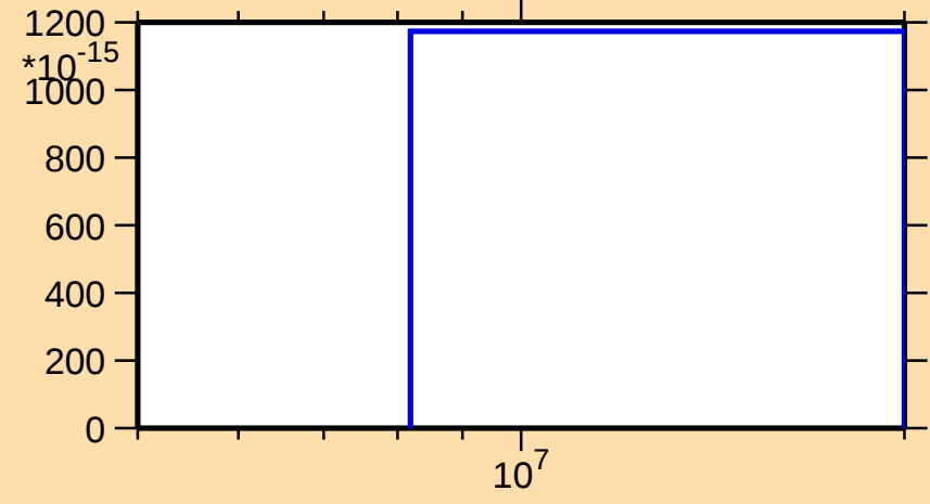
\sigma vs. E for ^{198}\text{Pb}(n,nt)
