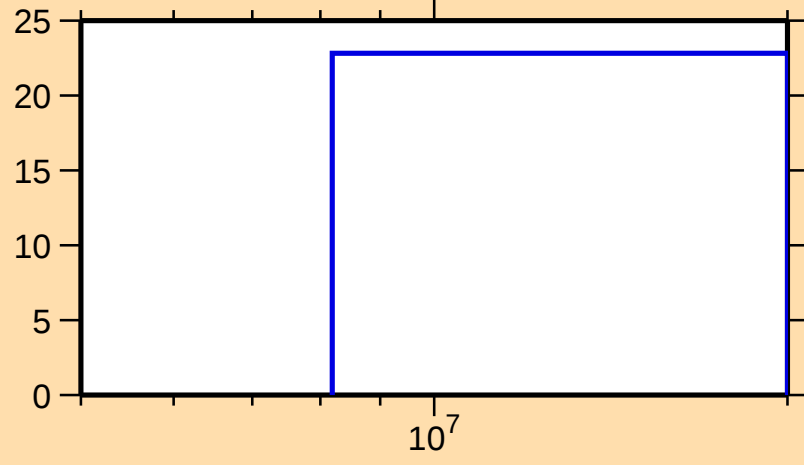
\Delta\sigma/\sigma vs. E for ^{198}\text{Pb}(n,\text{el.})
