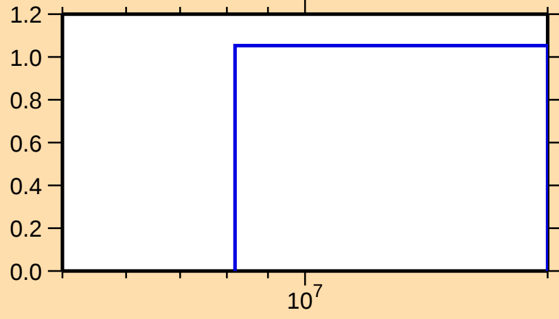
\sigma vs. E for ^{198}\text{Pb}(n,2n)
