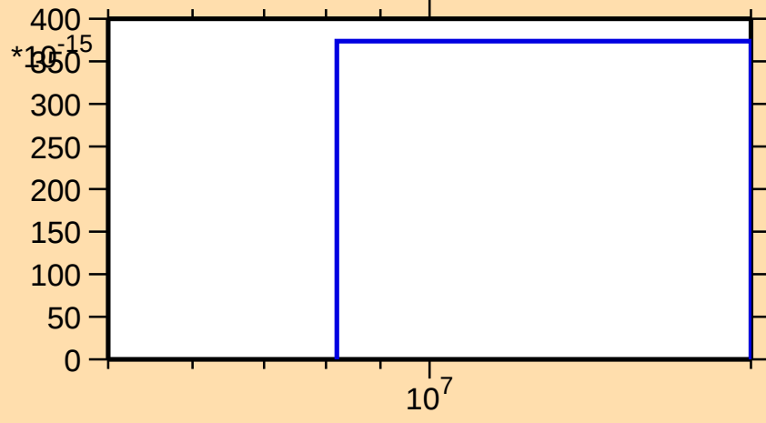
\sigma vs. E for ^{198}\text{Pb}(n,\text{pd})
