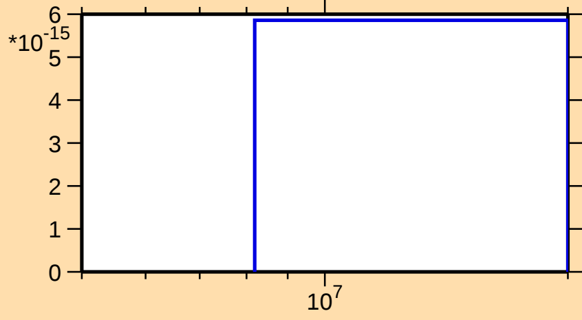
\sigma vs. E for ^{198}\text{Pb}(\text{mt } 45)
