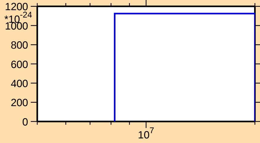
\sigma vs. E for ^{198}\text{Pb}(\text{mt } 11)
