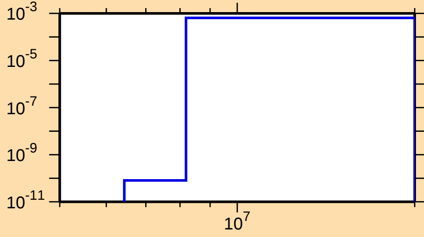
\sigma vs. E for ^{198}\text{Pb}(n,d)
