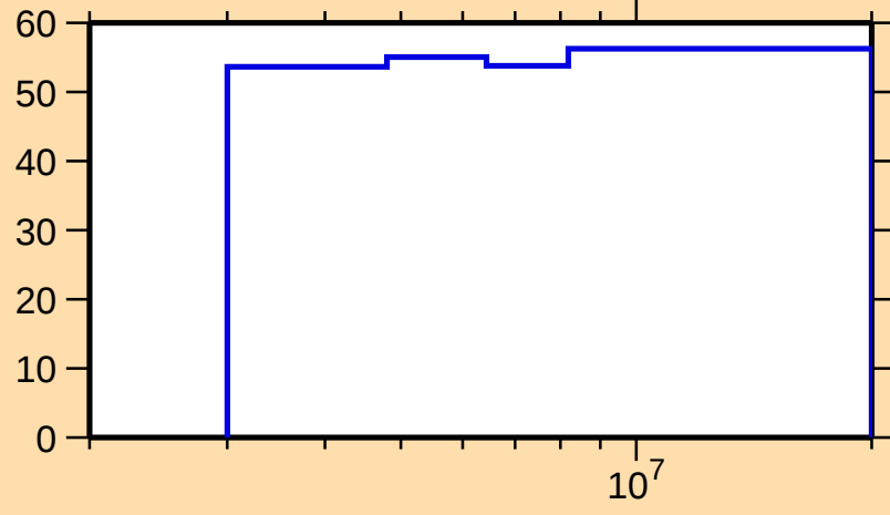
\Delta\sigma/\sigma vs. E for ^{198}\text{Pb}(n, n_1)
