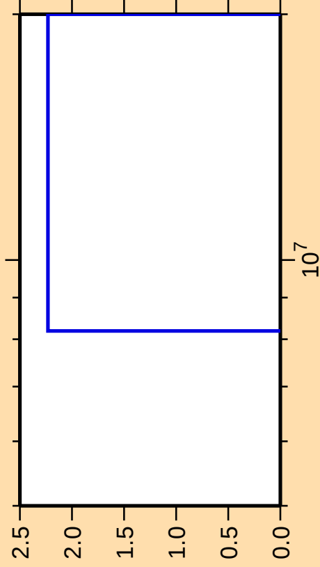
\Delta\sigma/\sigma vs. E for ^{198}\text{Pb}(n,\text{pd})
