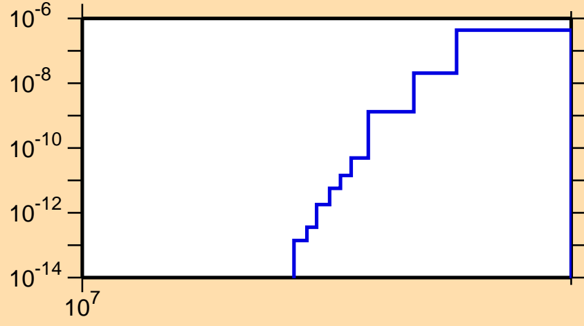
\sigma vs. E for ^{199}\text{Pb}(n,\text{nd})
