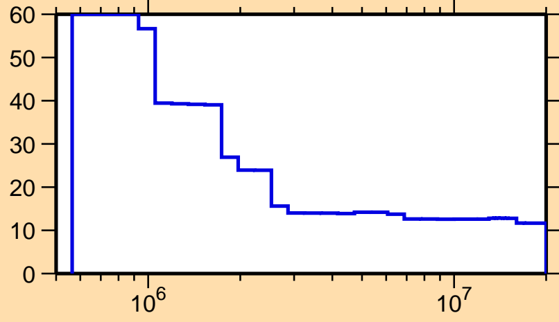
\Delta\sigma/\sigma vs. E for ^{199}\text{Pb}(n,n\text{nonel.})
