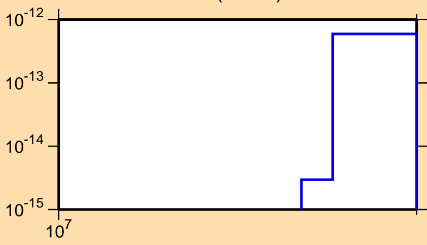
\sigma vs. E for ^{199}\text{Pb} (mt 34)
