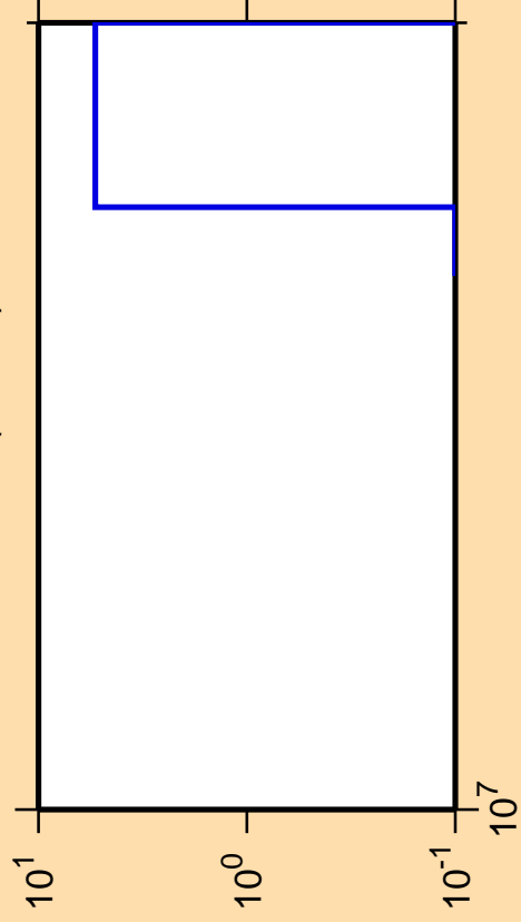
\Delta\sigma/\sigma vs. E for ^{199}\text{Pb} (mt 34)
