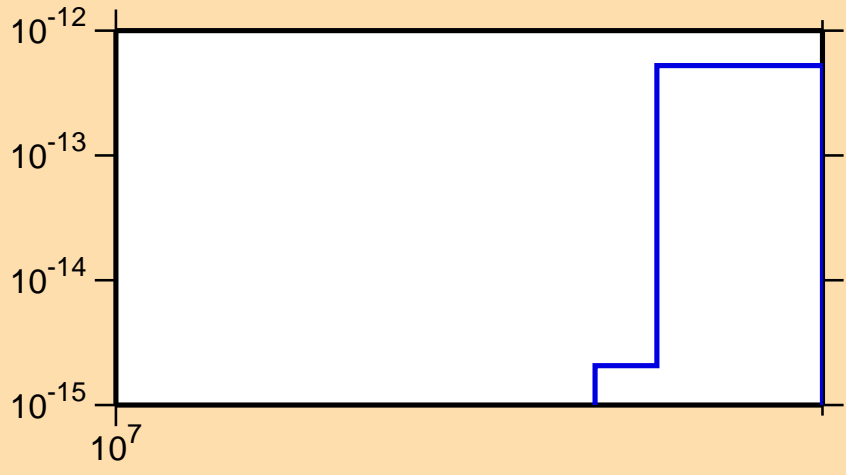
\sigma vs. E for ^{199}\text{Pb}(n,\text{pt})
