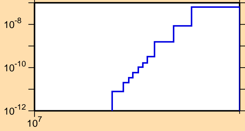
\sigma vs. E for ^{199}\text{Pb}(n,\text{He3})
