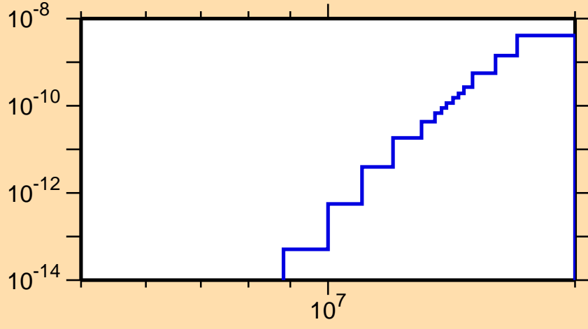
\sigma vs. E for ^{199}\text{Pb}(n,p\alpha)
