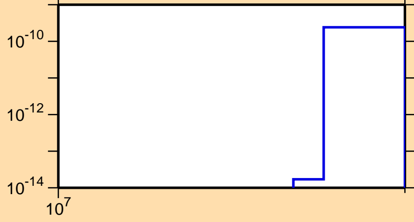
\sigma vs. E for ^{199}\text{Pb}(n,nt)
