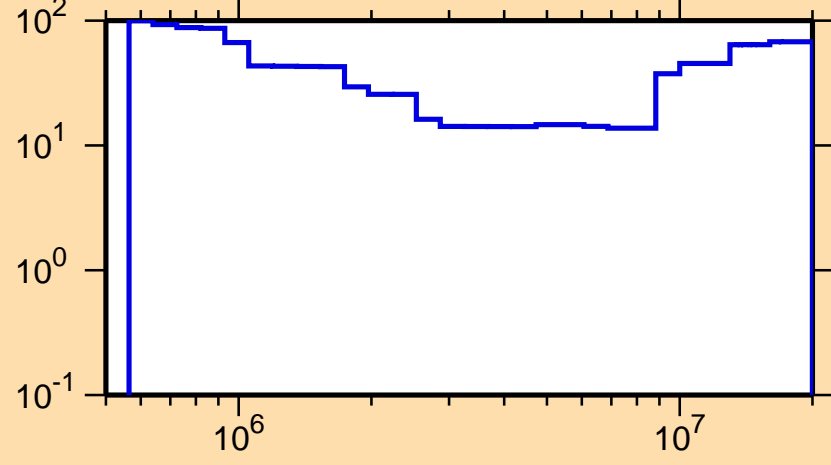
\Delta\sigma/\sigma vs. E for ^{199}\text{Pb}(n,n\text{cont.})
