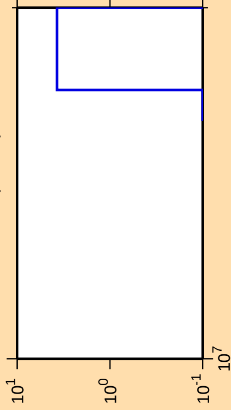
\Delta\sigma/\sigma vs. E for ^{199}\text{Pb}(\text{mt } 34)
