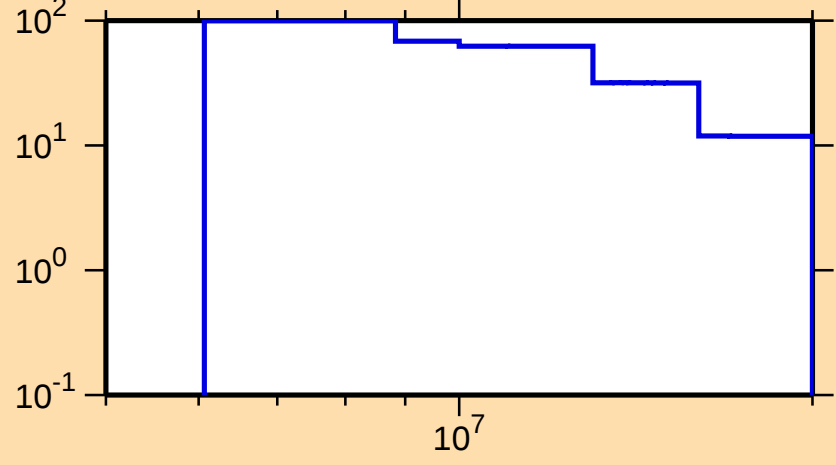
\Delta\sigma/\sigma vs. E for ^{199}\text{Pb}(n,2n)
