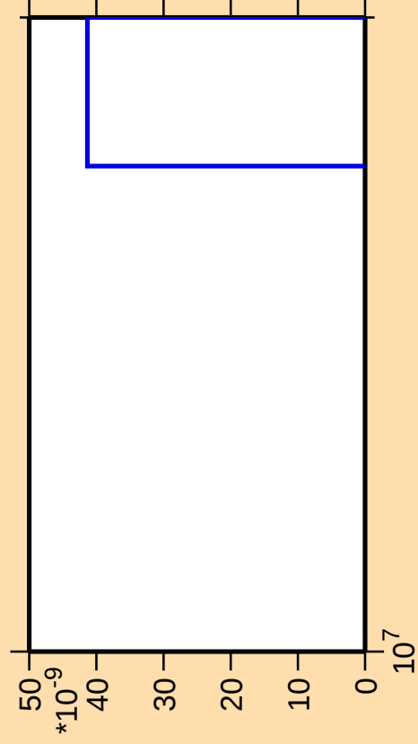
\Delta\sigma/\sigma vs. E for ^{199}\text{Pb}(\text{mt } 11)
