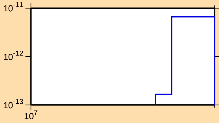
\sigma vs. E for ^{199}\text{Pb}(n,\text{pd})
