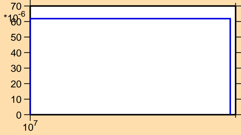
\sigma vs. E for ^{199}\text{Pb}(n,3n)
