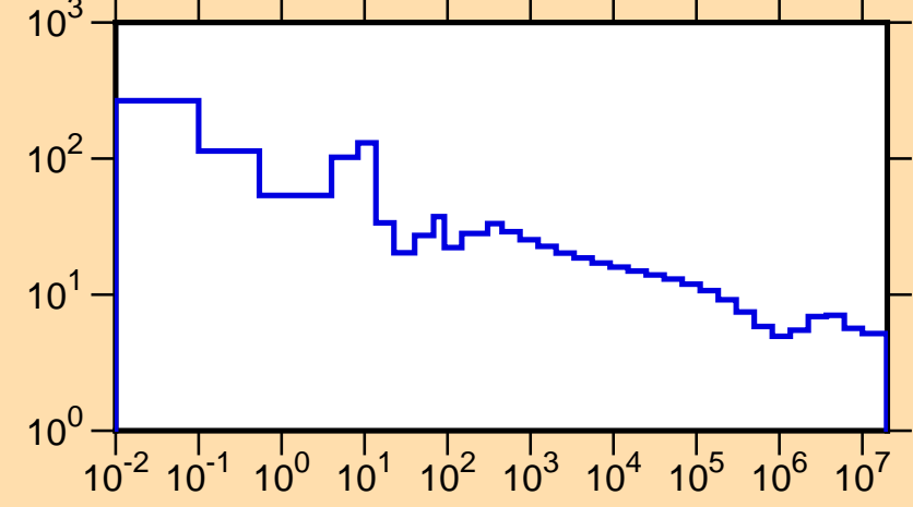
\sigma vs. E for ^{199}\text{Pb}(n,\text{tot.})
