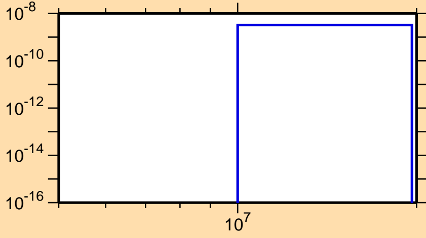
\sigma vs. E for ^{199}\text{Pb}(n,\text{He3})
