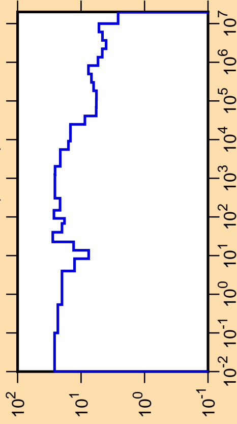
\Delta\sigma/\sigma vs. E for ^{199}\text{Pb}(n,\text{tot.})
