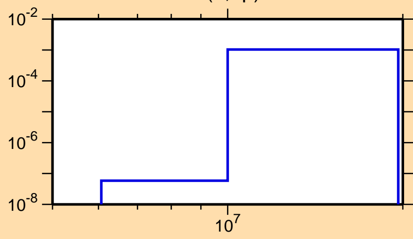
\sigma vs. E for ^{199}\text{Pb}(n,np)
