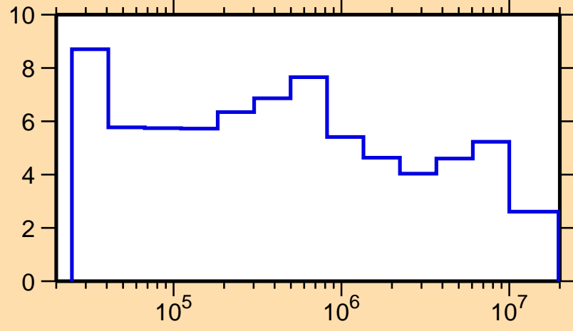
\Delta\sigma/\sigma vs. E for ^{199}\text{Pb}(n,\text{tot.})
