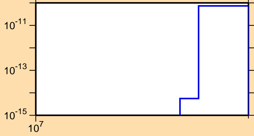
\sigma vs. E for ^{200}\text{Pb}(n,nt)
