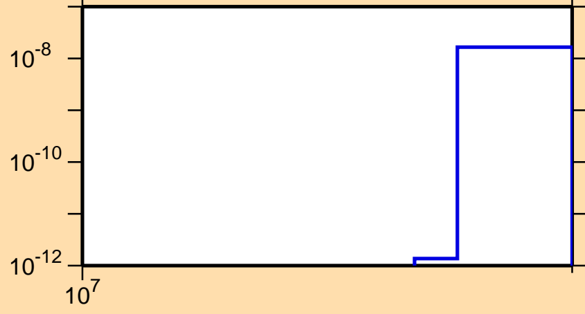
\sigma vs. E for ^{200}\text{Pb}(n,2np)
