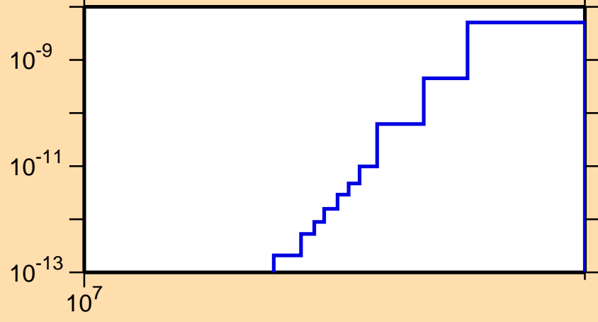
\sigma vs. E for ^{200}\text{Pb}(n,\text{He3})
