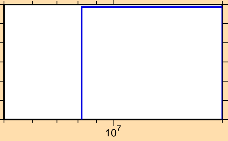
\sigma vs. E for ^{200}\text{Pb}(n,3n)
