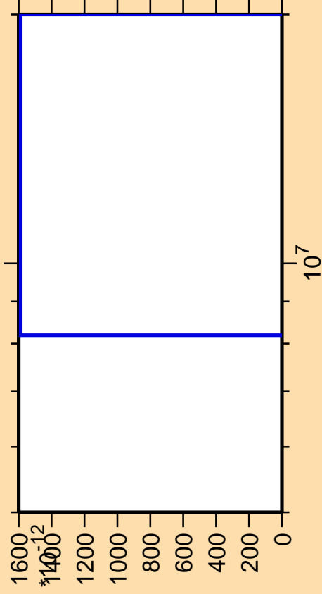
\Delta\sigma/\sigma vs. E for ^{200}\text{Pb}(\text{mt } 11)
