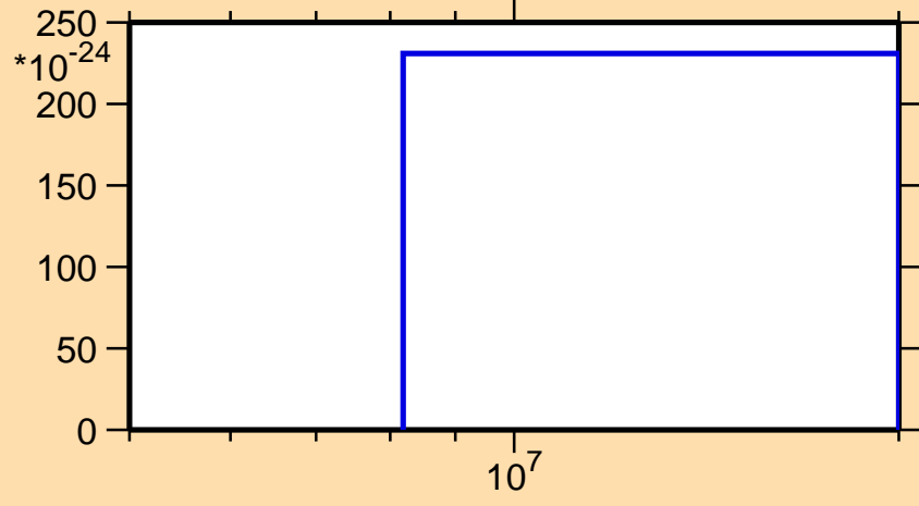
\sigma vs. E for ^{200}\text{Pb}(\text{mt } 11)
