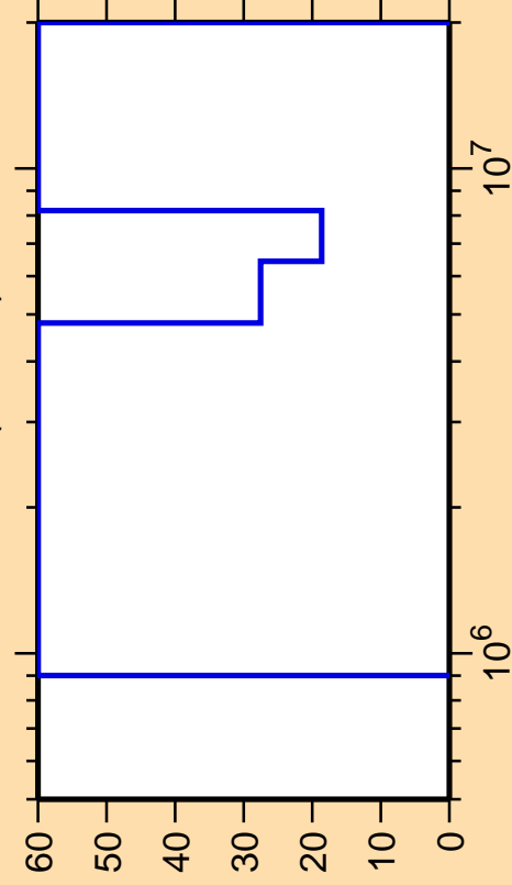
\Delta\sigma/\sigma vs. E for ^{200}\text{Pb}(n,\text{inel.})
