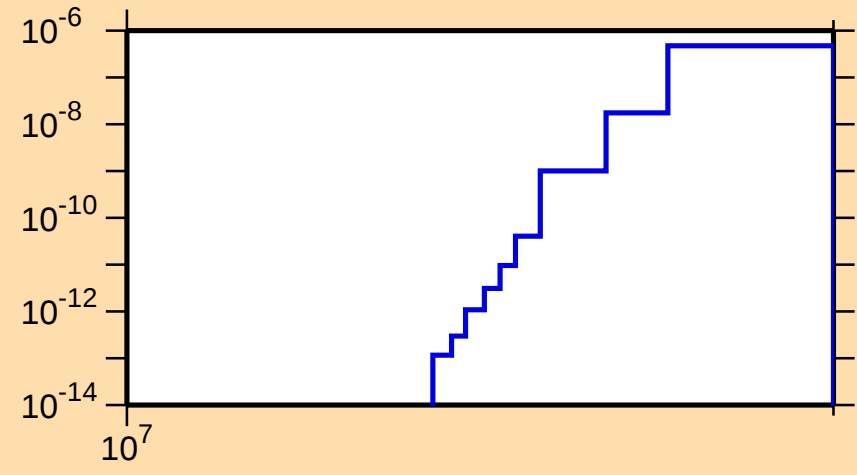
\sigma vs. E for ^{203}\text{Pb}(n,\text{nd})
