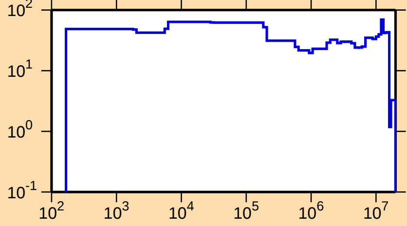
\Delta\sigma/\sigma vs. E for ^{203}\text{Pb}(n,n_1)
