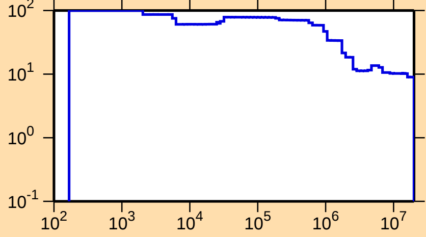
\Delta\sigma/\sigma vs. E for ^{203}\text{Pb}(n,\text{nonel.})
