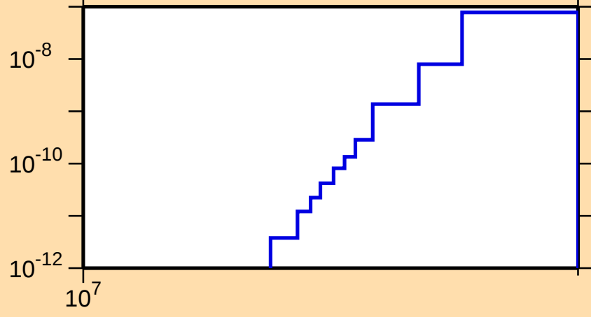
\sigma vs. E for ^{203}\text{Pb}(n,2n\alpha)
