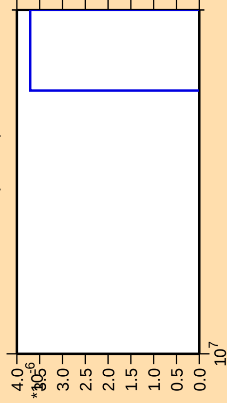
\Delta\sigma/\sigma vs. E for ^{203}\text{Pb}(\text{mt 11})
