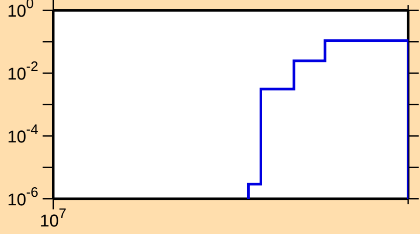
\sigma vs. E for ^{203}\text{Pb}(n,3n)
