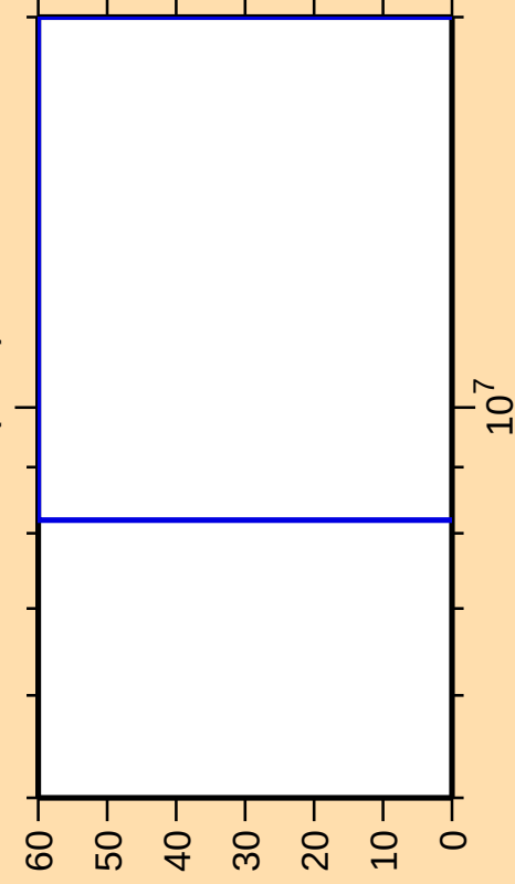
\Delta\sigma/\sigma vs. E for ^{203}\text{Pb}(n,\text{nt})
