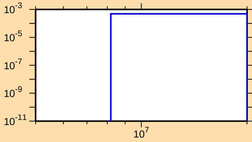
\sigma vs. E for ^{203}\text{Pb}(n,np)
