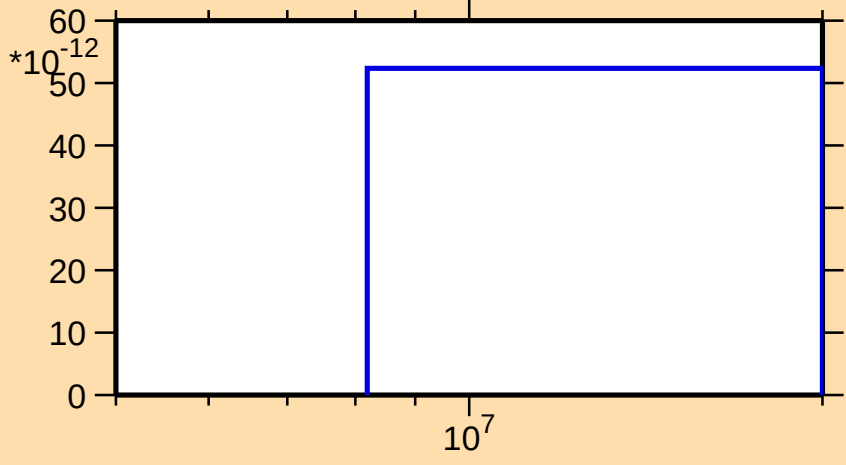
\sigma vs. E for ^{203}\text{Pb}(n,\text{He3})
