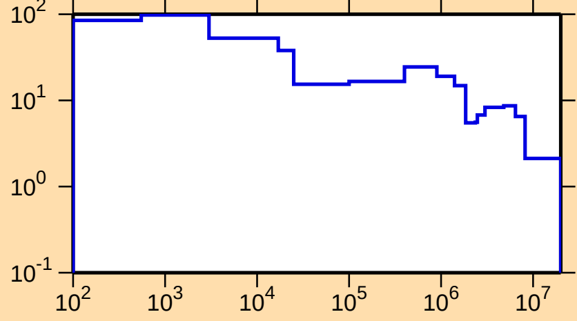
\Delta\sigma/\sigma vs. E for ^{203}\text{Pb}(n,\text{tot.})
