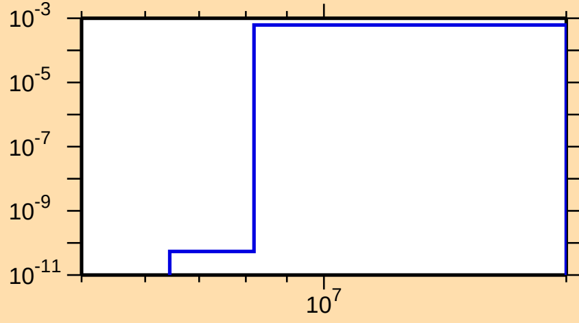
\sigma vs. E for ^{203}\text{Pb}(n,d)
