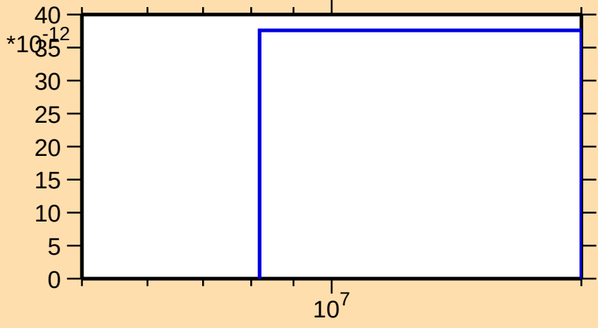
\sigma vs. E for ^{203}\text{Pb}(n,\text{nt})
