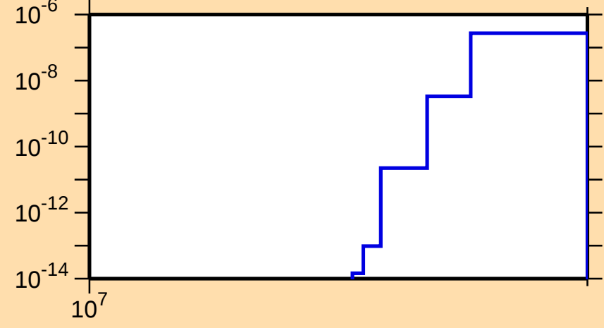
\sigma vs. E for ^{212}\text{Pb}(n,\text{nd})
