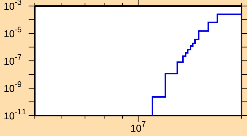
\sigma vs. E for ^{212}\text{Pb}(n,d)
