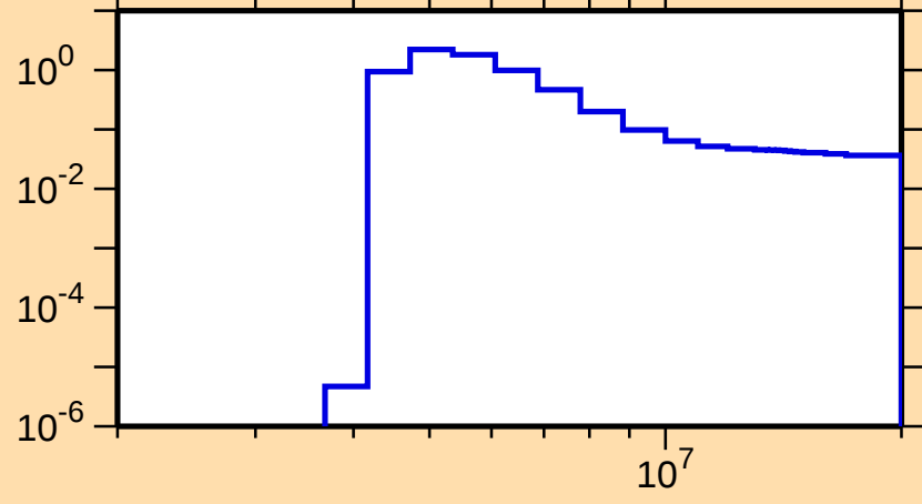
\sigma vs. E for ^{212}\text{Pb}(n,n\text{cont.})
