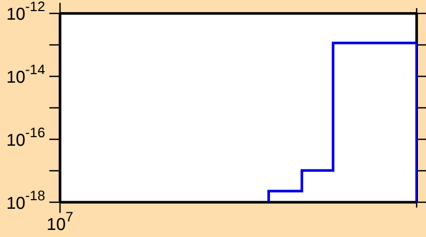
\sigma vs. E for ^{212}\text{Pb} (mt 11)
