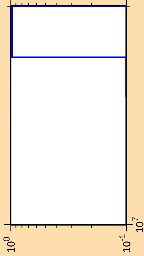
\Delta\sigma/\sigma vs. E for ^{212}\text{Pb} (mt 11)
