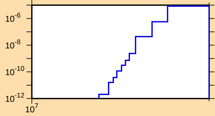
\sigma vs. E for ^{212}\text{Pb}(n,nt)
