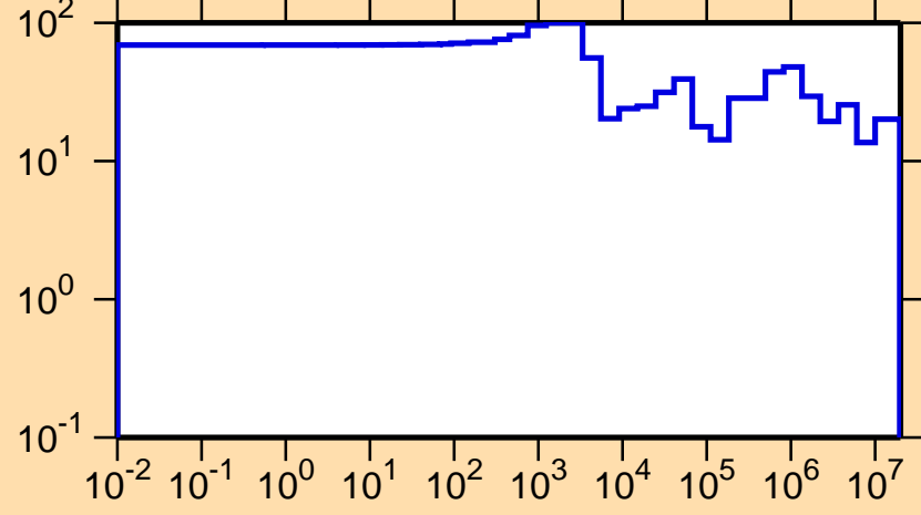
\Delta\sigma/\sigma vs. E for ^{212}\text{Pb}(n,\text{el.})
