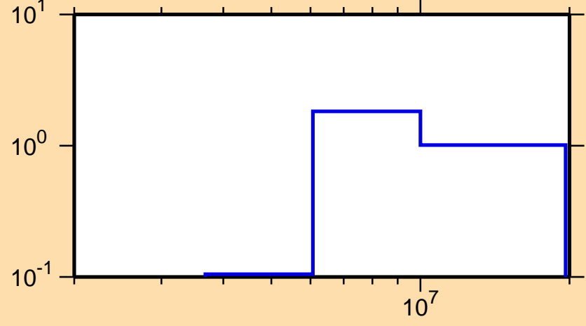
\sigma vs. E for ^{212}\text{Pb}(n,2n)
