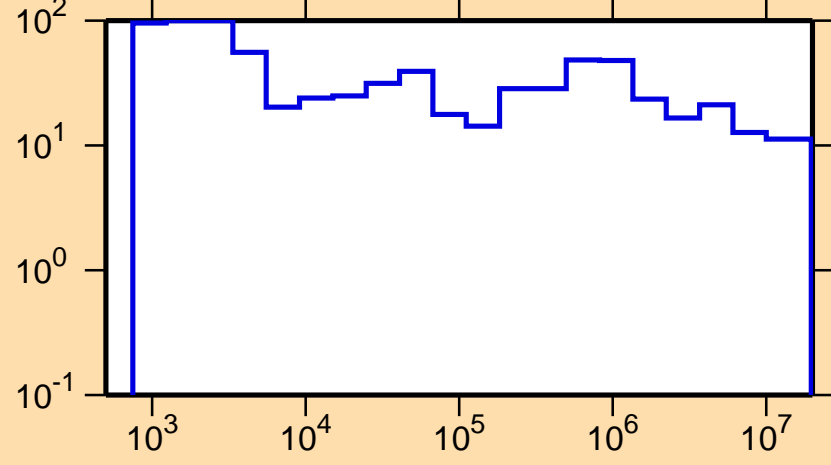
\Delta\sigma/\sigma vs. E for ^{212}\text{Pb}(n,\text{tot.})
