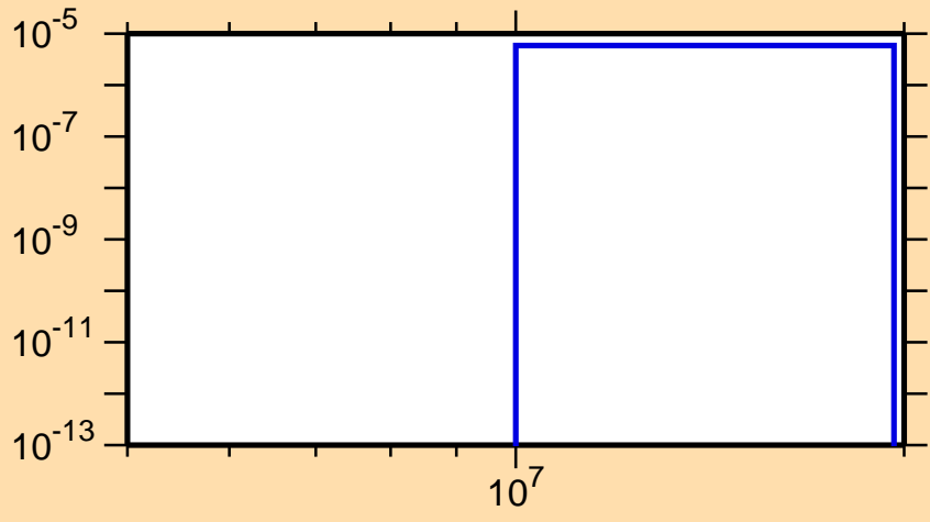
\sigma vs. E for ^{212}\text{Pb}(n,np)
