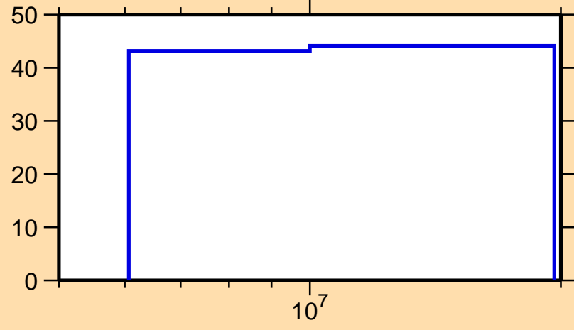
\Delta\sigma/\sigma vs. E for ^{212}\text{Pb}(n,ncont.)
