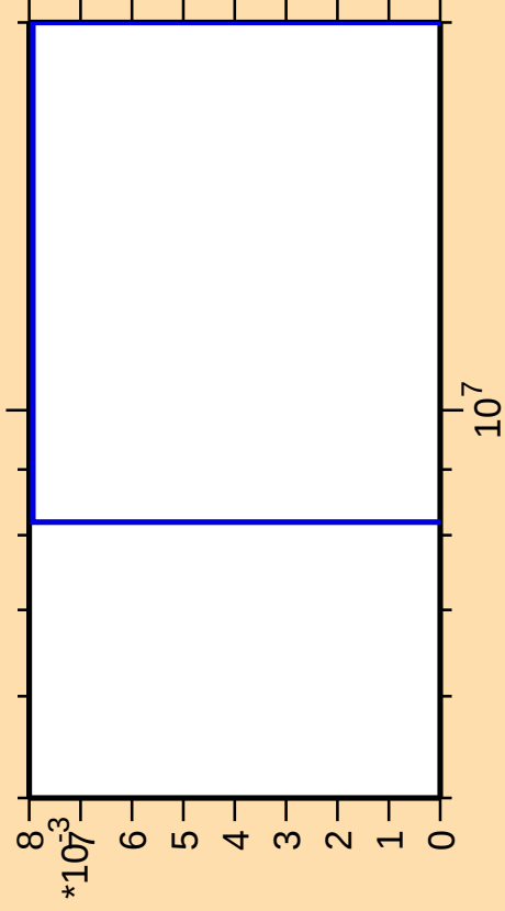
\Delta\sigma/\sigma vs. E for ^{212}\text{Pb}(\text{mt } 11)
