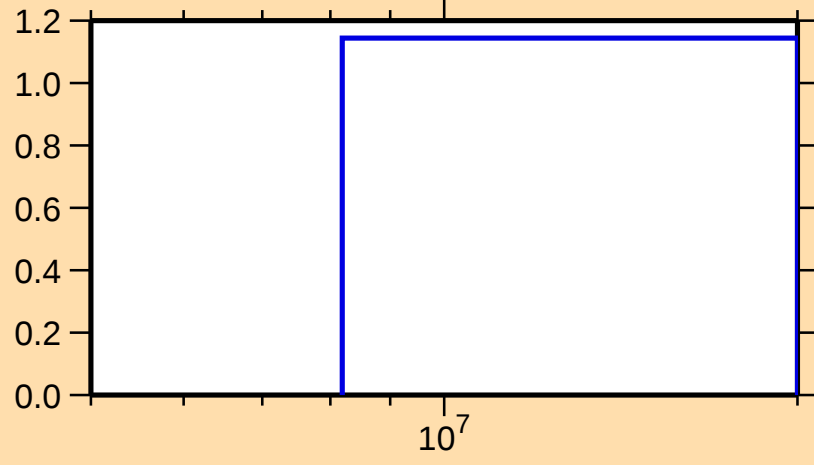
\sigma vs. E for ^{212}\text{Pb}(n,3n)
