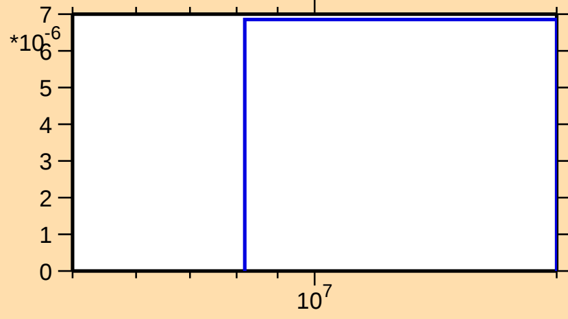
\sigma vs. E for ^{212}\text{Pb}(n,d)
