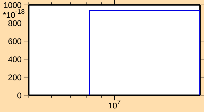
\sigma vs. E for ^{212}\text{Pb}(\text{mt } 11)
