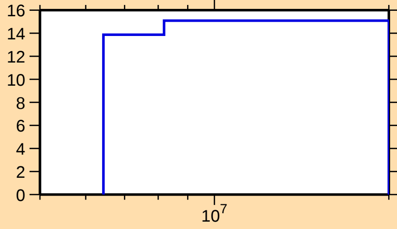
\Delta\sigma/\sigma vs. E for ^{212}\text{Pb}(n,\text{nonel.})
