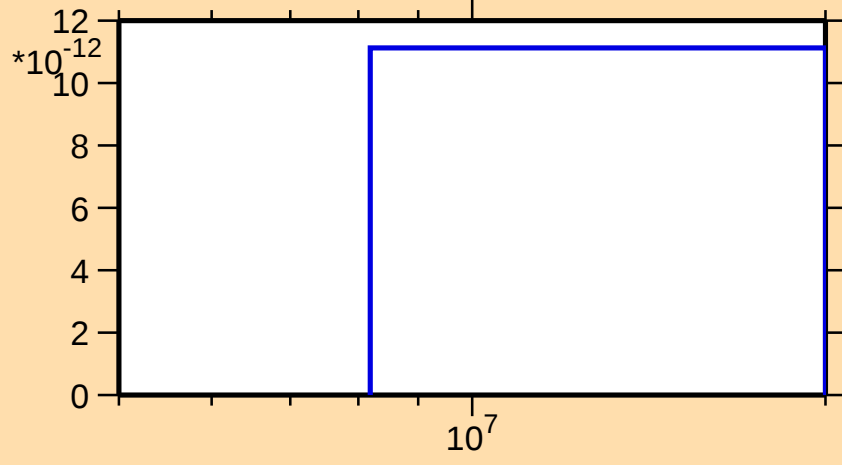
\sigma vs. E for ^{212}\text{Pb}(n,3n\alpha)
