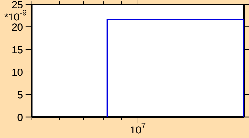
\sigma vs. E for ^{212}\text{Pb}(n,2n\alpha)
