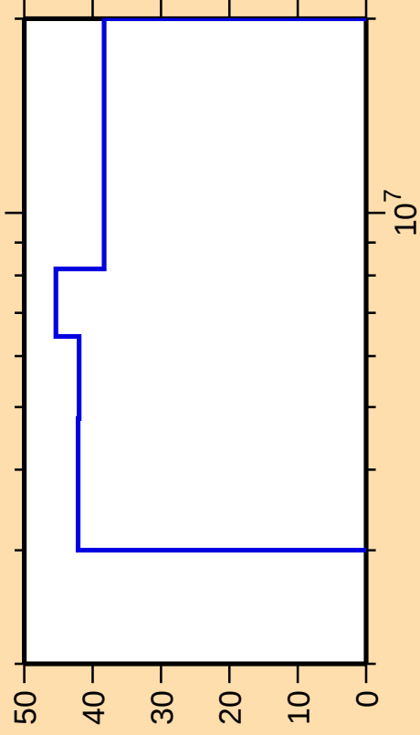
\Delta\sigma/\sigma vs. E for ^{212}\text{Pb}(n,\text{ncont.})
