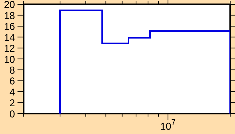
\Delta\sigma/\sigma vs. E for ^{212}\text{Pb}(n,n\text{nonel.})
