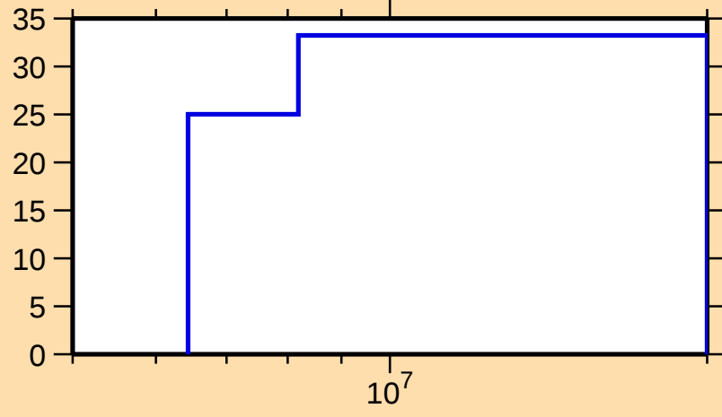
\Delta\sigma/\sigma vs. E for ^{212}\text{Pb}(n,n_1)
