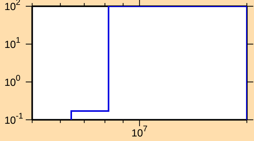
\Delta\sigma/\sigma vs. E for ^{212}\text{Pb}(n,p)
