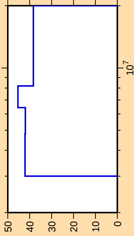
\Delta\sigma/\sigma vs. E for ^{212}\text{Pb}(n,n\text{cont.})
