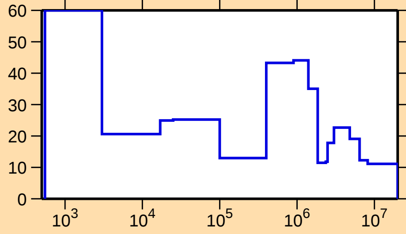
\Delta\sigma/\sigma vs. E for ^{212}\text{Pb}(n,\text{tot.})
