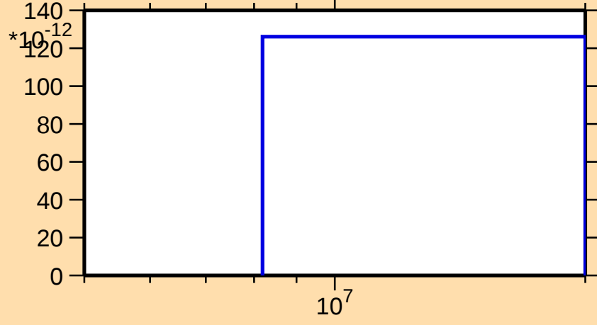
\sigma vs. E for ^{212}\text{Pb}(n,2np)
