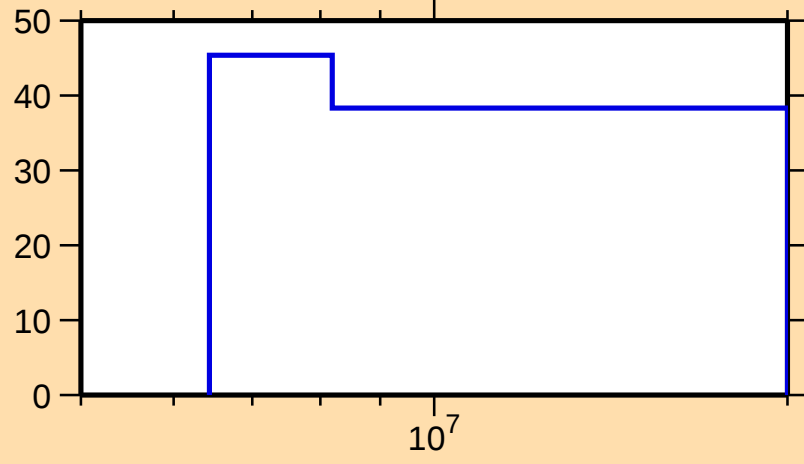
\Delta\sigma/\sigma vs. E for ^{212}\text{Pb}(n,n\text{cont.})
