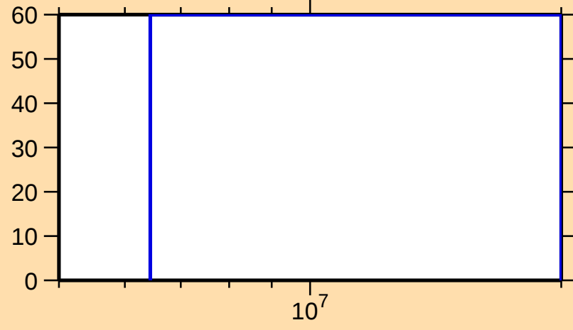
\Delta\sigma/\sigma vs. E for ^{212}\text{Pb}(n,\gamma)
