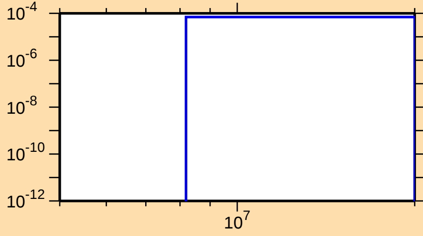
\sigma vs. E for ^{212}\text{Pb}(n,p)
