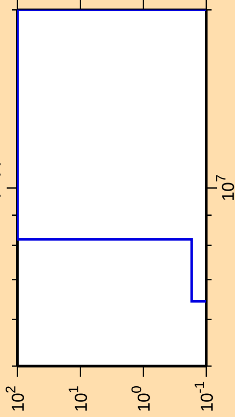
\Delta\sigma/\sigma vs. E for ^{212}\text{Pb}(n,p)
