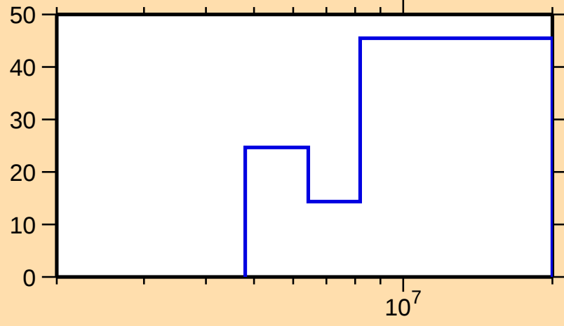
\Delta\sigma/\sigma vs. E for ^{212}\text{Pb}(n,2n)
