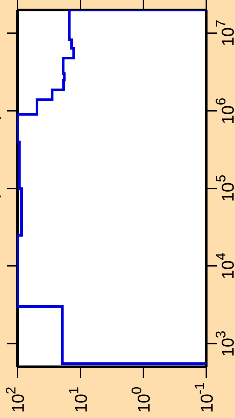
\Delta\sigma/\sigma vs. E for ^{212}\text{Pb}(n,\text{nonel.})
