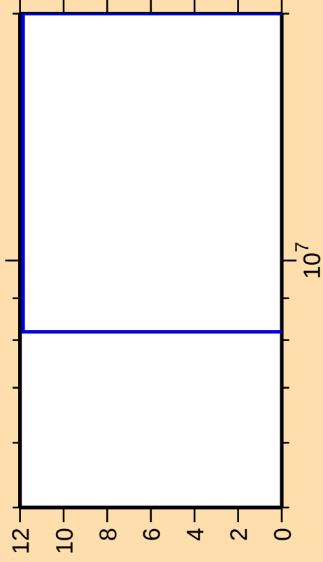
\Delta\sigma/\sigma vs. E for ^{212}\text{Pb}(n,3n)
