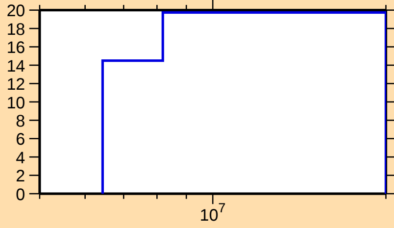
\Delta\sigma/\sigma vs. E for ^{212}\text{Pb}(n,\text{el.})
