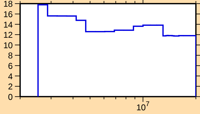
\Delta\sigma/\sigma vs. E for ^{213}\text{Pb}(n,\text{nonel.})
