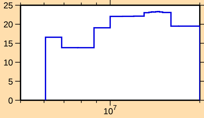
\Delta\sigma/\sigma vs. E for ^{213}\text{Pb}(n,2n)
