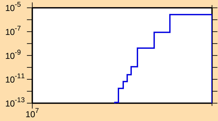
\sigma vs. E for ^{213}\text{Pb}(n,\text{nd})
