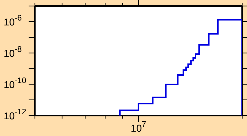
\sigma vs. E for ^{213}\text{Pb}(n,2n\alpha)
