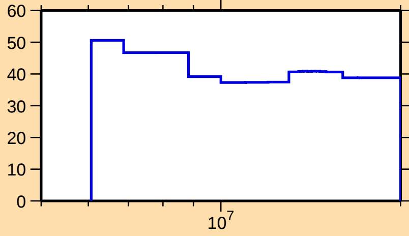
\Delta\sigma/\sigma vs. E for ^{213}\text{Pb}(n,n_1)
