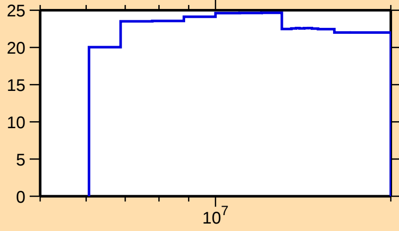
\Delta\sigma/\sigma vs. E for ^{213}\text{Pb}(n,n\text{cont.})
