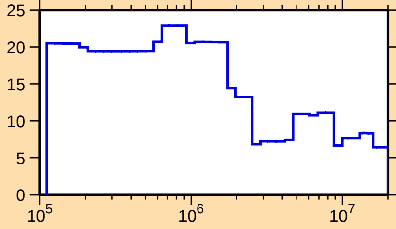
\Delta\sigma/\sigma vs. E for ^{213}\text{Pb}(n,\text{el.})
