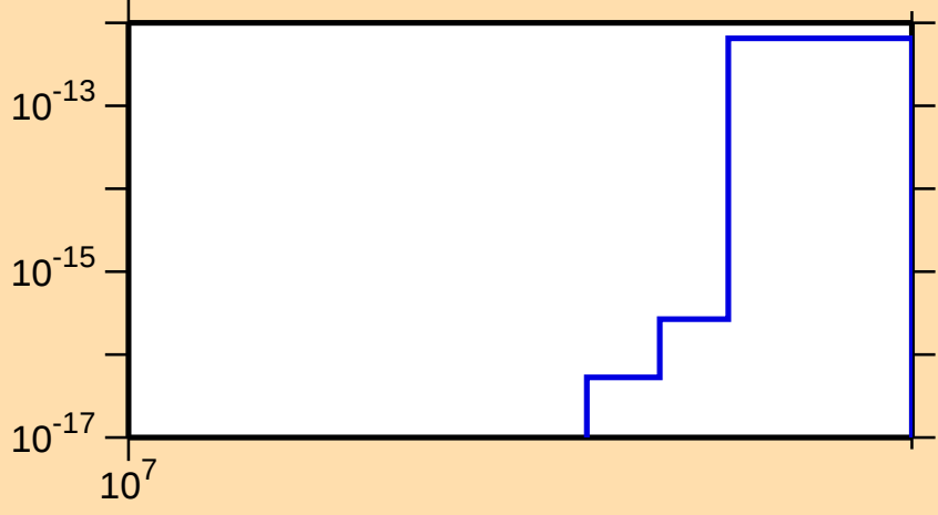
\sigma vs. E for ^{213}\text{Pb} (mt 11)
