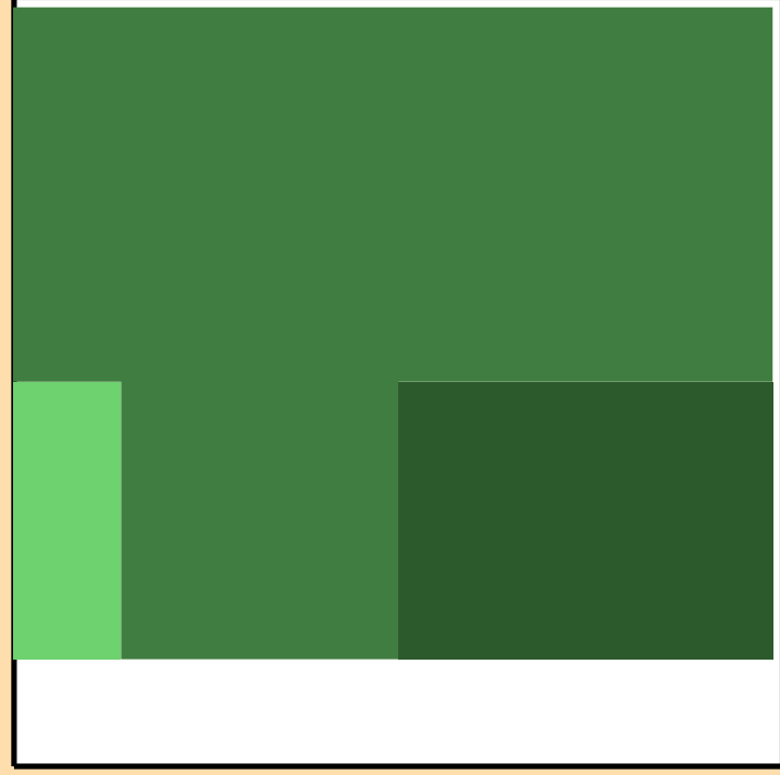
\Delta\sigma/\sigma vs. E for ^{213}\text{Pb}(n,\gamma)
