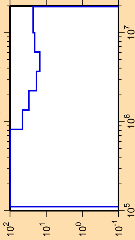
\Delta\sigma/\sigma vs. E for ^{213}\text{Pb}(n,\text{ncont.})
