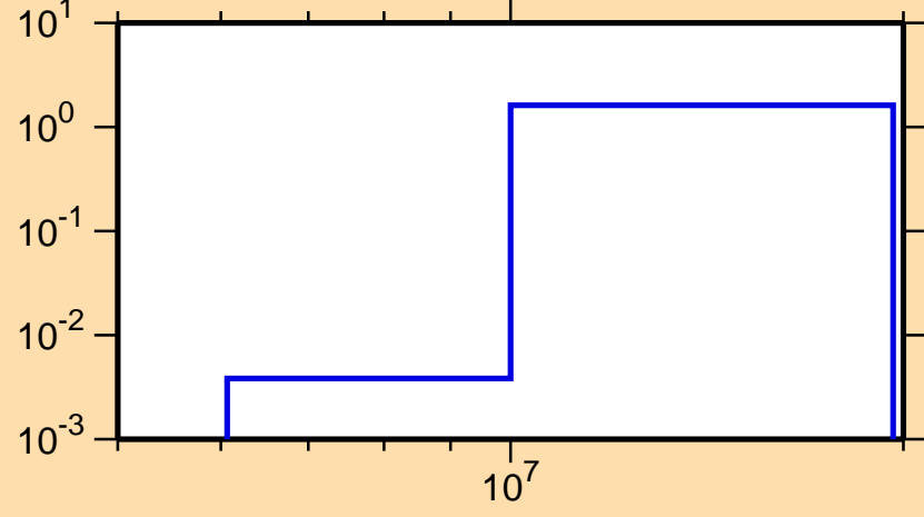
\sigma vs. E for ^{213}\text{Pb}(n,3n)
