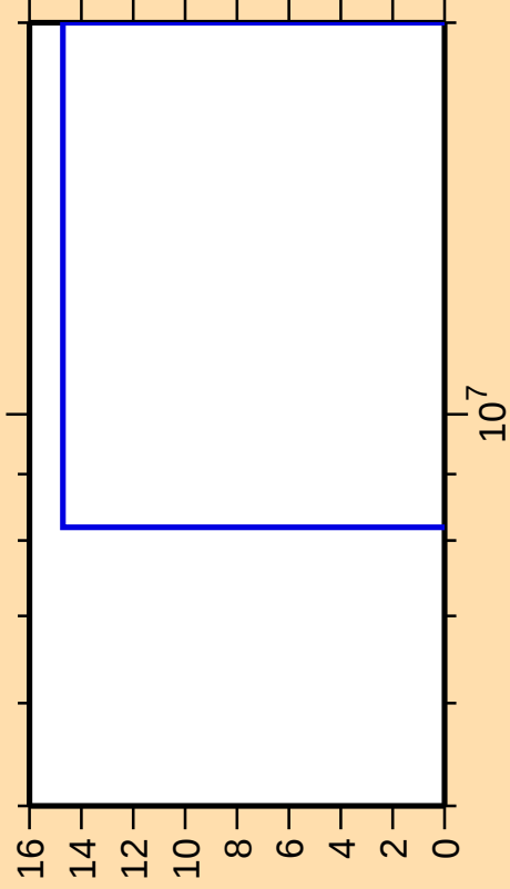
\Delta\sigma/\sigma vs. E for ^{213}\text{Pb}(n,3n)
