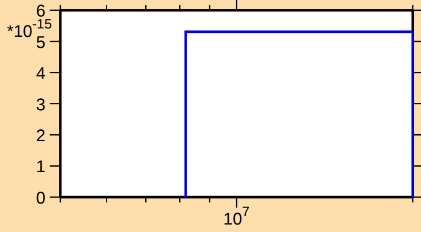
\sigma vs. E for ^{213}\text{Pb}(\text{mt 11})
