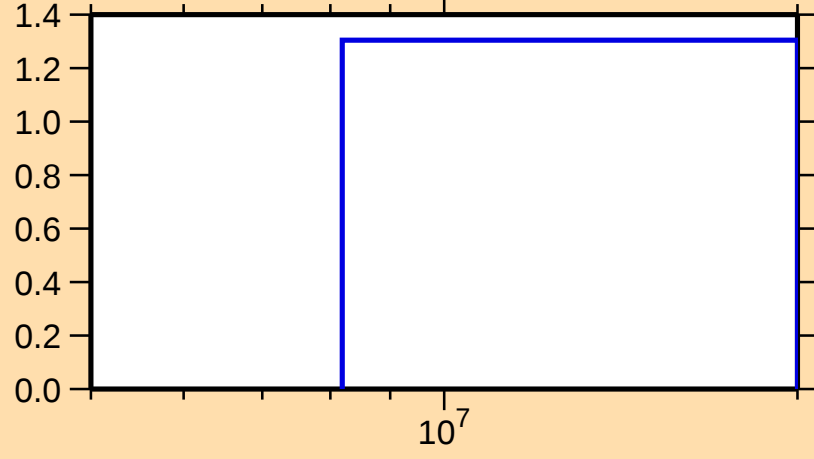
\sigma vs. E for ^{213}\text{Pb}(n,3n)
