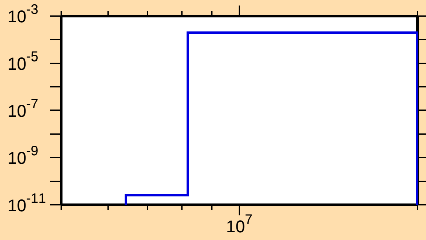
\sigma vs. E for ^{213}\text{Pb}(n,p)
