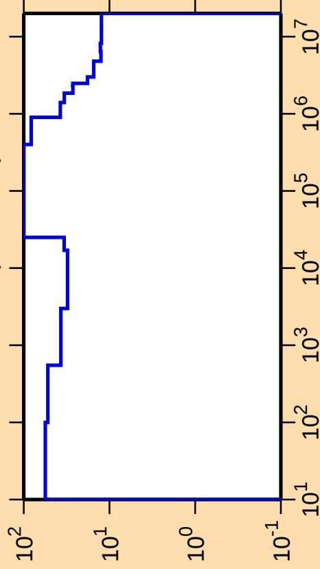
\Delta\sigma/\sigma vs. E for ^{213}\text{Pb}(n,\text{nonel.})
