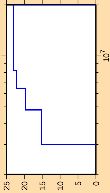
\Delta\sigma/\sigma vs. E for ^{213}\text{Pb}(n,n\text{cont.})
