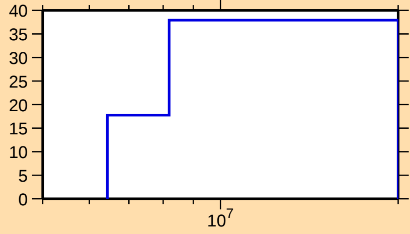
\Delta\sigma/\sigma vs. E for ^{213}\text{Pb}(n,p)
