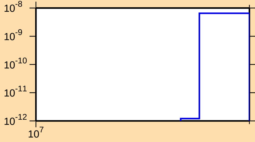
\sigma vs. E for ^{214}\text{Pb}(n,2np)
