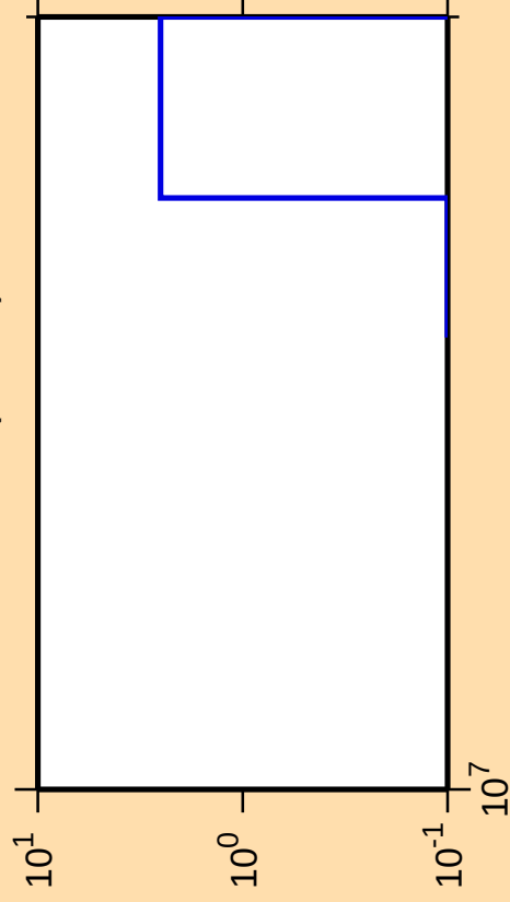
\Delta\sigma/\sigma vs. E for ^{214}\text{Pb} (mt 11)
