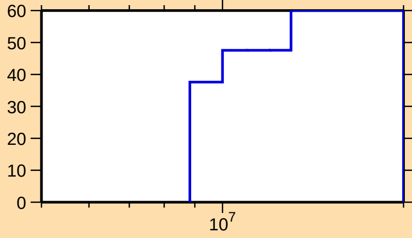
\Delta\sigma/\sigma vs. E for ^{214}\text{Pb}(n,2n)
