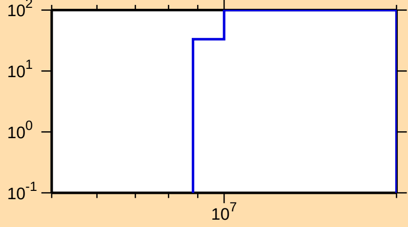
\Delta\sigma/\sigma vs. E for ^{214}\text{Pb}(n,p)
