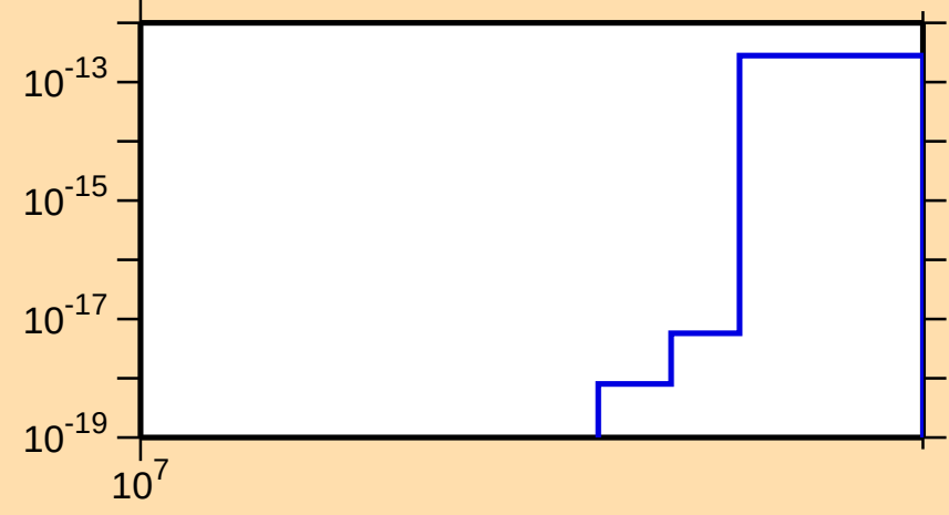
\sigma vs. E for ^{214}\text{Pb} (mt 11)
