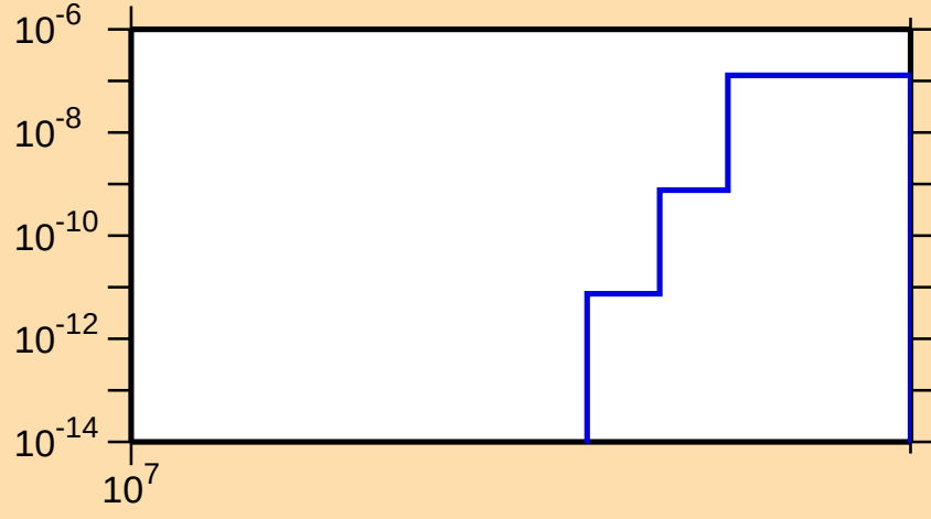
\sigma vs. E for ^{214}\text{Pb}(n,\text{nd})
