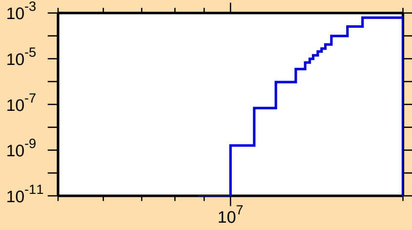
\sigma vs. E for ^{214}\text{Pb}(n,p)
