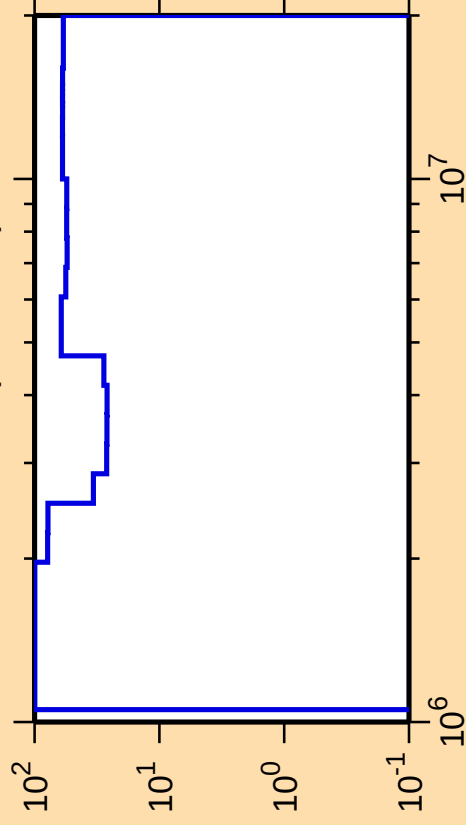
\Delta\sigma/\sigma vs. E for ^{214}\text{Pb}(n,n_{\text{cont}})
