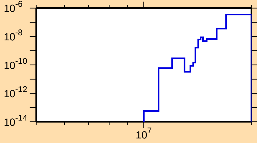
\sigma vs. E for ^{214}\text{Pb}(n,2n\alpha)
